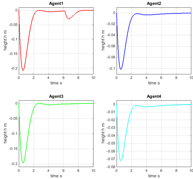
Figure 7.10: Height responses of the linear LQR system controlled by the distributed controller in the presence of link failure between agent 1 and agent 2 followed by an impulse disturbance to agent 1
