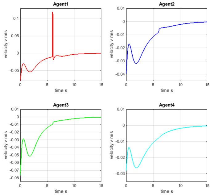
Figure 7.11: Velocity responses of the linear LQR system controlled by the distributed controller in the presence of link failure between agent 1 and agent 2 followed by an impulse disturbance to agent 1
