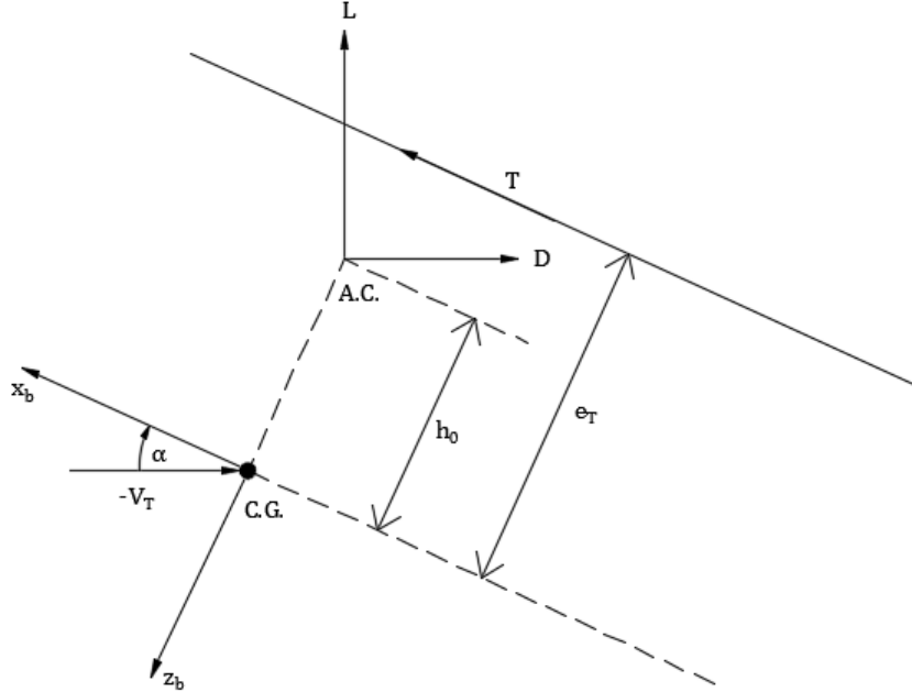
Figure 6.6: Longitudinal aerodynamic forces and moments and thrust representation for X-RAE1
