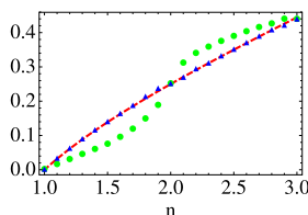
Fig. 2. The dashed line is the function 4\Delta_n = \frac{1}{6} \left( n - \frac{1}{n} \right) . The circles are the values of x_{T\bar{T}} as given by (44) and the triangles are the values of \bar{x}_{T\bar{T}} as given by (63). Clearly the extra poles included in (63) give a very sizable contribution for non-integer values of n .
