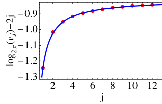
Fig. 4. The dots show the numerical values of \log_{2\pi}(v_j) - 2j evaluated using a Monte Carlo approach. The solid line is the function \log_{2\pi} \frac{v_j^{\text{fit}}}{(2\pi)^{2j}} = -0.806996 - \frac{0.436331}{j} . The fit is extremely good indicating that for j large the \log_{2\pi}(v_j) is linear in j .
