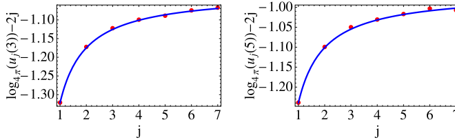
Fig. 3. The dots show the numerical values of \log_{4\pi}(u_j(n)) - 2j for n = 3 and n = 5 and j \leq 7 evaluated using a Monte Carlo approach. The solid lines are fits of the form \alpha + \frac{\beta}{j} .
