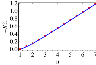
Fig. 5. The dots show the numerical values of -K_{\mathcal{T}\mathcal{T}}^o evaluated using formula (76) with h^o(j, n) for various (non-integer and integer) values of n and summing as many terms as needed to ensure convergence. The solid line is the function -0.34 + \frac{0.13}{n} + 0.215n . The fit is extremely good indicating that the ratio of \mathcal{C}_{\mathcal{T}\mathcal{T}}^2 and \langle \mathcal{T} \rangle_n decays exponentially for n odd. Here, as before, we have set the mass scale m = 1 .
