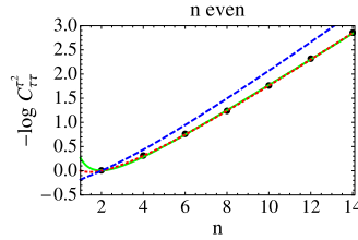
Fig. 6. The logarithm of the structure constant C_{TT}^2 for even values of n (dots). The solid and dotted lines provide two possible fits of the points obtained. The solid (green) curve is the function -\log(C_1(n)) = -1.074 + \frac{1.064}{n} + 0.274n and the dotted (red) curve is the function -\log(C_2(n)) = -0.308 + 0.311n - 0.456 \log n . As we can see both are extremely good for the points we have and yet their curvatures around n = 1 are quite different. The dashed blue line represents an analytical prediction given in [20] (see section 6 for discussions on this comparison). (For interpretation of the references to colour in this figure legend, the reader is referred to the web version of this article.)
