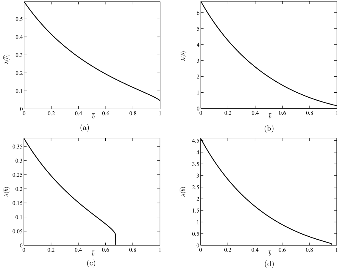
Figure 4. Values of \lambda(\bar{b}) for different vector recruitment rates and minimal contact rates. (a) \Lambda_v = 10^3 \mu_{v_1}, \beta_{\min} = 0.075, p_1 = 1, p_2 = 1 , (b) \Lambda_v = 10^4 \mu_{v_1}, \beta_{\min} = 0.025, p_1 = 1, p_2 = 1 , (c) \Lambda_v = 10^3 \mu_{v_1}, \beta_{\min} = 0.075, p_1 = 0.75, p_2 = 0.75 , (d) \Lambda_v = 10^4 \mu_{v_1}, \beta_{\min} = 0.025, p_1 = 0.75, p_2 = 0.75 . Values of the remaining parameters are \mu_{v_1} = 1/28, \mu_{\max} = \mu_{v_1}, \beta_{\max} = 0.1, \mu_h = 1/(55 \times 365), \Lambda_h = 10^3 \mu_h, \delta_h = 4.1 \times 10^{-4}, \gamma_h = 1/14 .
