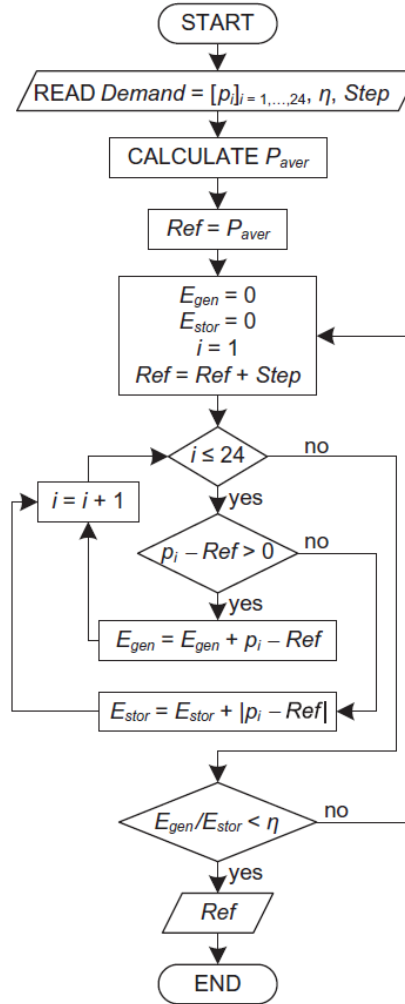
Figure 2.13. Flowchart for calculating set-point reference value for demand smoothening algorithm
