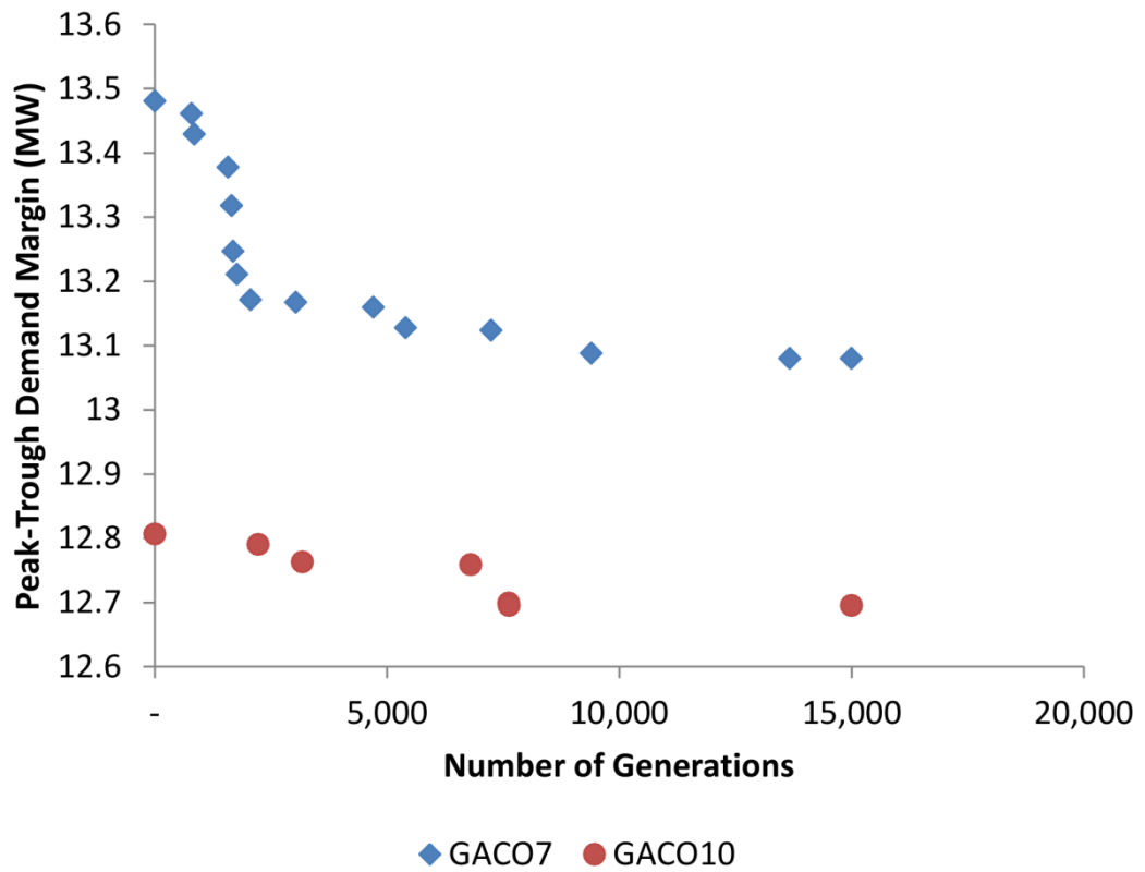
Figure 6.17. Evolution of demand margin showing improvement in load-levelling after application of GACO
