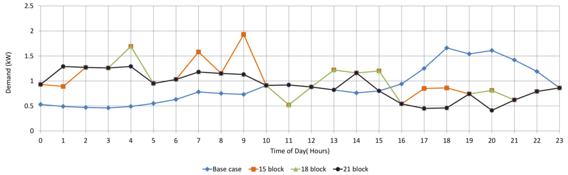
Figure 6.21. Summer Demand using Algorithm to dispatch ESS in different energy block configurations
