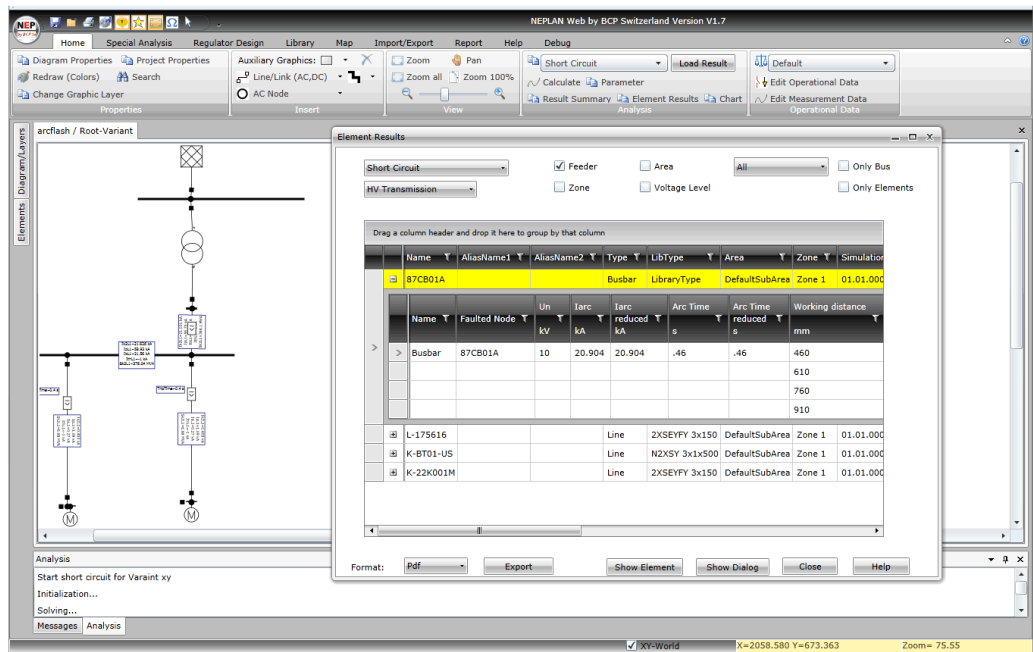
Figure 4.5. NEPLAN 360 Graphical User Interface
