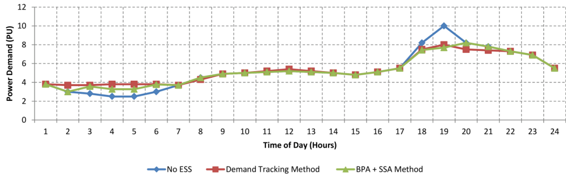
Figure 6.10. Comparative analysis of combinatorial optimisation method and demand tracking set-point
