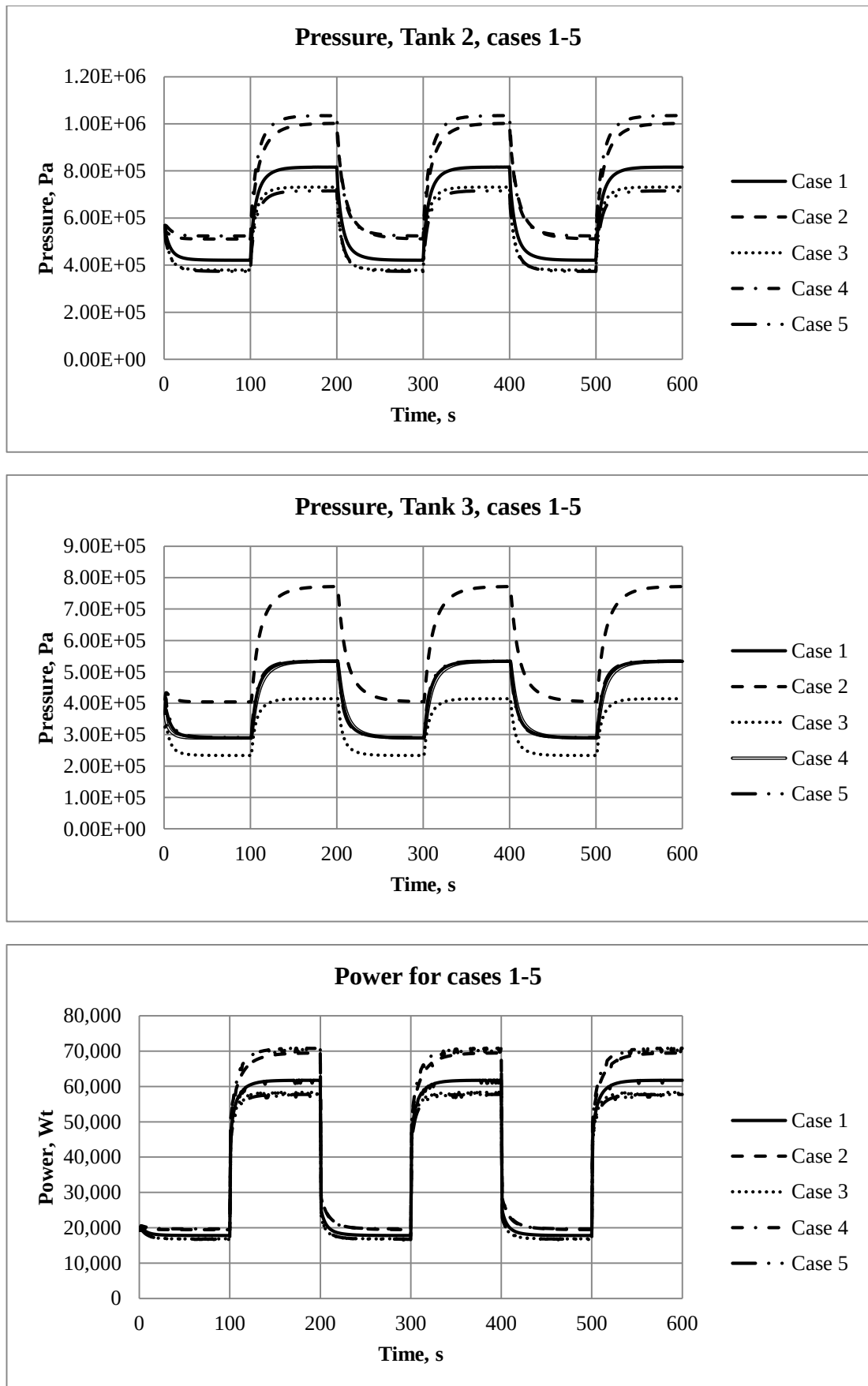
Figure 48: Pressure in Tank2 and Tank3 and input power for cases 1-5
