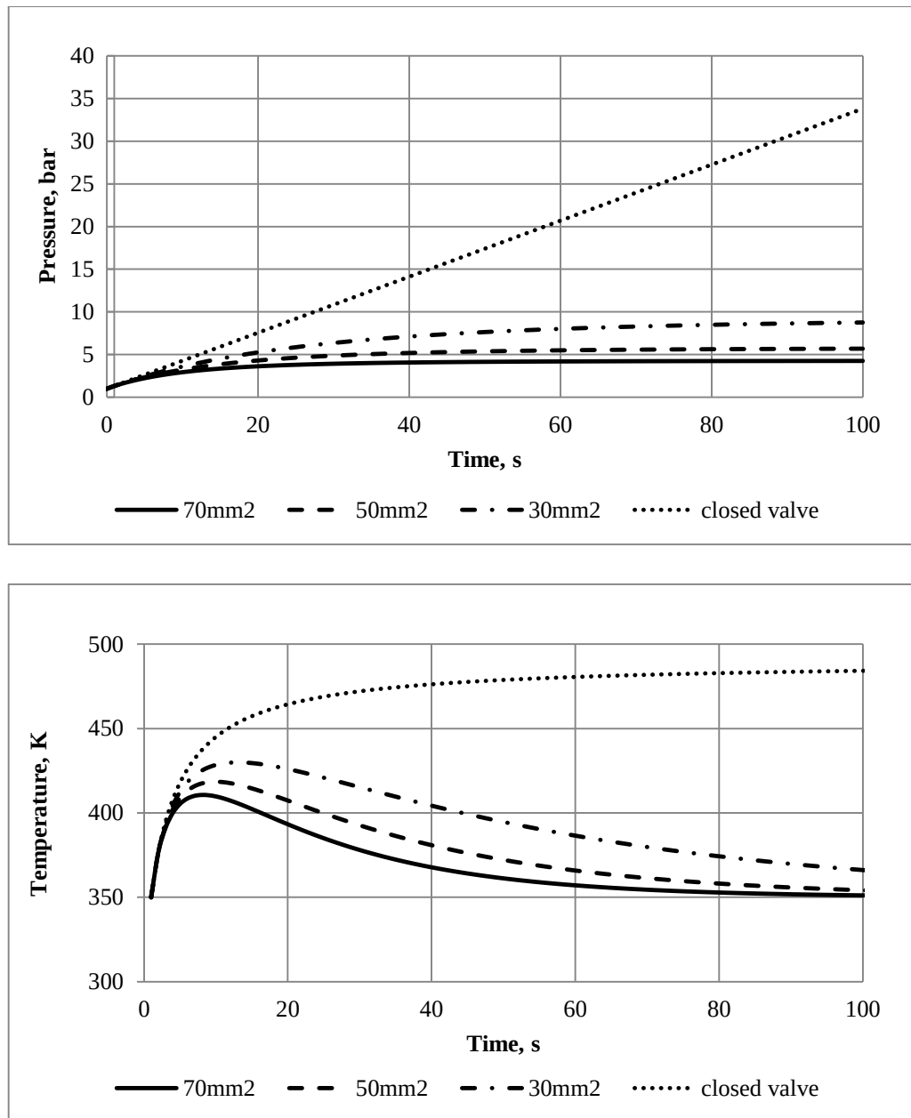
Figure 35: The effect of varying the valve area in an oil-injected air screw compressor plant. The upper graph shows the Tank Pressure, and the lower graph shows the Temperature
