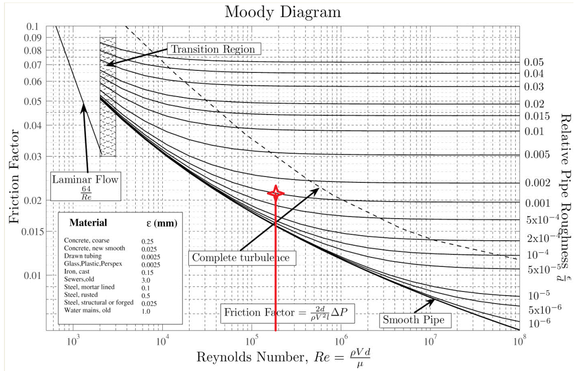
Figure 58: Moody diagram
