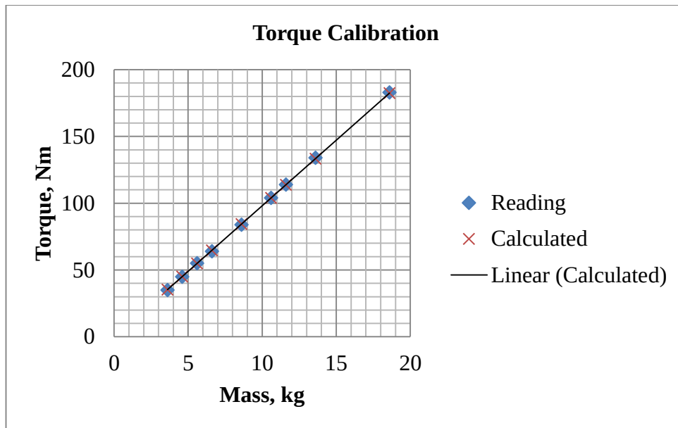
Figure 69: Torque meter calibration results
