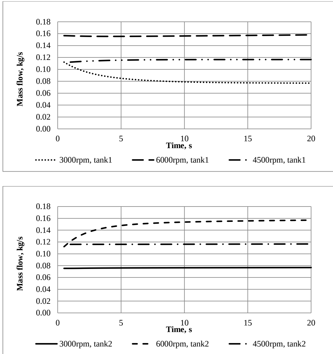
Figure 40: Mass flow going to both tanks at different shaft speeds
