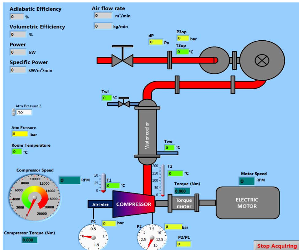
Figure 6: Schematic view of oil-free compressor test rig – Computer screen
