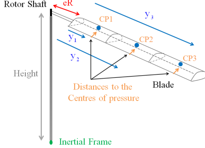
Figure 4: Blade and centre of pressure geometry, showing the spatial configuration in connection with inertial frame.
