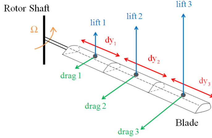
Figure 6: Lift and drag forces representation for the corresponding points on the main rotor.
