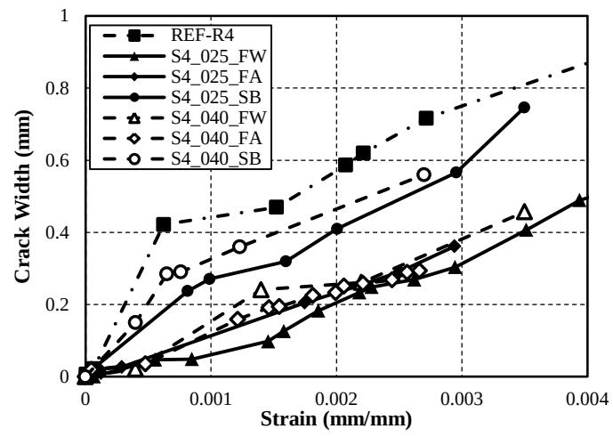
Fig. 10. Crack width details
