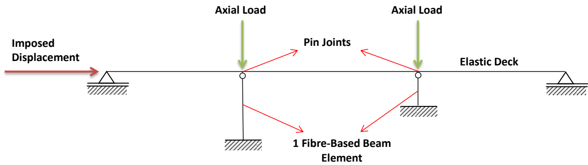
Fig. 7: Modelling using 2D frame elements for bridge with Bearing type Connection
