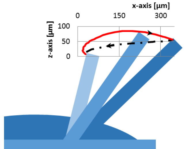
Fig. 4: Schematic view of the flap movement with the measured path of a flap's tip. The upper path represents the fast power stroke whereas the lower path corresponds to the slow recovery stroke. In the upper path high-pressure whereas in the lower path low-pressure is applied. The data were obtained from measuring the flap deflection optically
