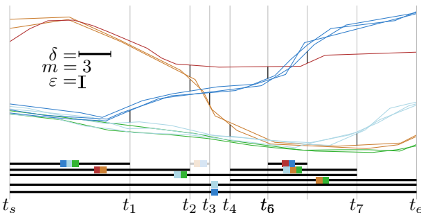
Fig. 3. A set of trajectories and maximal groups as defined by Buchin et al. [5]. The two sets of blue entities also form a group on [t_s, t_1] , however this group is not maximal, as all blue entities together with the green entities also form a group on [t_s, t_1] . The orange and blue entities do not form a group on [t_2, t_3] as their time interval is too short.
