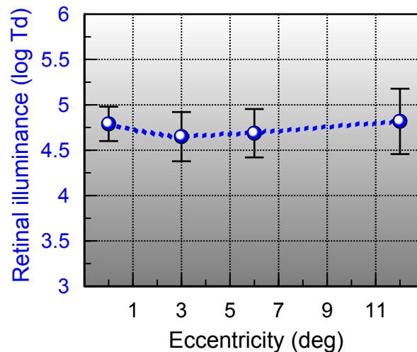
Figure 3-8 Mean discomfort glare thresholds from a sample of 12 participants were shown for a range of different eccentricities. The source size was 1.33° in diameter. The error bars represent \pm 2 SE. Measurements taken at the fovea and three peripheral (3°, 6° and 12°) locations show no change in thresholds with eccentricity.
