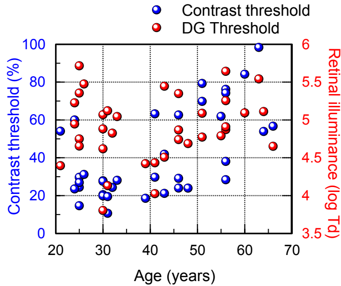
Figure 5-13 Comparison between functional contrast threshold and discomfort glare threshold for a sample of 36 participants. The Landolt C stimulus in the CAA test was presented in the fovea with the background luminance of 2.6 cd/m 2 . The disability glare placed at 10° to the right of the centre was set to 19.21 lx.
