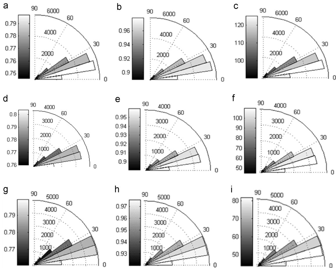
Fig. 8. Distribution of angle \alpha for the specimens: (a) Int3 shaded by EI ; (b) Int3 shaded by S (c) Int3 shaded by CA ; (d) Int3S shaded by EI ; (e) Int3S shaded by S (f) Int3S shaded by CA ; (g) Rec3 shaded by EI ; (h) Rec3 shaded by S (i) Rec3 shaded by CA .
