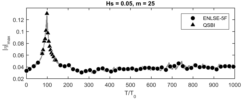
Fig. 18. Maximum wave elevations with indicator which model is used for the cases of different numbers of rogue waves in spatial domain
