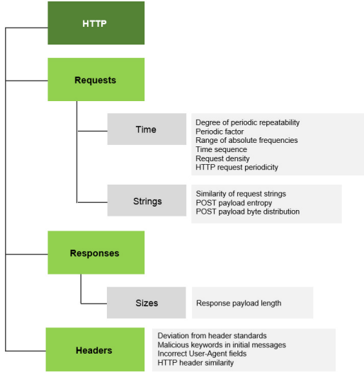
Figure 4. HTTP-based features, from (Etemad & Vahdani, 2012), (Eslahi et al., 2013), (Eslahi et al., 2015), (Cai & Zou, 2012), (Al-Bataineh Figure 5. DNS-based features, from (Schivoni et al., 2014) & (Sharifnya & Abadi, 2013).
