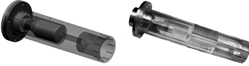
Figure 6. Nozzle design to induce cavitation: CAD model (left), manufactured nozzle (right).
