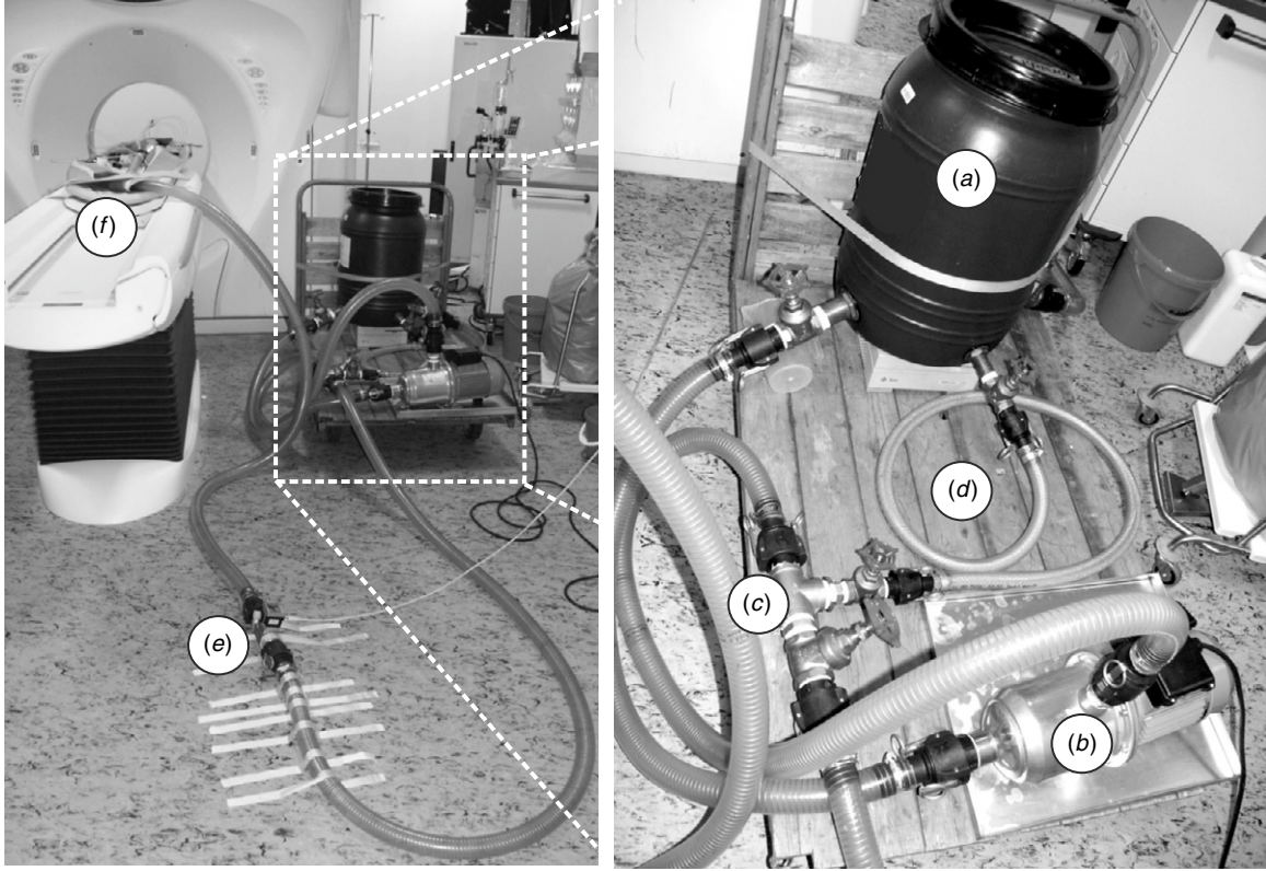
Figure 8. Mobile test rig: (a) tank, (b) pump, (c) tee branch with two valves, (d) bypass, (e) main pipe with flow meter, (f) nozzle.
