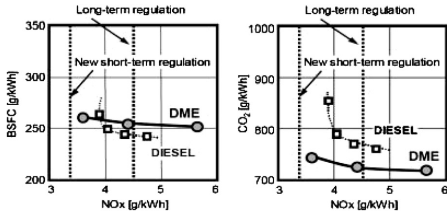
Fig. 3. Fuel consumption (BSFC), \text{NO}_x and \text{CO}_2 emissions for DME compared to diesel from a six-cylinder 71 turbocharged/intercooled heavy-duty diesel engine operating in Japanese D13 mode [18].
