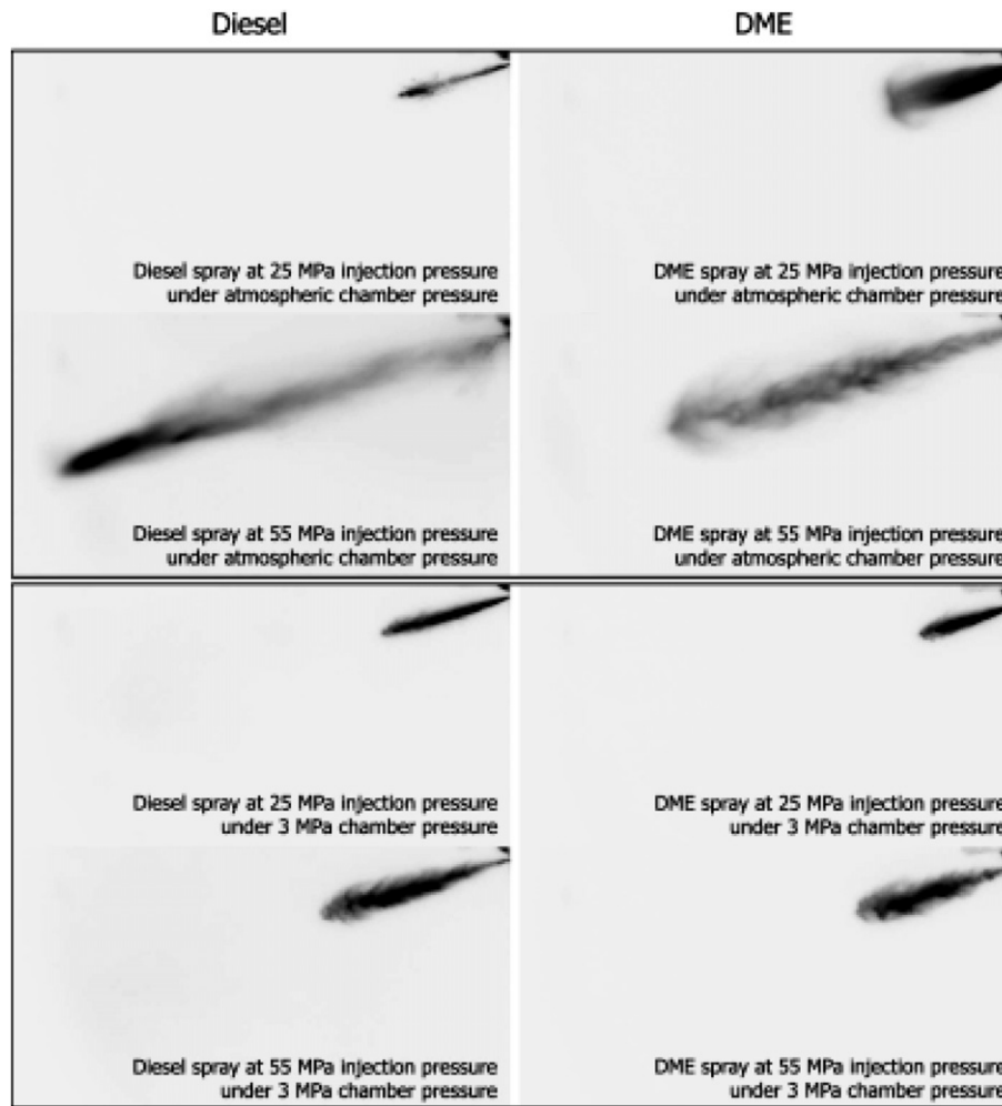
Fig. 2. DME sprays at various conditions compared to diesel sprays [18]; atmospheric (10.1 MPa) and high pressure (3 MPa) ambient conditions with fuel-injection pressures at 25 and 55 MPa.
