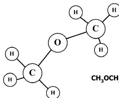
Fig. 1. Structure of di-methyl ether (DME).
