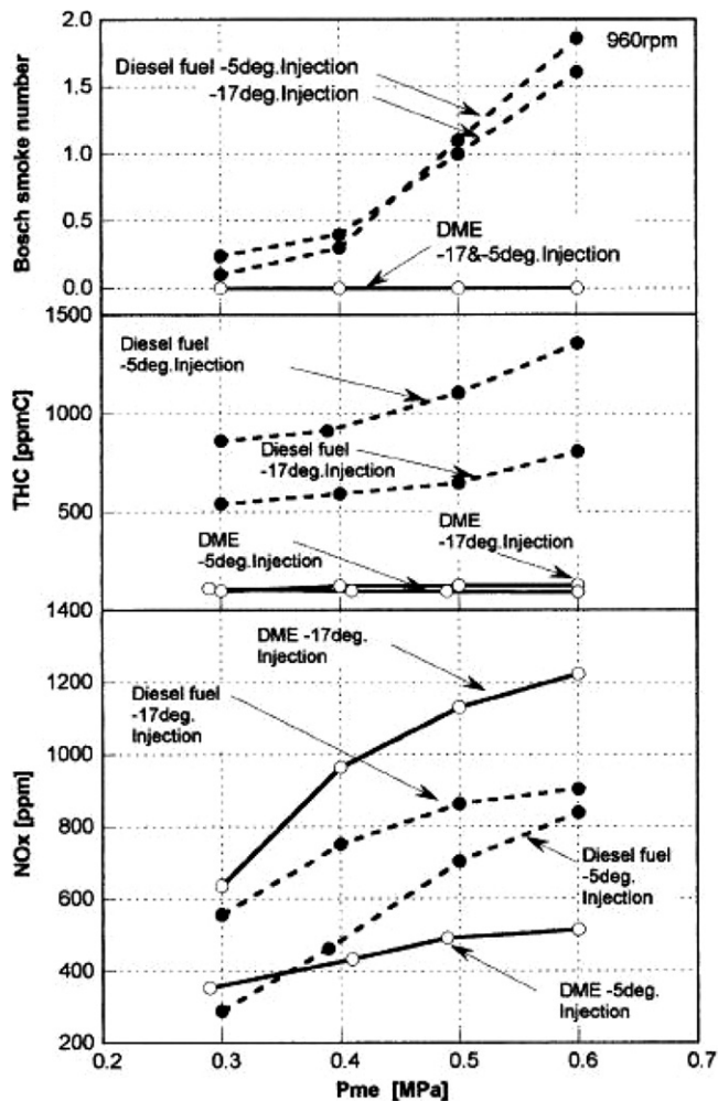
Fig. 4. Smoke, THC and \text{NO}_x emission for DME and diesel from a single cylinder of 638 \text{ cm}^3 DI compression-ignition engine [33].
