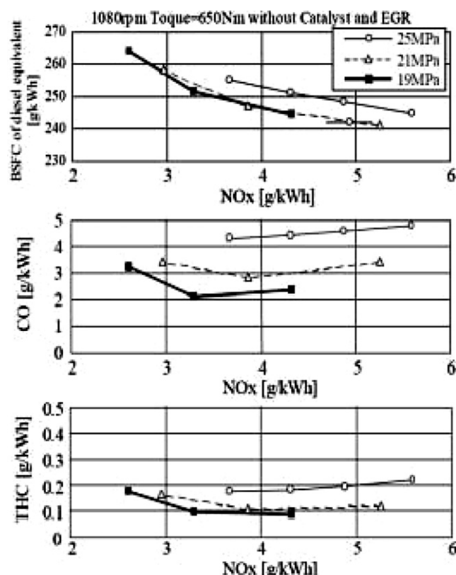
Fig. 5. Effect of fuel-injection pressure in the low speed and high load operating conditions for DME with a single cylinder of 638 ml DI compression-ignition engine [18].
