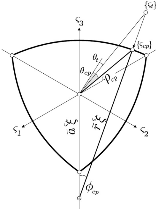
Fig. 6. Modified Reuleaux closest point in a deviatoric plane.
