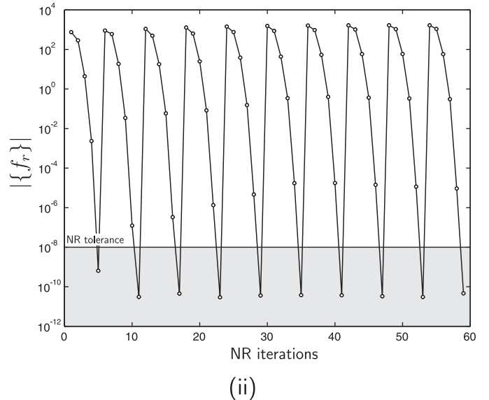
Fig. 20. Single 3D finite element analysis results (i) force-displacement plots for different forms of the model, with and without LAD (ii) convergence for the W-W LAD ( \alpha = \gamma = 0.5 ).
