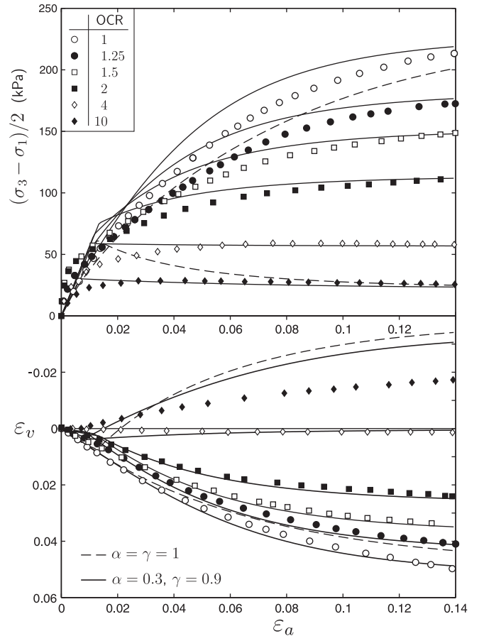
Fig. 14. Drained triaxial compression test simulations compared with experimental data (shown by discrete points) [20]. Above: axial strain ( \epsilon_a ) against deviatoric stress ( (\sigma_3 - \sigma_1)/2 ). Below: axial strain ( \epsilon_a ) against volumetric strain ( \epsilon_v ).
