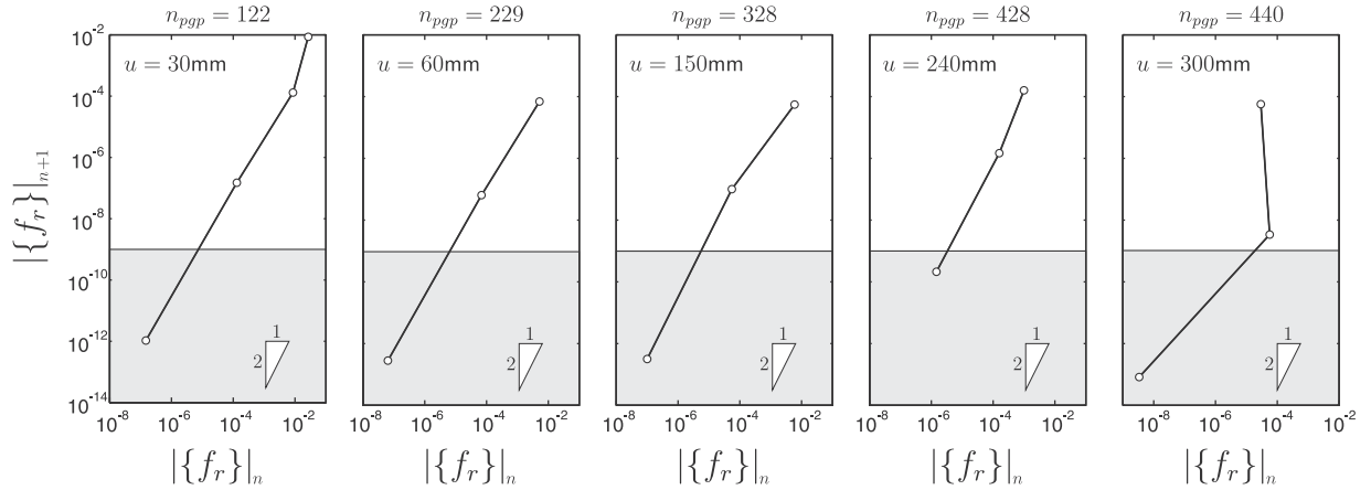
Fig. 24. Rigid strip footing convergence showing the norm of the residual out-of-balance force against the previous out-of-balance force for loadsteps 10, 20, 50, 80 and 100.
