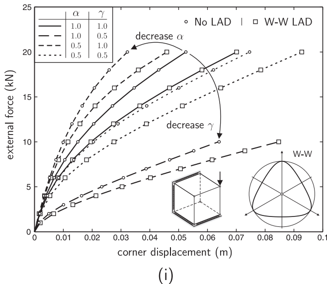
Fig. 20. Single 3D finite element analysis results (i) force-displacement plots for different forms of the model, with and without LAD (ii) convergence for the W-W LAD ( \alpha = \gamma = 0.5 ).
