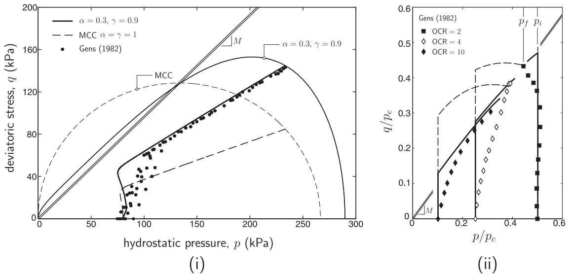
Fig. 8. Test simulations using the MCC model ( \alpha = \gamma = 1 ) and the two-parameter model ( \alpha = 0.3 , \gamma = 0.9 ) compared against experimental data (shown by discrete points) from Gens [20]: (i) one-dimensional consolidation (ii) undrained triaxial compression with OCR = 2, 4 and 10 (the dashed line indicates the MCC model response, whereas the continuous line shows the stress path obtained from the two-parameter hyperplastic model).
