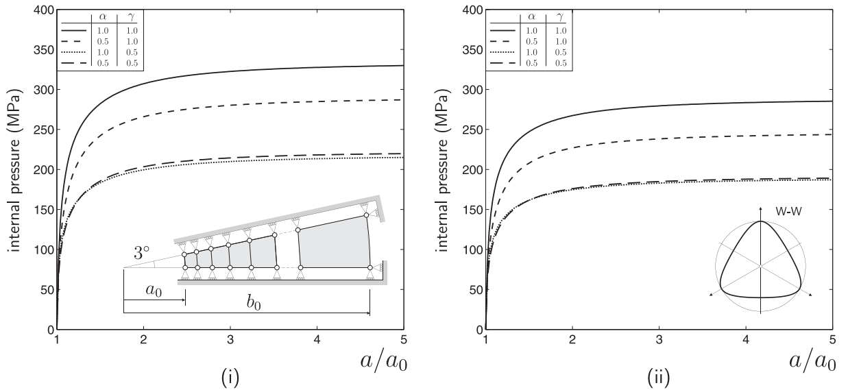
Fig. 25. Finite deformation expansion of a cylindrical cavity (i) no LAD (ii) W-W LAD with \bar{p}_e = 0.7695 .
