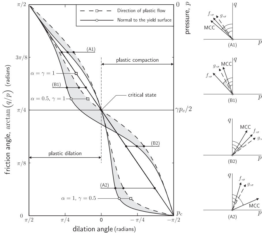
Fig. 10. Dilation angle for the plastic flow direction and the normal to the yield surface for \alpha = \gamma = 1 , \alpha = 0.5, \gamma = 1 (B1–2) and \alpha = 1, \gamma = 0.5 (A1–2). The width of the shaded region indicates the degree of non-associatedness of the flow.
