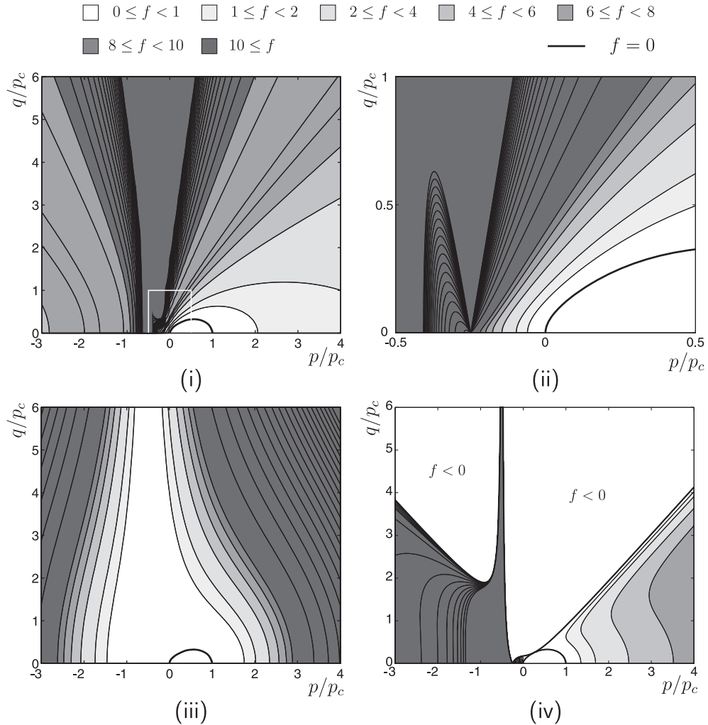
Fig. 18. Contours of the yield function outside of the yield surface for a two-parameter Critical State model where \alpha = \gamma = 0.5 (i) f given by (71) from [7,11,8,9], (ii) local detail of f given by (71), (iii) f given by (36) 1 , and (iv) f from (73) with negative regions appearing outside the yield surface.
