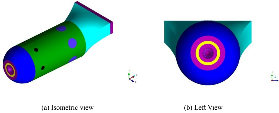
Fig. 3 Configuration of model can type combustor
