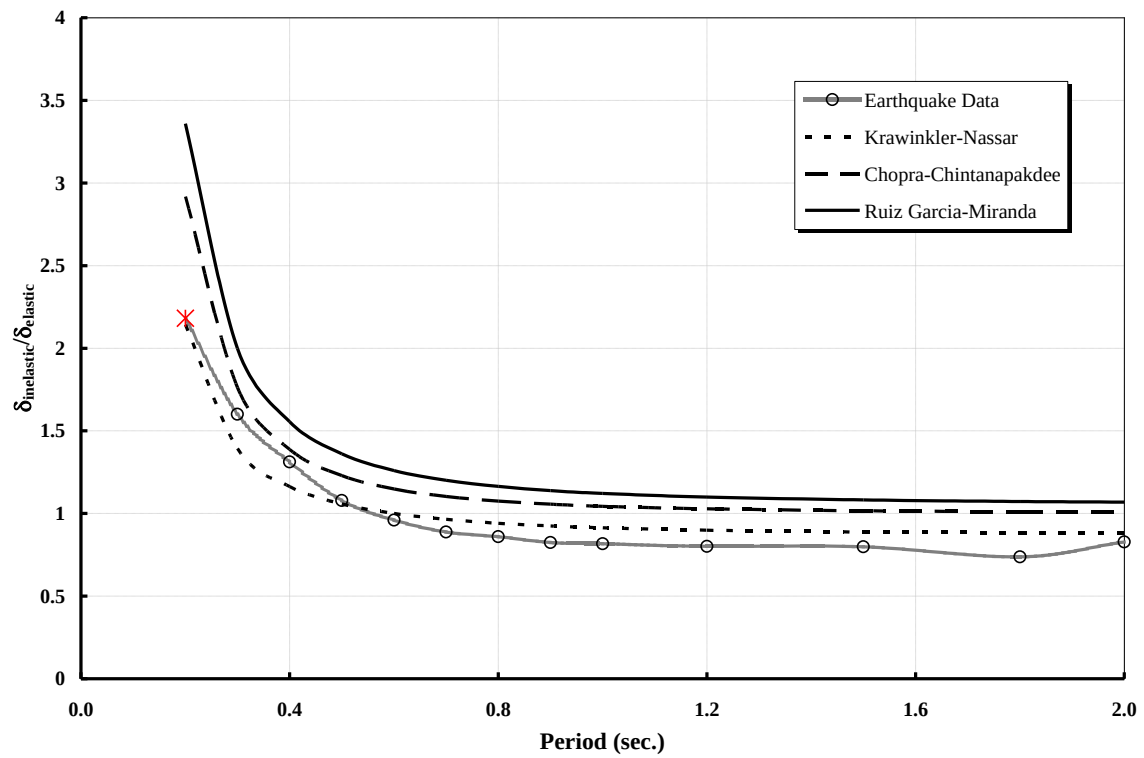
Fig. 20 Inelastic Displacement Ratio, Modified Clough Model-R=4,Low Degradation
