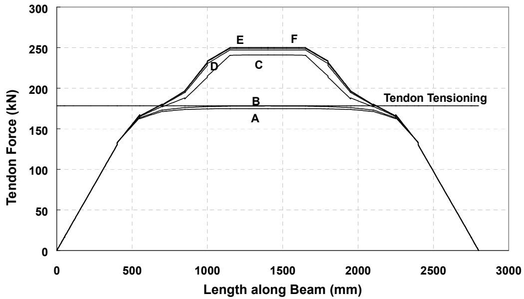
FIGURE 16 TENDON FORCE DISTRIBUTION FOR BEAM 16/65-1150
