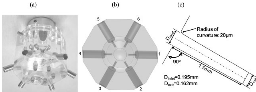
Fig. 3 (a) Photograph of the \times 15 enlarged fully transparent nozzle replica used for visualization of cavitation inside the injection holes, (b) bottom view of the transparent nozzle indicating the injection holes numbering and expansion tubes, and (c) tapered nozzle hole geometric characteristics
