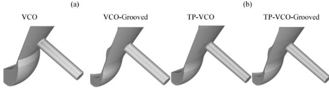
Fig. 2 Numerical grid of the 60° sector of the VCO nozzle designs investigated: (a) cylindrical hole nozzle and (b) tapered hole nozzle. For each nozzle, two different needle shapes have been tested, one with a flat needle as shown and one incorporating a recovery groove
