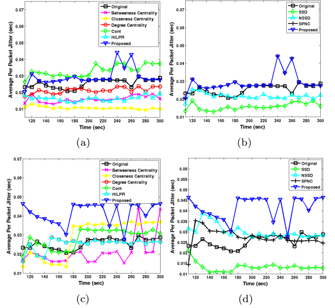
Figure 8: Time evolution of the per packet jitter for the original network, and when a) & b) A single node, c) & d) 10% of the most critical nodes are removed according to betweenness centrality, closeness centrality, degree centrality, Hybrid Interactive Linear Programming Rounding (HILPR), the Controllability of complex networks (Cont), the Sum Squared Difference (SSD) approach, the Normalized Sum Squared Difference (NSSD) approach and the Spectral Partitioning for Node Criticality (SPNC) approach.
