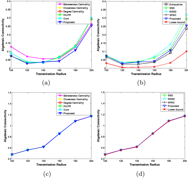
Figure 3: Algebraic Connectivity versus the transmission radius when: a) & b) a single node is removed from the network, c) & d) five nodes are removed from the network.
