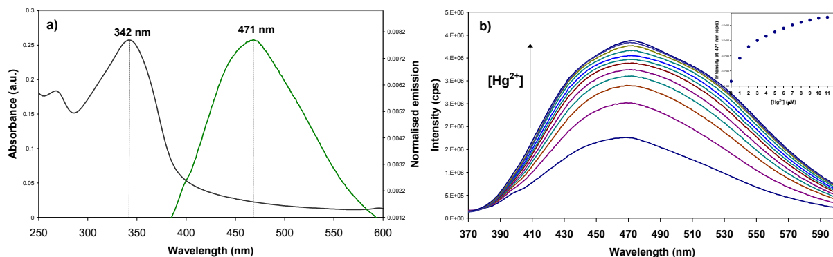
Figure 2. a) Absorption and emission spectra of CACE (10 \mu\text{M} ) in \text{H}_2\text{O}/\text{MeCN} (7:3, v/v). Emission spectrum recorded with \lambda_{\text{ex}} = 350 nm. b) Emission spectra of CACE at [\text{Hg}^{2+}] ranging from 0 to 11 \mu\text{M} . The inset shows the titration plots at 471 nm ( \lambda_{\text{ex}} = 350 nm).
