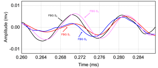
Fig. 8. Acoustic signals acquired by the optical based acoustic sensors at all four sensor locations of the half-rudder when rudder was subject to excitation of the sonotrode.
