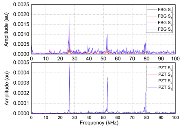
Fig. 9. Frequency response of FBG-based acoustic sensors and PZT acoustic sensors indicating a close match of standard sonotrode frequency of 26 kHz.
