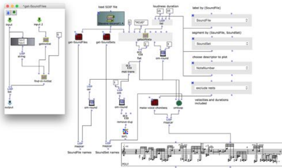
Figure 11. Patch for Without Words with sub-patch get-SoundFiles on the left.
