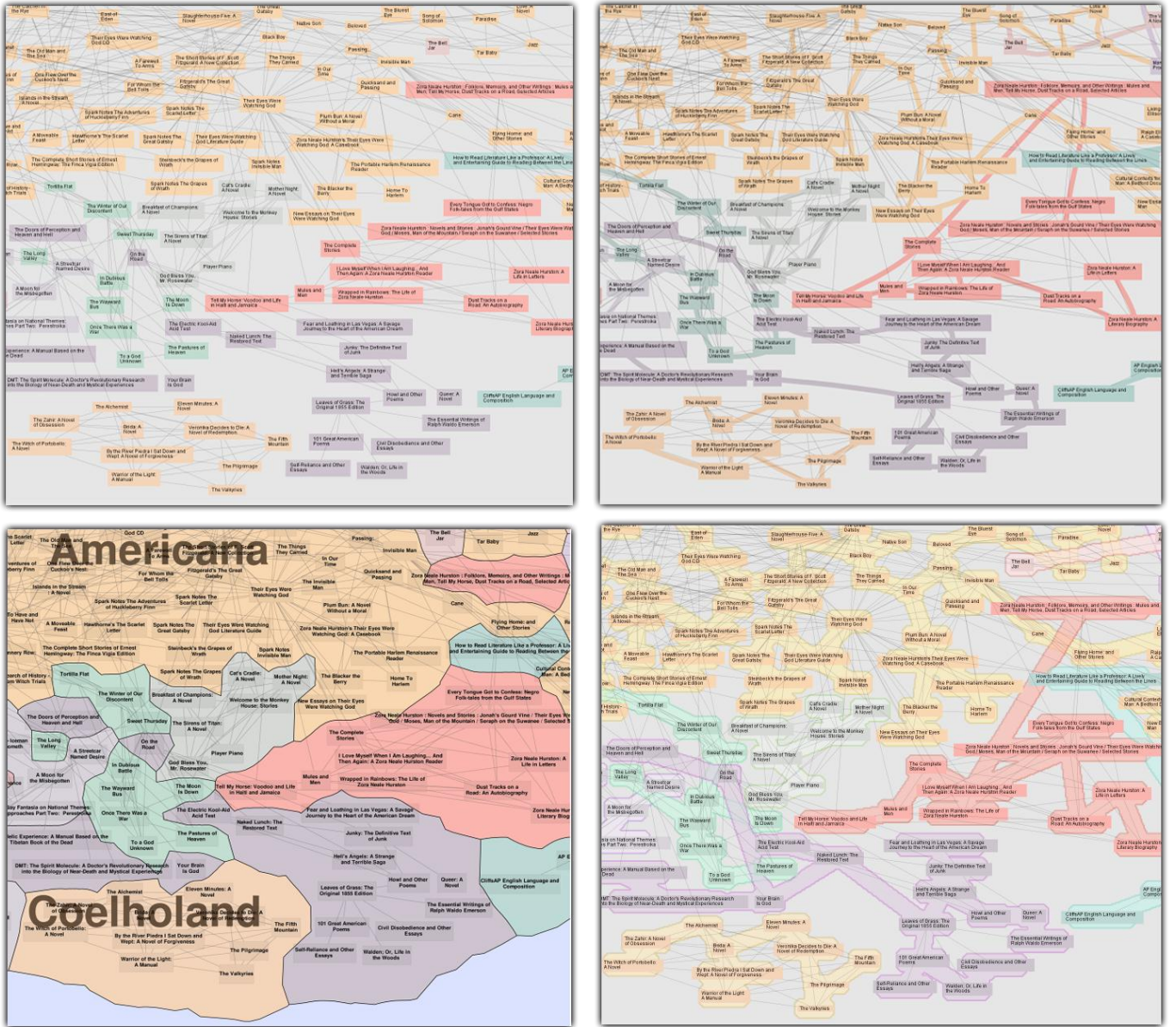
Fig. 1: Four visualizations for viewing group information over node-link diagrams: colored node-link diagram (top left), LineSets (top right), GMap (bottom left), and BubbleSets (bottom right).
