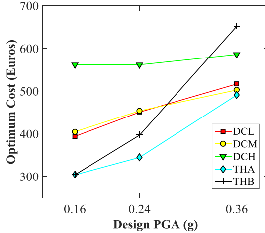
Figure 5: Optimum costs obtained by different design methodologies and design PGAs for the 10/50 seismic hazard level.
