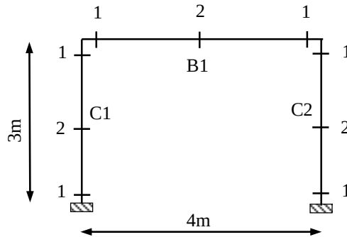
Figure 3: Example portal frame
