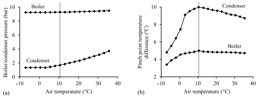
Figure 8. (a) Boiler and condenser pressure; (b) Pinch point temperature differences required for maximum net power output at off-design conditions using WORC optimised for 10.5 °C air temperature.
