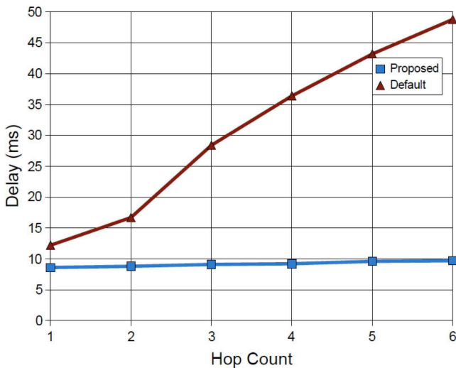
Fig. 12: Average queueing delay in a chain topology.
