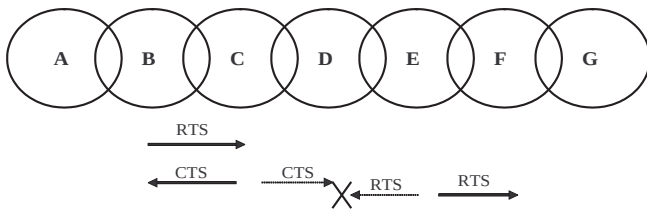
Fig. 3: 802.11 control packets collisions.
