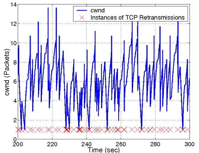
Fig. 4: Illustration of TCP congestion window change in a 6 hop chain topology.
