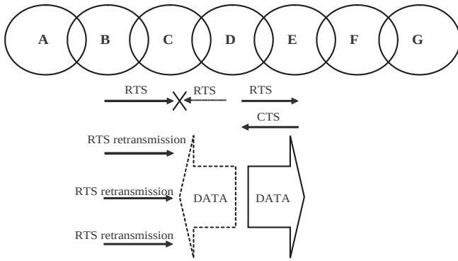
Fig. 2: RTS &amp; TCP DATA collision.
