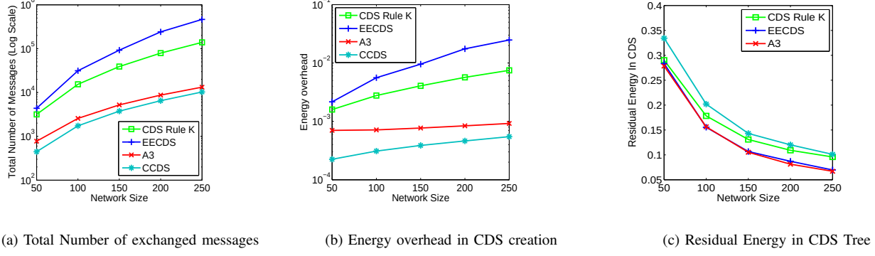
Fig. 7. CCDS analysis under varying network sizes.
