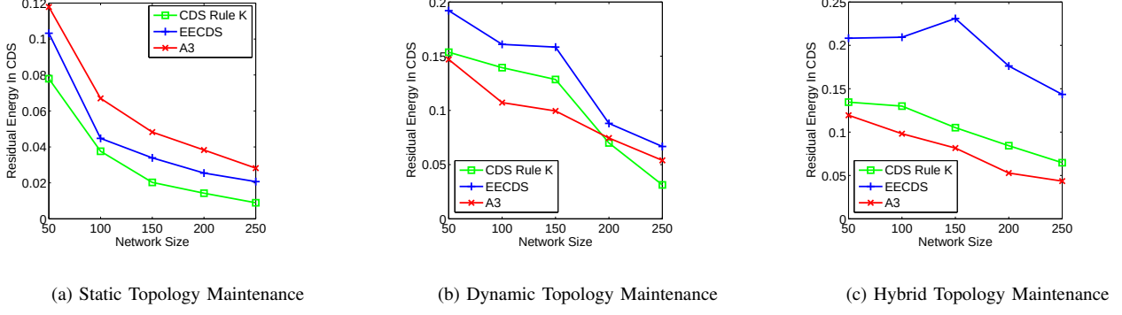
Fig. 3. Residual energy under varying network sizes.
