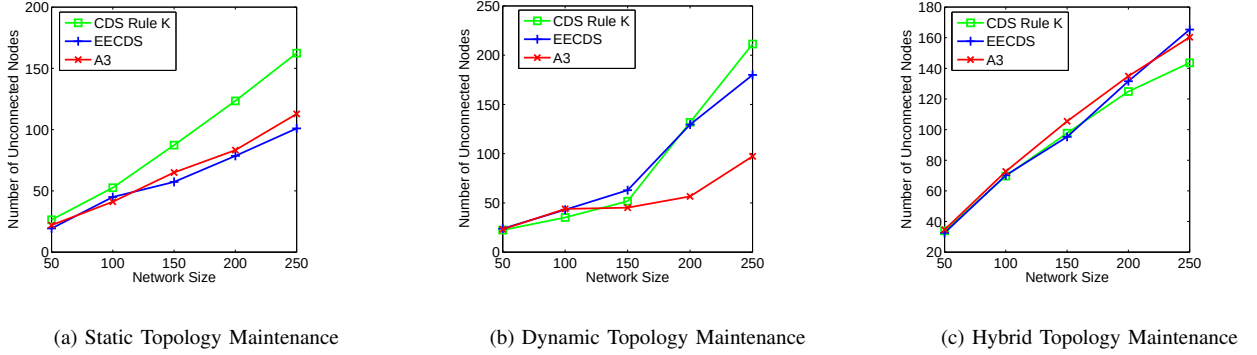
Fig. 4. Number of unconnected nodes under varying network sizes.
