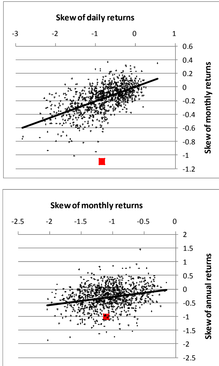
Figure 2:Skewness of index returns at different intervals
