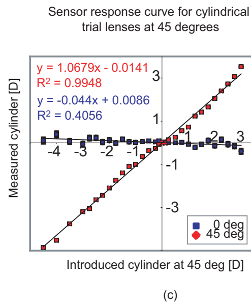
Figure 3. The sensor response curve for trial lenses. (a) Spherical lenses, (b) Cylindrical lenses oriented at approximately 0^\circ (b) Cylindrical lenses oriented at approximately 45^\circ .
