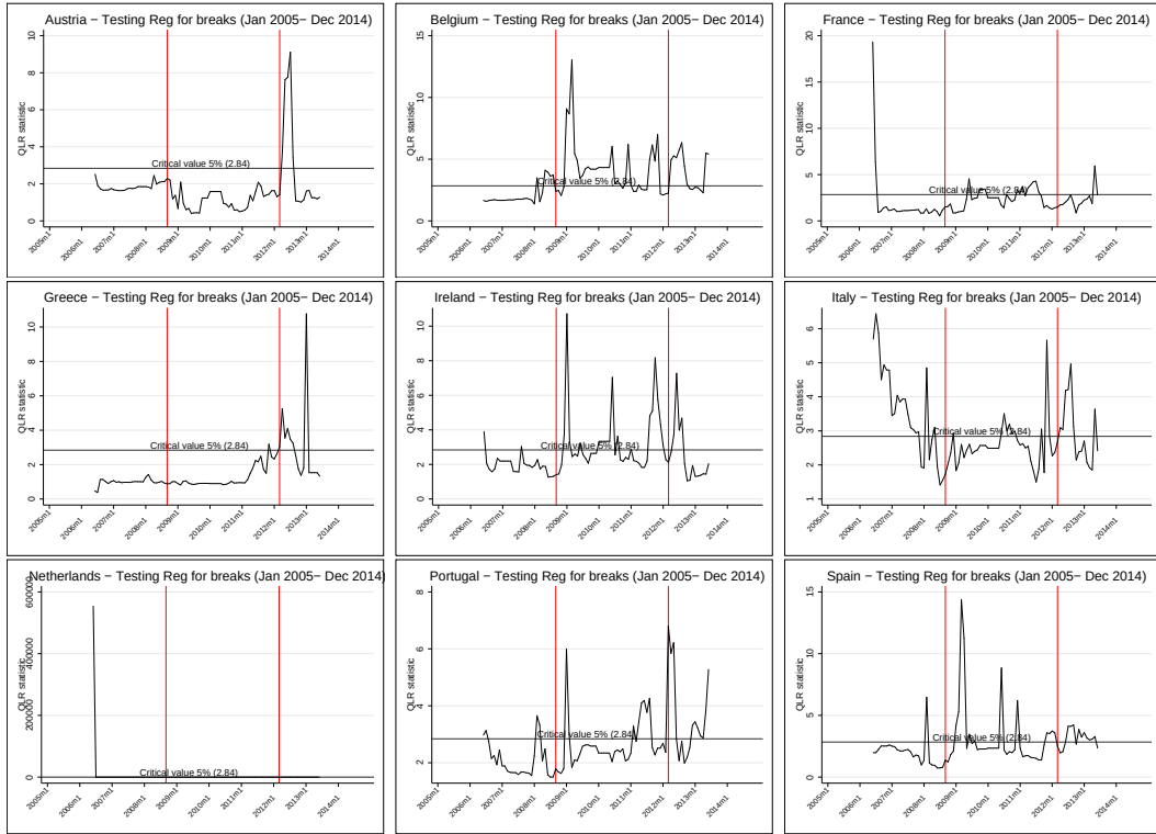
Figure 4.3: Quandt Likelihood Ratio (QLR) Structural Break in Regression
