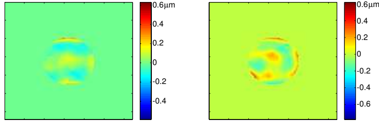
Fig. 1. Films showing the evolution of the wavefront transmitted through the tear film at 22Hz for subjects 2 (left, 2MB) and 7 (right, 1MB.)
