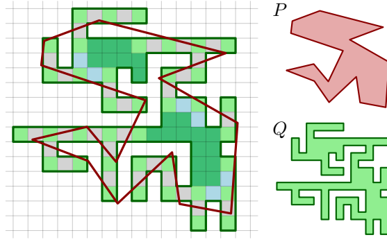
■ Figure 4 Example of the Hausdorff algorithm; the input and output are shown on the right. Colors: ■ Q_1 , ■ Q_2 , ■ Q_3 , ■ Q_4 .
