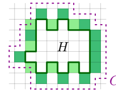
■ Figure 5 A hole in Q . Colors: ■ Q_1 \cap B ; ■ Q_2 \cap B .
