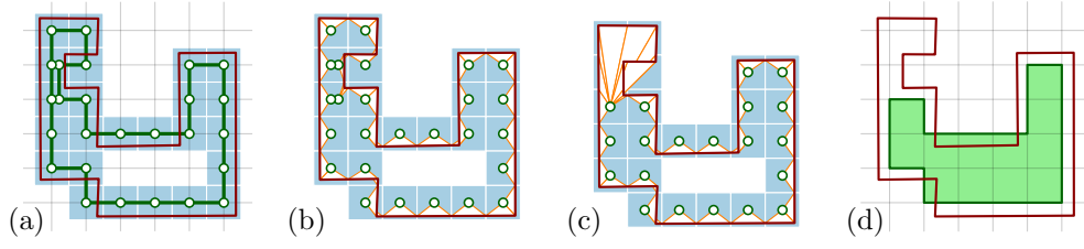
■ Figure 8 Constructing Q for the upper bound on the Fréchet distance. (a) Input polygon on the grid and the squares it visits (shaded); initial state of C with revisited vertices slightly offset for legibility. (b) Initial mapping \mu (white triangles) between the vertices of C and \partial P . (c) Removal of duplicate vertices in C , and its effect on \mu . (d) Resulting cycle represents a grid polygon.
