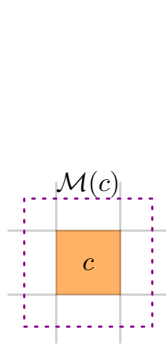
■ Figure 3 Module \mathcal{M}(c) (dashed) of a cell c .
