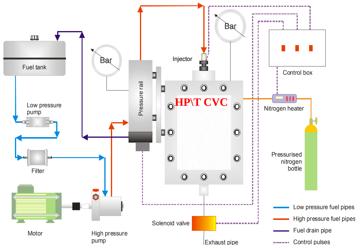
Figure 2 Schematic of the high-pressure\temperature constant volume chamber (HP\T CVC) test rig and the high pressure injection system.
