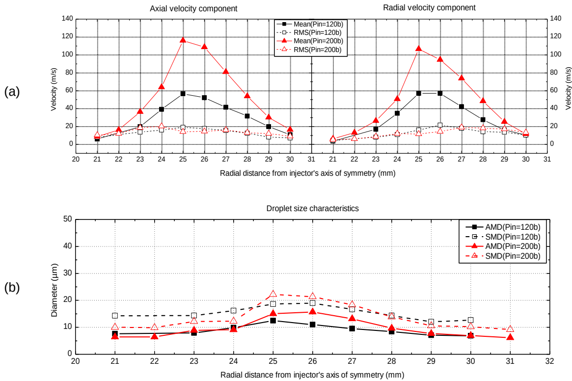
Fig. 22 Spatial variation of (a) droplet velocity and (b) droplet diameter at injection pressures of 120 and 200\text{bar} , chamber pressure of 1\text{bar} and axial location 30\text{mm} from nozzle exit.
