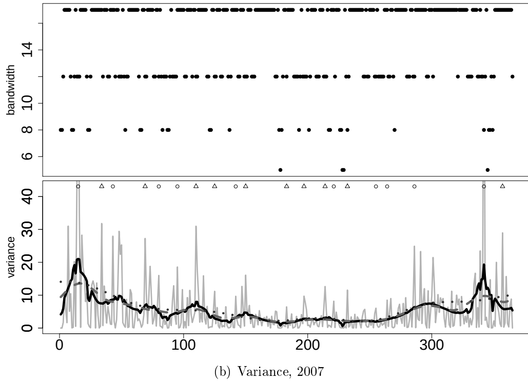
Figure 7: Estimation of mean and variance for New York. In both figure sequence of bandwidths (upper panel), averaged observations (solid grey line), nonparametric function estimation with fixed bandwidth (dashed grey line), adaptive bandwidth (solid black line) and truncated Fourier (dotted line) (bottom panel of each figure). Circles and triangles in each bottom panel for variance represents the 10 smallest and the 10 largest outliers respectively.
