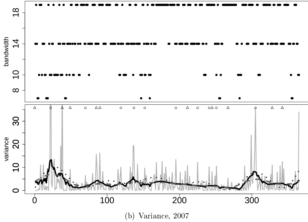
Figure 5: Estimation of mean and variance for Berlin. In both figure sequence of bandwidths (upper panel), averaged observations (solid grey line), nonparametric function estimation with fixed bandwidth (dashed grey line), adaptive bandwidth (solid black line) and truncated Fourier (dotted line) (bottom panel of each figure). Circles and triangles in each bottom panel for variance represents the 10 smallest and the 10 largest outliers respectively.
