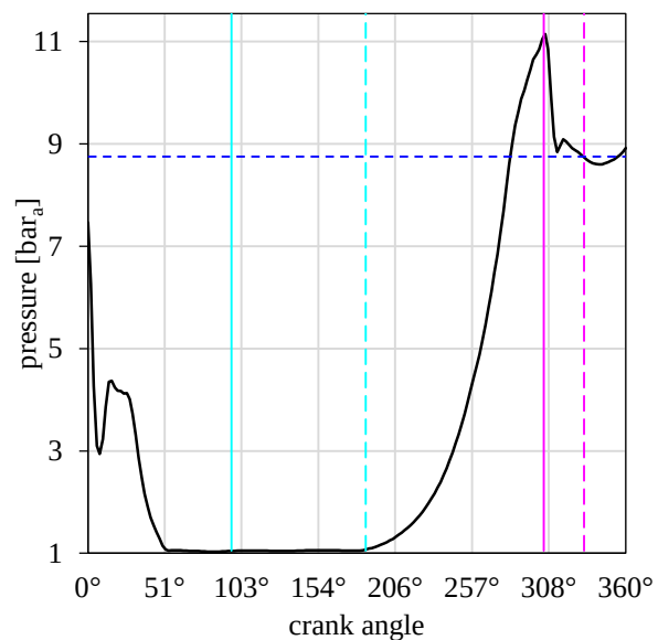
Figure 10: Vane pressure evolution with angular references of ports and outlet pressure
