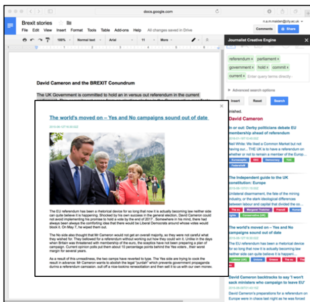
Figure 4: JUICE showing creative search results retrieved for the inserted text (about David Cameron) in the sidebar, and one story in the opened dialogue box
