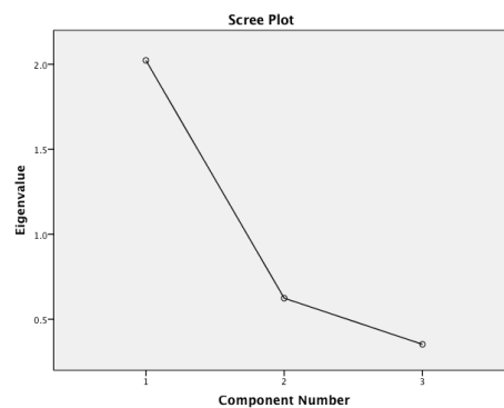
Figure 7.10 Eigenvalue graph
