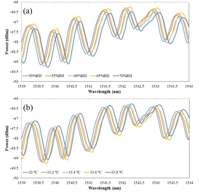
Fig. 8. The displacement of the transmission spectrum for the MZI-SMTF-2 corresponding to changing the: (a) RH and (b) temperature.
