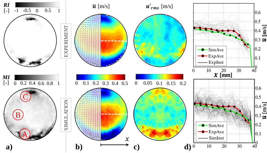
Fig. 10 Comparison between experiment and simulation at 160°CA. Orientation identical to Fig. 5b. a) Relevance index and magnitude index. b) Phase-averaged velocity vectors and magnitude of the experiment and the in-plane components of the simulation. c) Root mean square of resolved velocity fluctuations. d) Phase-averaged velocity magnitude of experiment and simulation as well as instantaneous velocities of experiment (top) and simulation (bottom) along the white dashed line in b.
