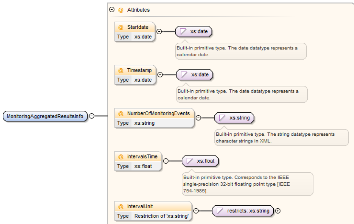
Figure 25 - MonitoringAggregatedResultsInfo sub-element
