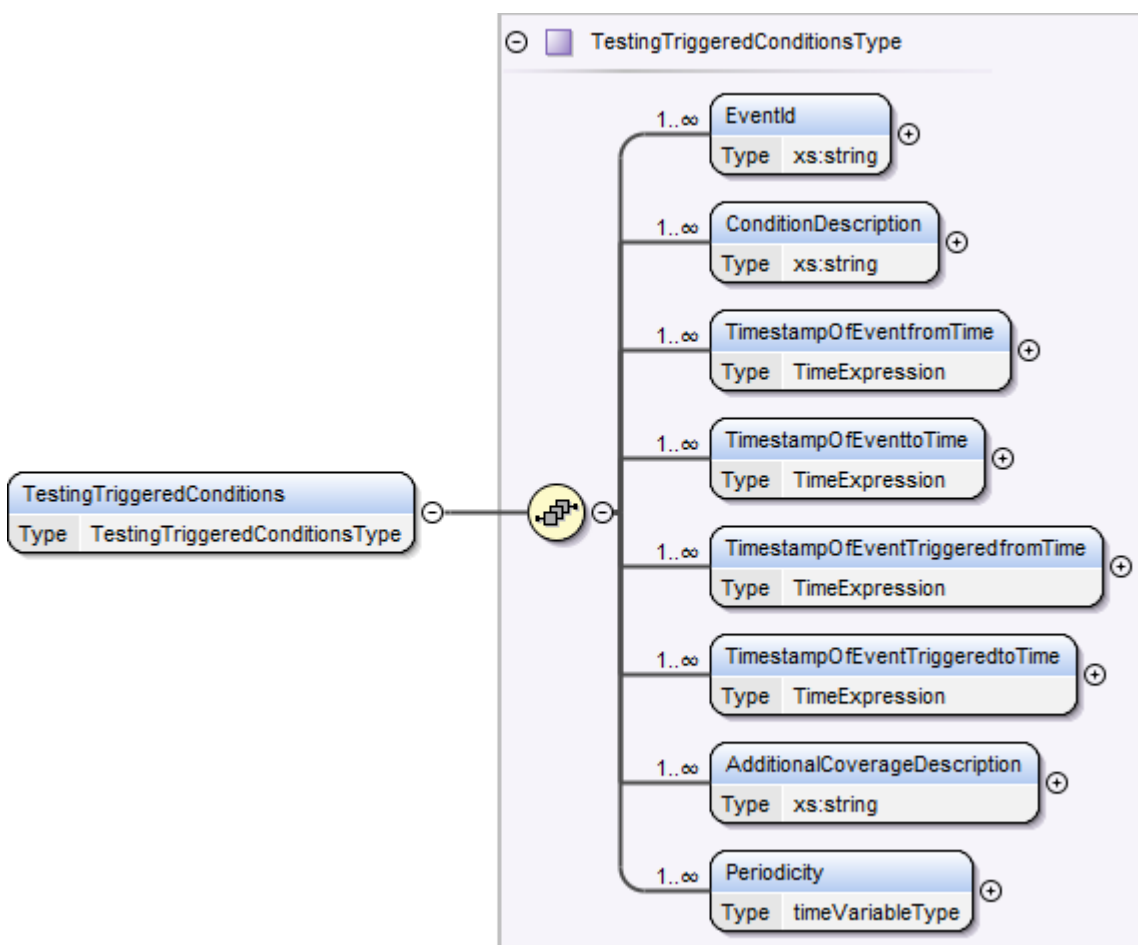
Figure 41 - TestingTriggeredConditionsType
