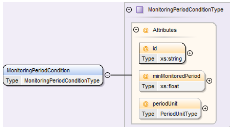
Figure 44 - MonitoringPeriodCondition sub-element
