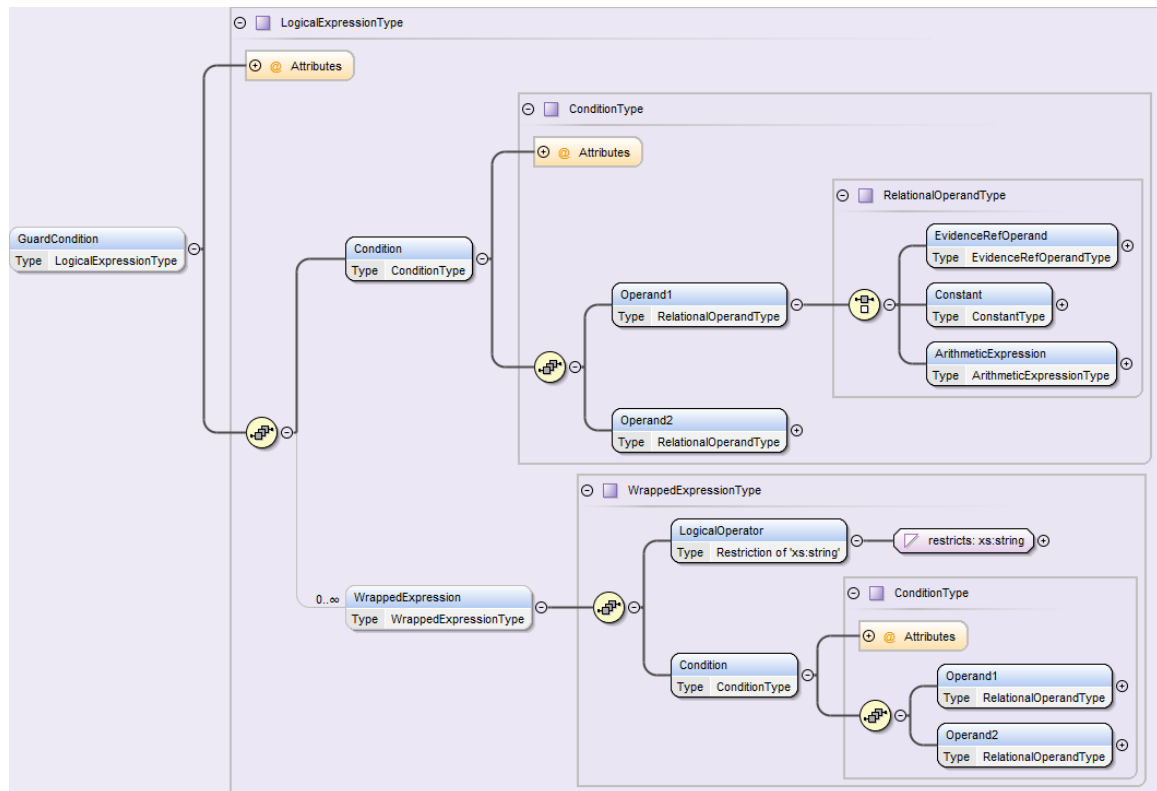
Figure 34 - Guard Conditions
