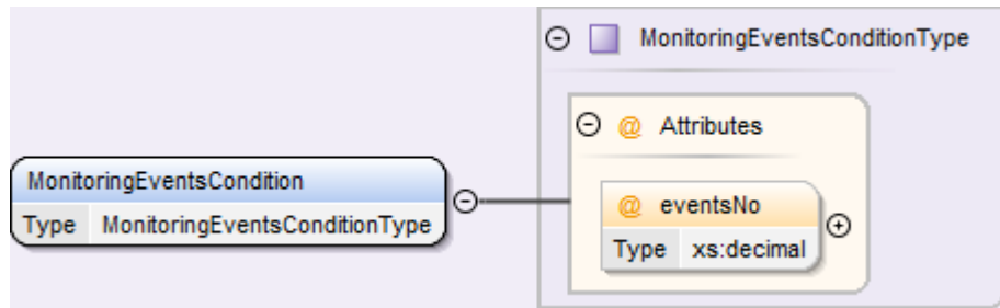
Figure 45 - MonitoringEventsCondition sub-element
