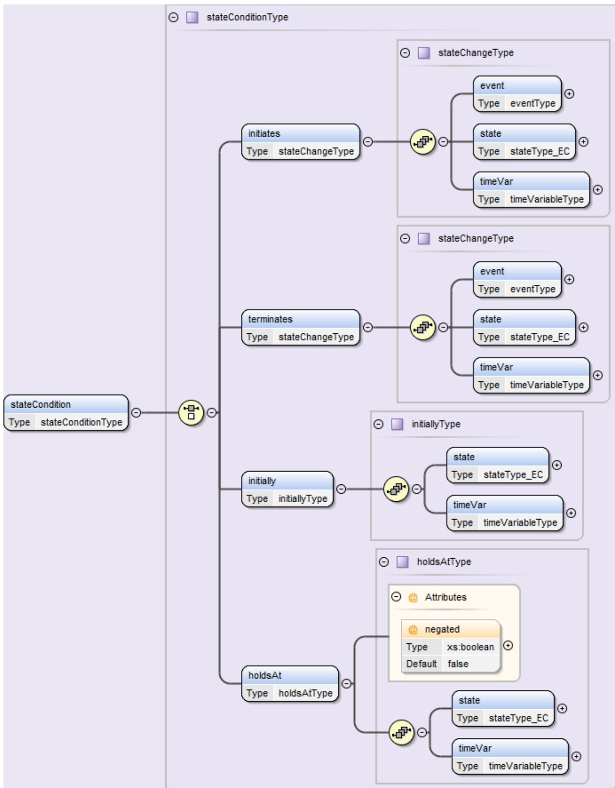
Figure 17 - stateCondition sub-element
