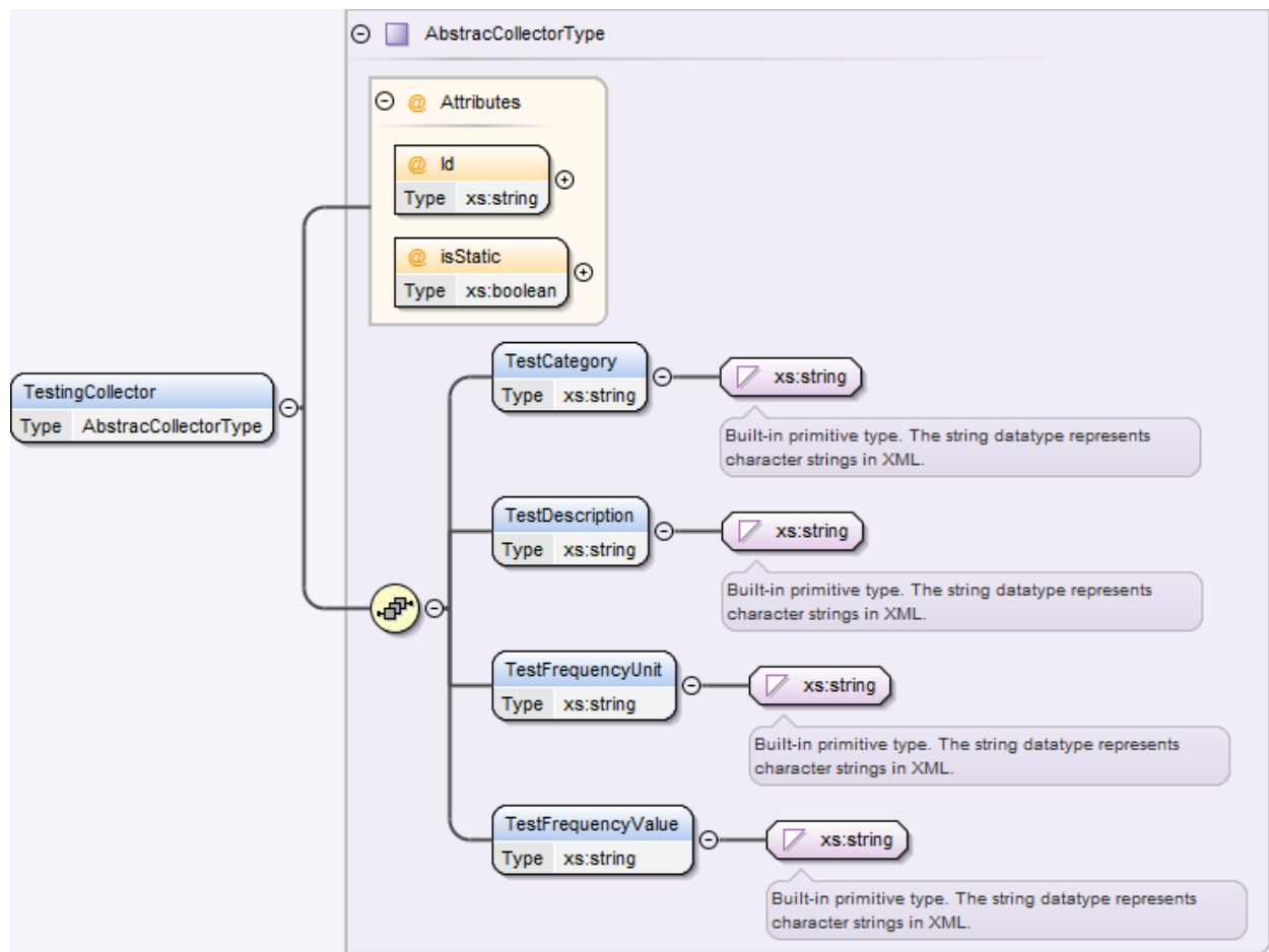
Figure 23 - TestingCollector sub-element
