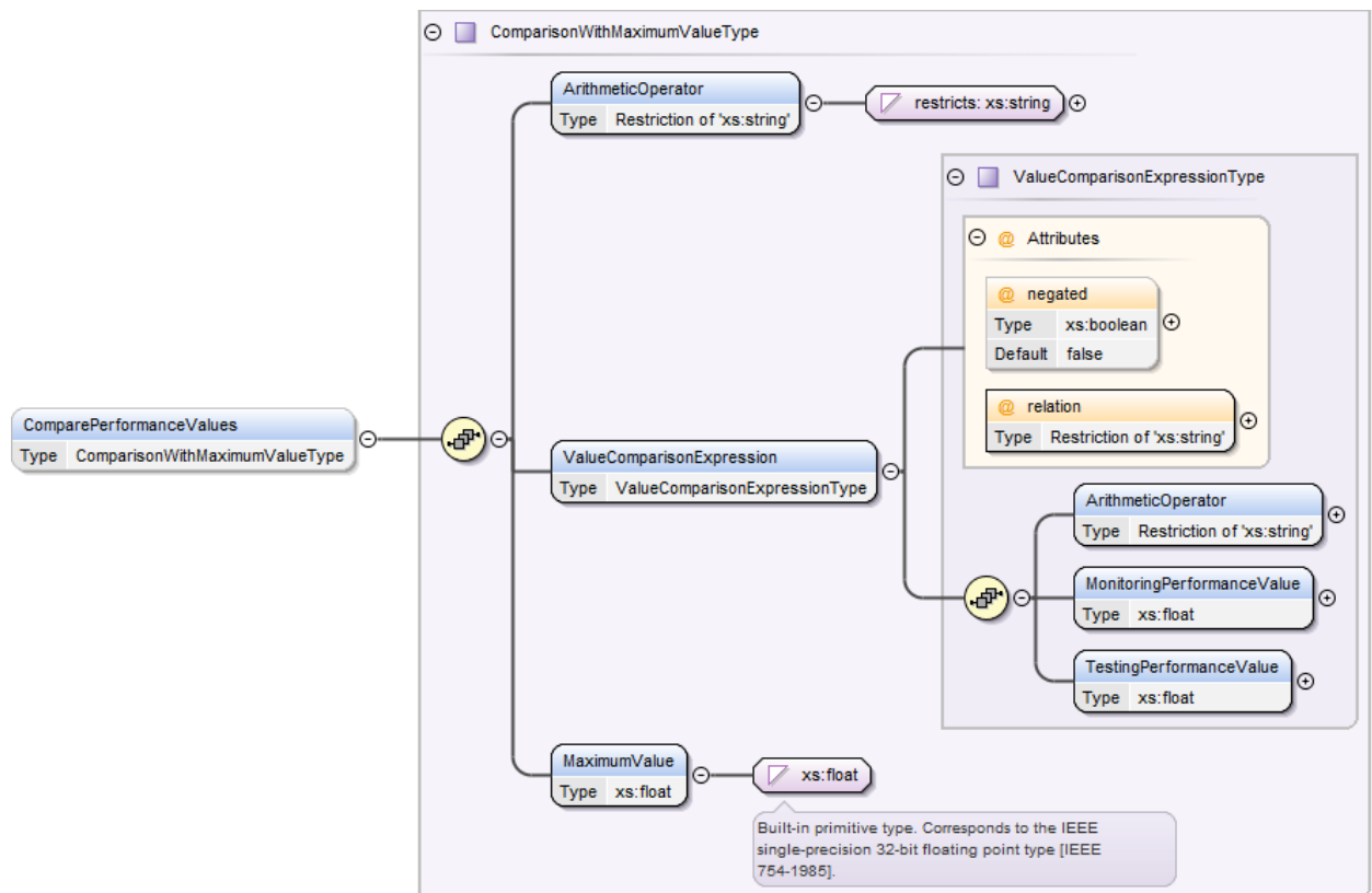
Figure 51 - ComparePerformanceValues sub-element
