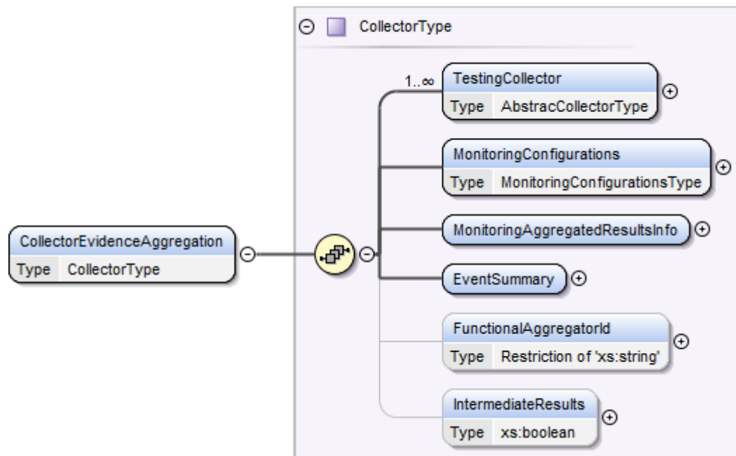
Figure 22 - CollectorsEvidenceAggregation element
