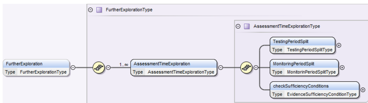
Figure 54 - FurtherExploration element
