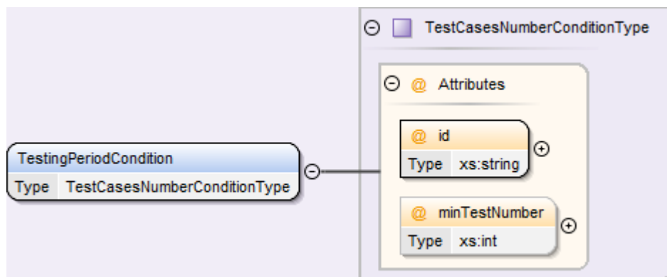
Figure 46 - TestingPeriodCondition sub-element
