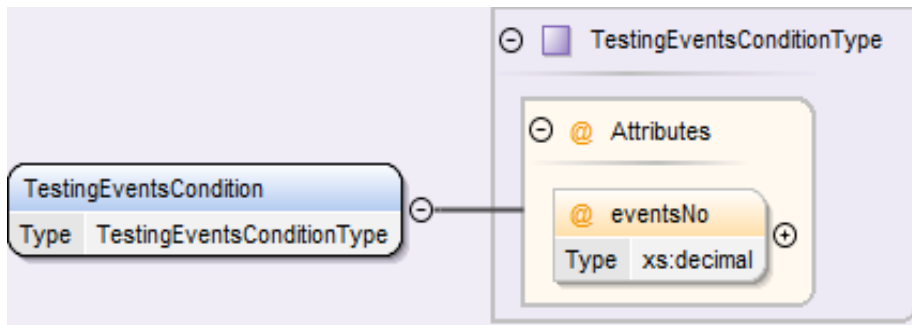
Figure 47 - TestingEventsCondition sub-element
