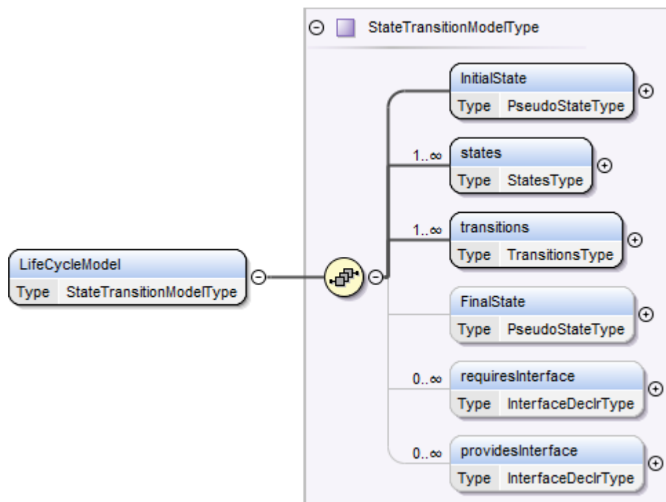
Figure 29 - LifeCycleModel element
