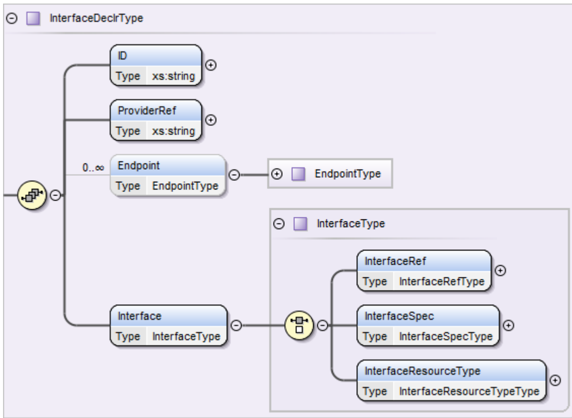
Figure 36 - InterfaceDeclrType
