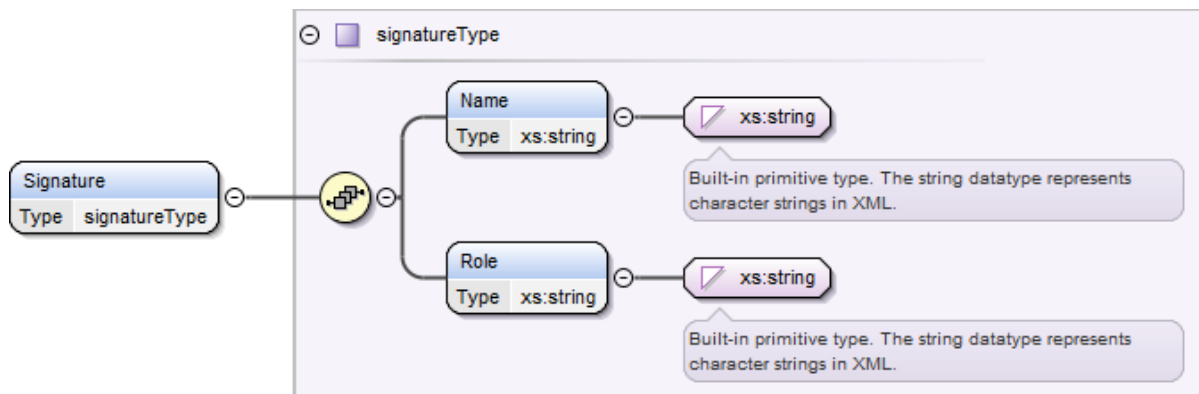
Figure 5 - Signature element
