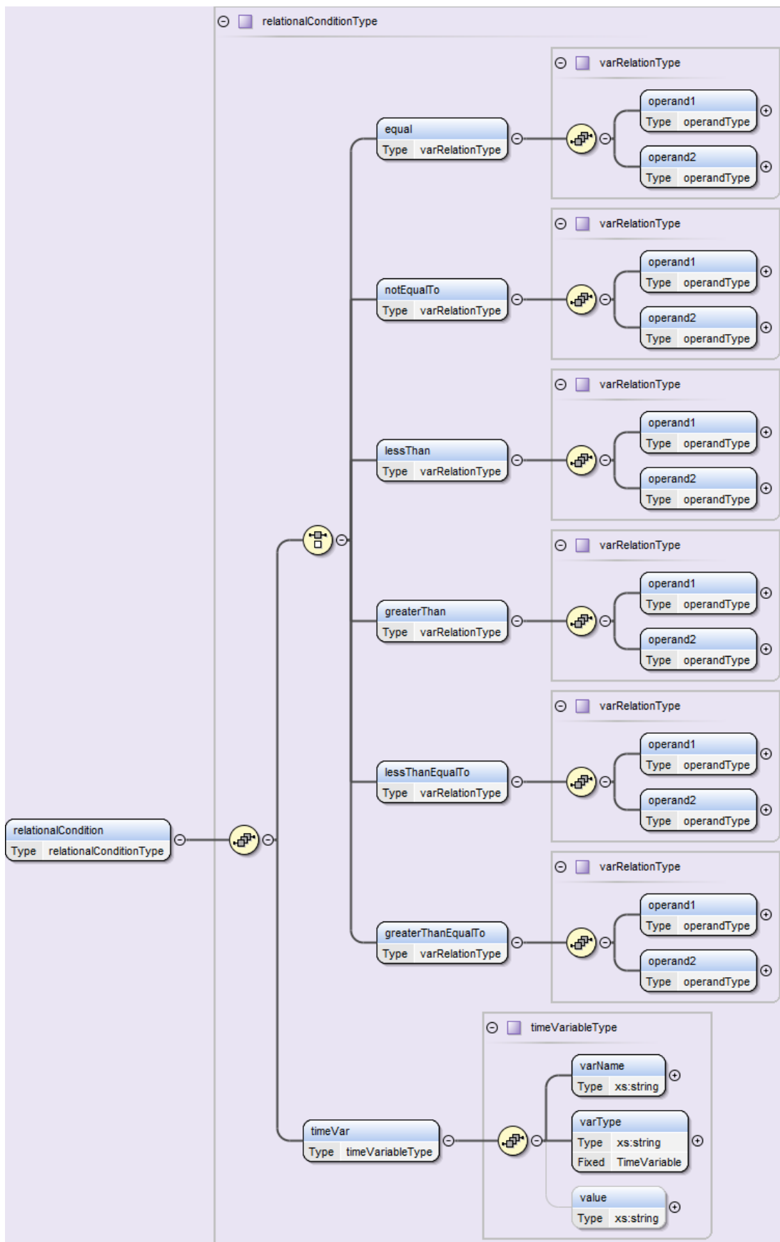
Figure 18 - relationalCondition sub-element
