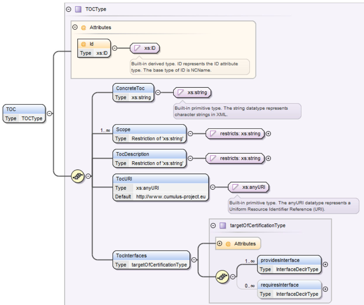
Figure 6 - TOC element
