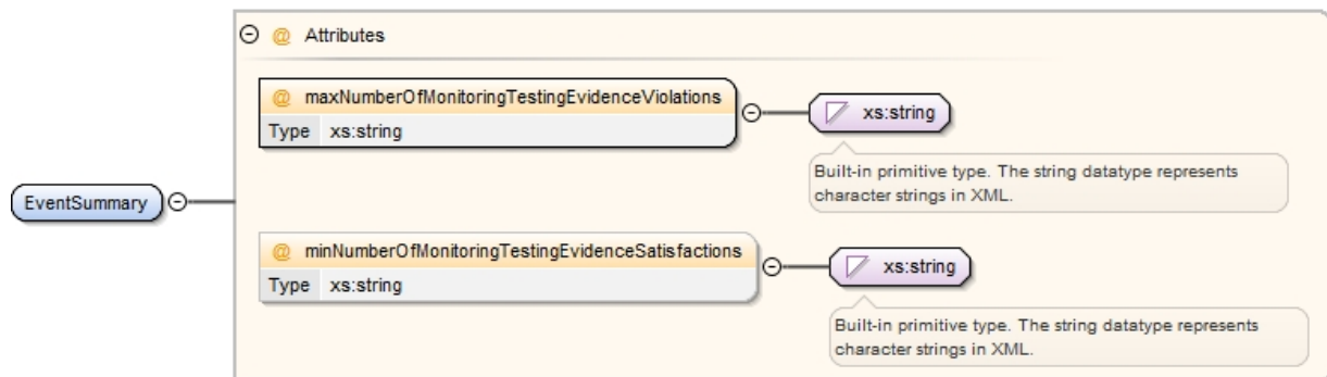
Figure 26 - EventSummary sub-element
