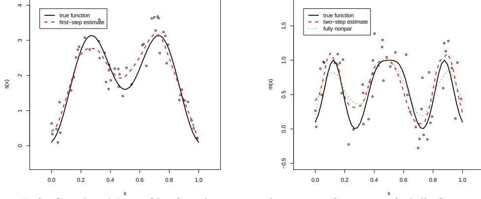
Figure 6: Left: Simulated Data (dots) with \sigma_s = 0.3 from inner function s (solid), first-step estimate (dashed); Right: Simulated Data (dots) with \sigma_m = 0.3 from function composition m (solid), two-step estimate (dashed), usual nonparametric estimate (dotted)
