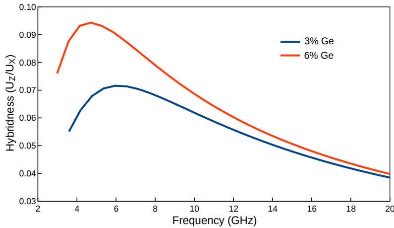
Fig. 4.25 Variation of the modal hybridness of U_{11}^X for different doping concentration.
