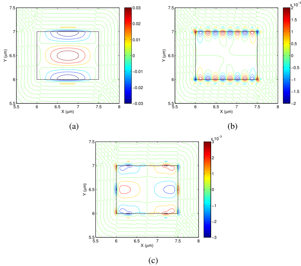
Fig. 6.23 Vector displacement profiles of (a) U_X , (b) U_Y and (c) U_Z components of the U_{13}^X mode at 21.3266 \text{ GHz} .
