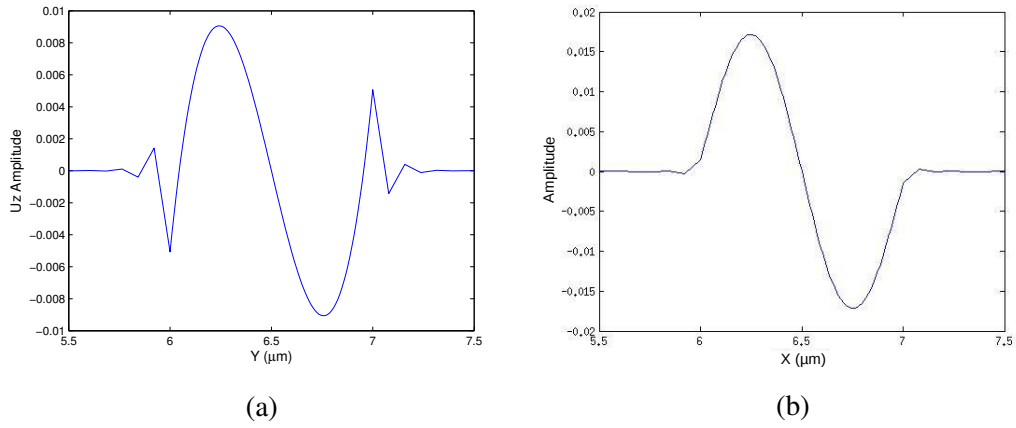
Fig. 6.30 Vector displacement profile of U_Z component of the U_{11}^Y mode at (a) 8.38 GHz and (b) 5.1957 GHz.
