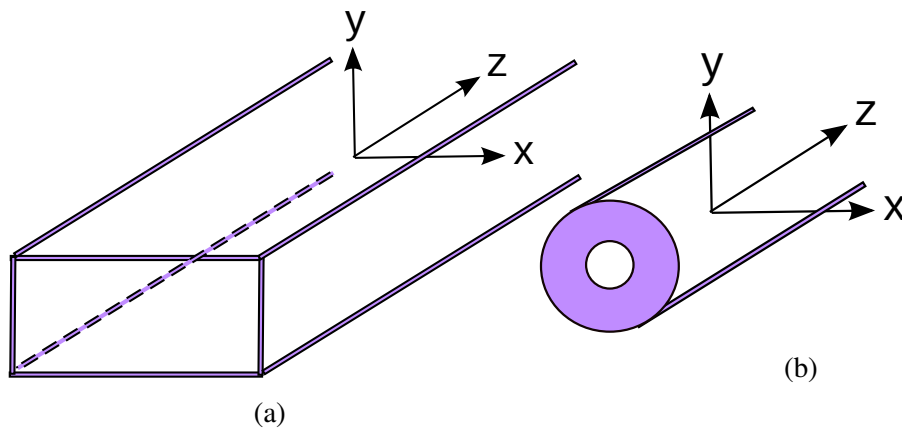
Fig. 2.8 (a) Rectangular and (b) circular two dimensional optical waveguides with indicated direction of propagation.
