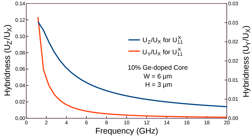
Fig. 5.7 Variations of hybridness with frequency for U_{11}^X mode in 10% Ge-doped core.
