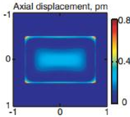
Fig. 6.45 Axial displacement component of the highly hybrid acoustic mode at 5.71 GHz [Laude, 2013].
