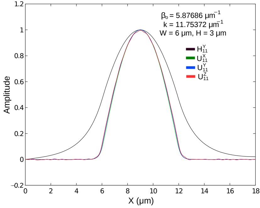
Fig. 5.20 Normalized field and displacement vector profiles along the x -axis.
