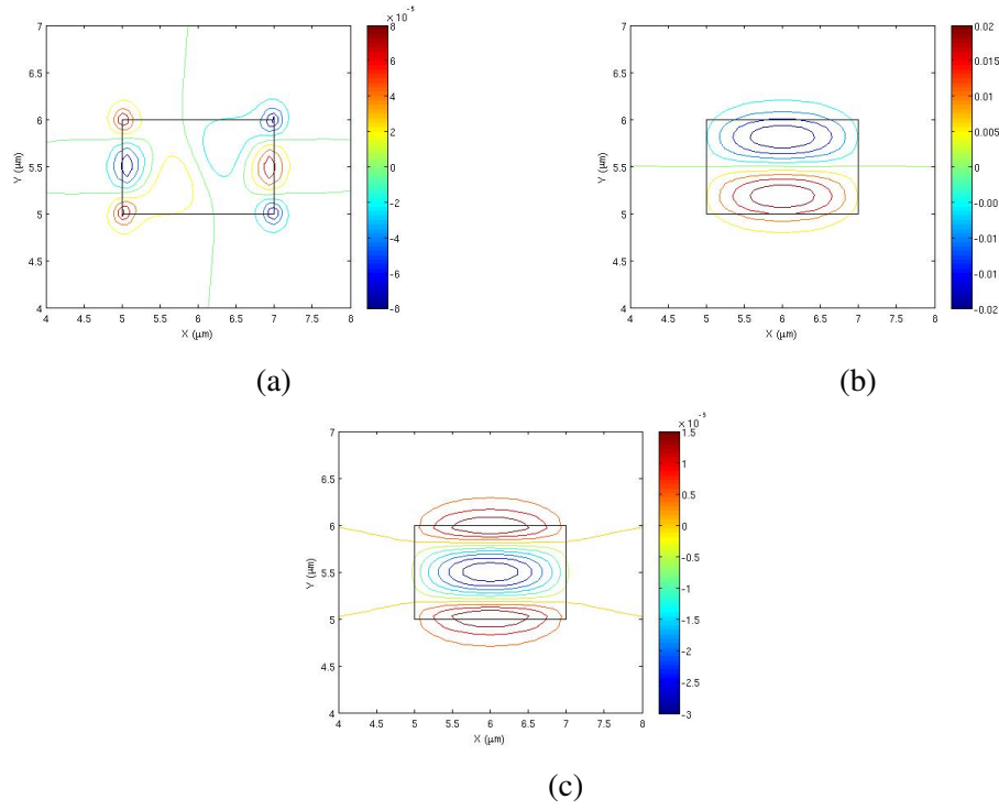
Fig. 4.15 U_X , U_Y and U_Z displacement vectors of the U_{12}^Y mode.
