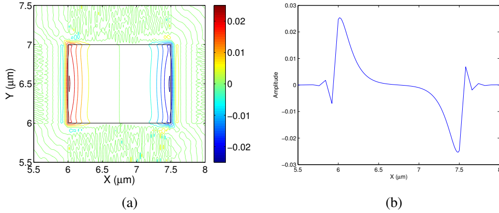
Fig. 6.40 (a) Vector displacement profile and (b) amplitude variations along the x -axis of U_x component of the highly hybrid acoustic mode U_{11}^{HZ} at 10.355 GHz.
