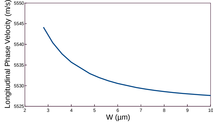
Fig. 5.13 Variation of phase velocity of U_{11}^Z mode with width.
