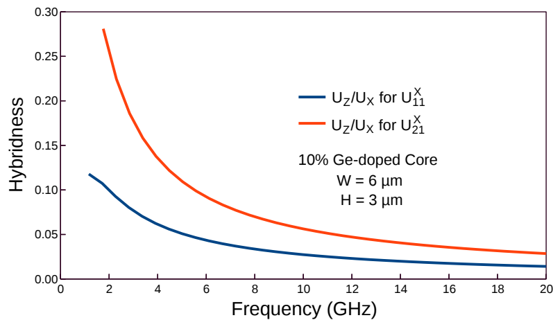
Fig. 5.8 Variations of hybridness with frequency for U_{11}^X and U_{21}^X modes in 10% Ge-doped core.
