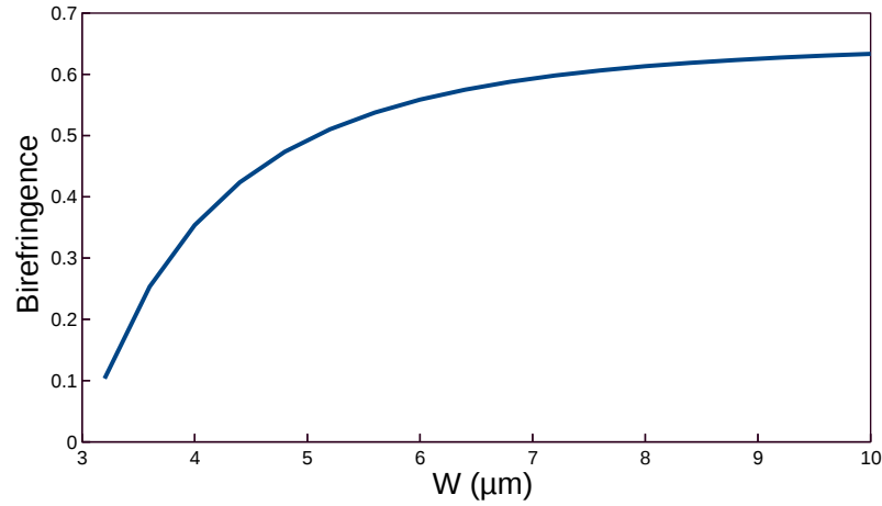
Fig. 5.6 Variation of birefringence with width.
