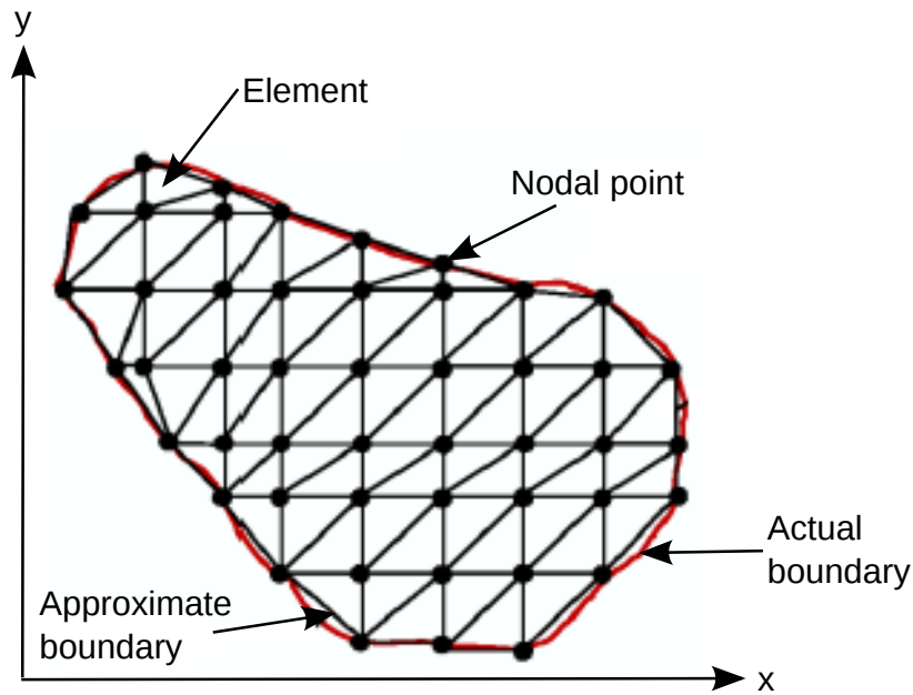
Fig. 3.2 Arbitrary two dimensional domain sub-divided into triangular elements [Leung, Thesis, 2013].
