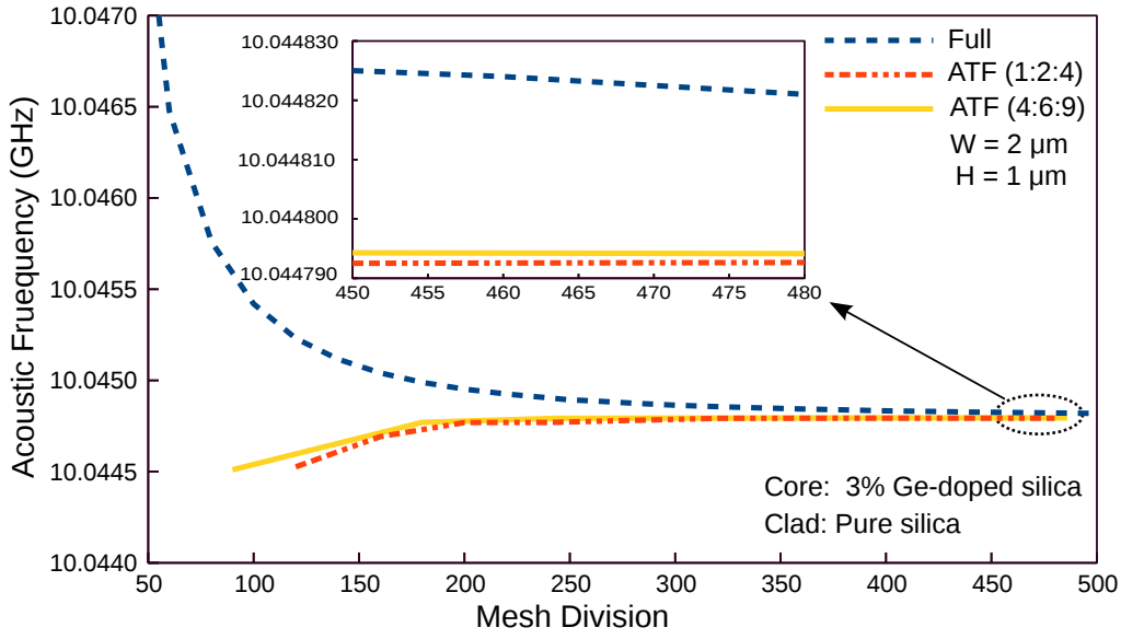
Fig. 3.5 Variation of eigen frequency with the mesh division for the U_{11}^x mode at k = 17 \mu m^{-1} .
