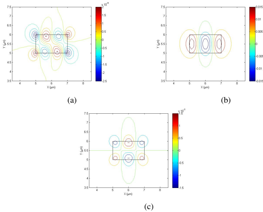
Fig. 4.16 U_X , U_Y and U_Z displacement vectors of the U_{31}^Y mode.
