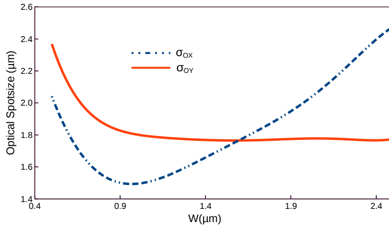
Fig. 6.4 Variations of spotsizes with width for H_{11}^Y mode in air caldded silica strip waveguide.
