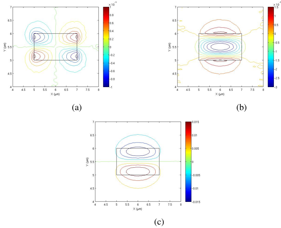
Fig. 4.33 U_X , U_Y and U_Z displacement vectors of the U_{12}^Z mode.
