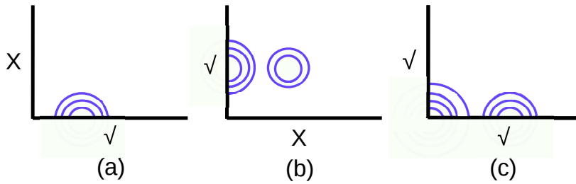
Fig. B.3 Drawn two-fold symmetric displacement profile of (a) U_X , (b) U_Y and (c) U_Z components of U_{21}^X mode fall in category 3.
