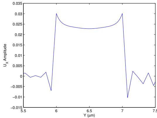
Fig. 6.9 Variations of amplitude along y -axis of U_X component of the fundamental quasi-shear acoustic mode U_{11}^X at 8 GHz.
