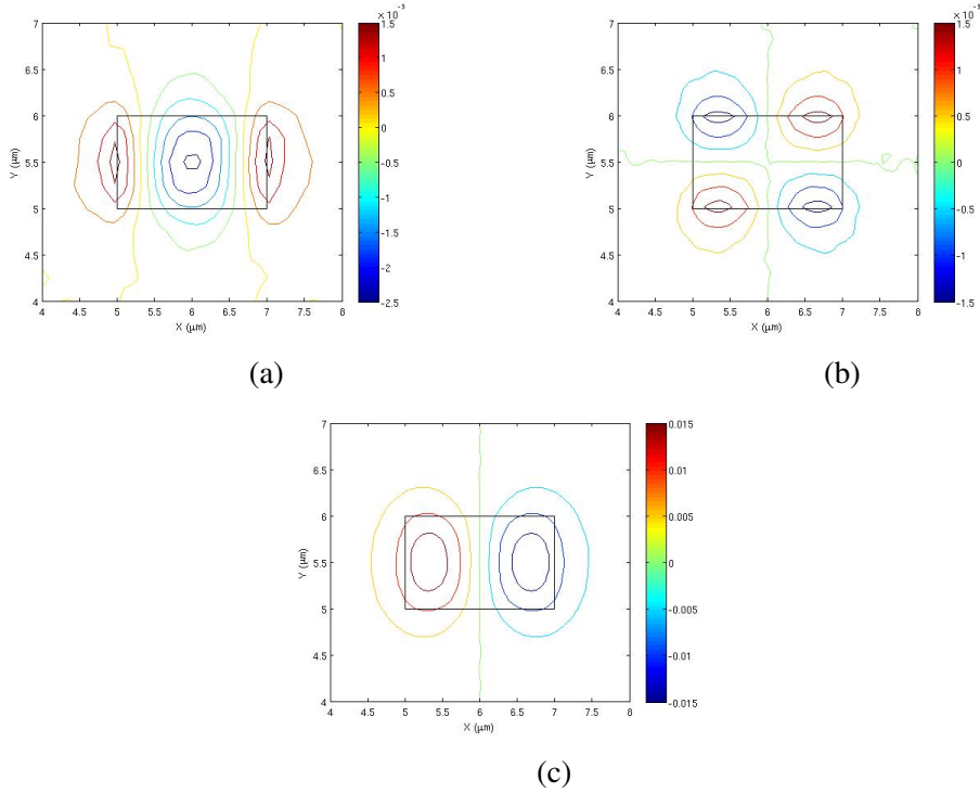
Fig. 4.32 U_X , U_Y and U_Z displacement vectors of the U_{21}^Z mode.
