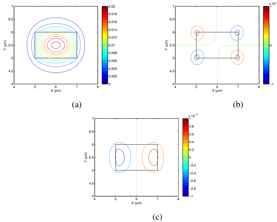
Fig. 4.37 U_X , U_Y and U_Z displacement vectors of the fundamental quasi-shear mode.
