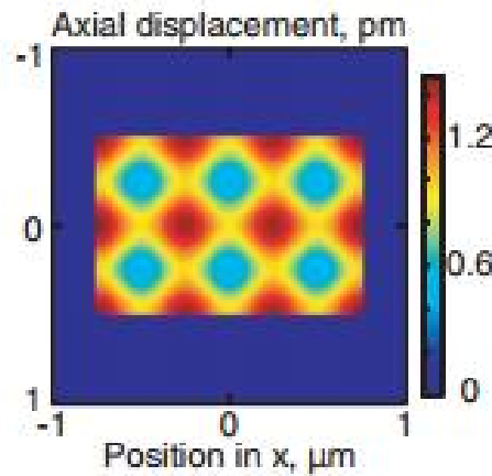
Fig. 6.53 Axial displacement component of the highly hybrid acoustic mode at 9.81 \text{ GHz} [Laude, 2013].
