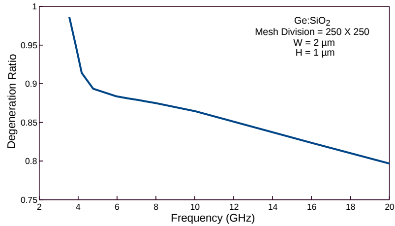
Fig. 4.20 Degeneration ratio against the acoustic frequency for U_y displacement vectors of the U_{11}^x mode.
