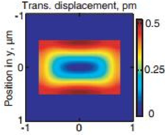
Fig. 6.38 Transverse plane displacement component of the highly hybrid acoustic mode at 5.71 \text{ GHz} [Laude, 2013].
