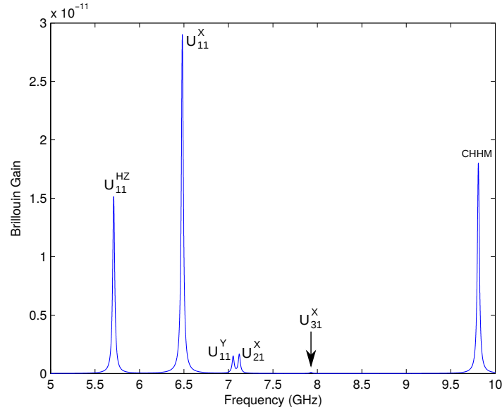
Fig. 6.58 Brillouin gain spectrum of strip silica waveguide surrounded by air between 5 GHz to 10 GHz.
