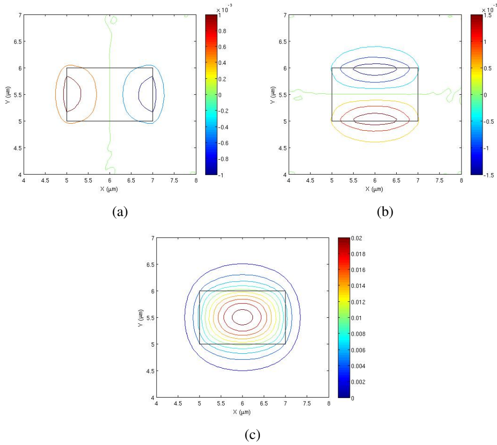
Fig. 4.29 U_X , U_Y and U_Z displacement vectors of the U_{11}^Z mode.
