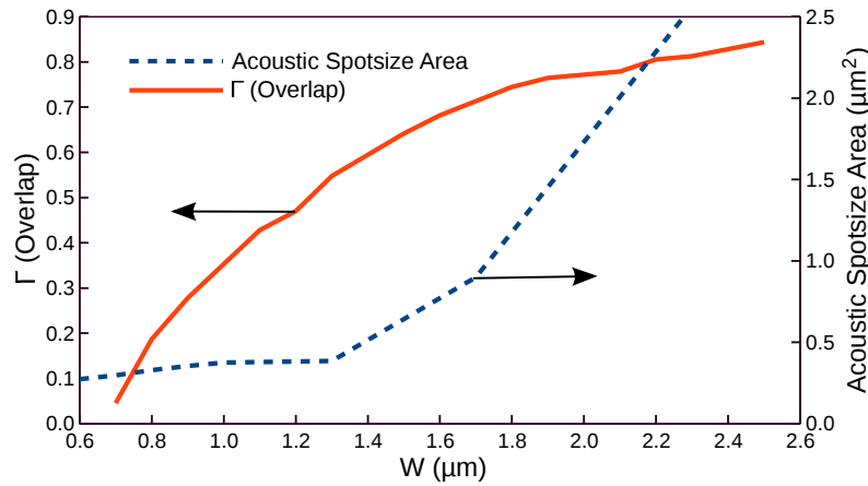
Fig. 6.54 Acoustic spotsizes area (at k = 10\mu m^{-1} ) and Overlap between U_X component of U_{11}^X acoustic mode and H_Y field of quasi-TE optical mode with W .
