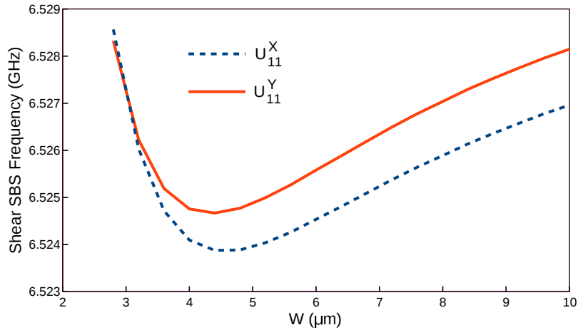
Fig. 5.24 Shear SBS Frequency shift with guide width.
