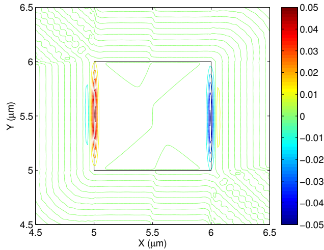
Fig. 3.10 Displacement vector profile of the U_X component of U_{21}^X acoustic mode at k = 200 \text{ m}^{-1} .
