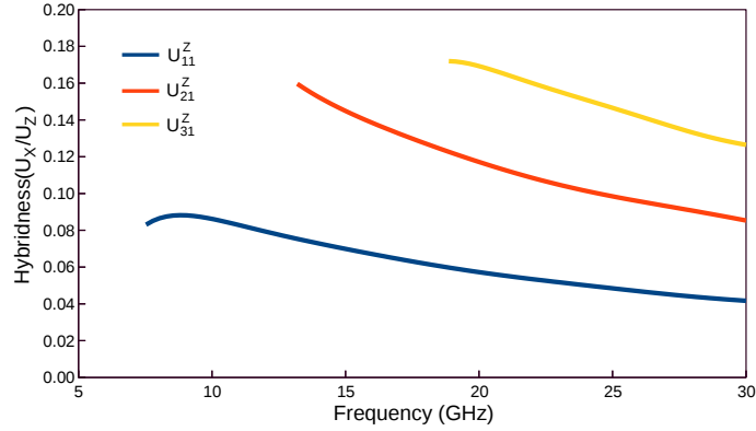
Fig. 4.35 Variation of the modal hybridness for the higher order modes with dominant U_Z component.
