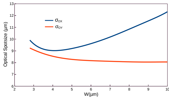
Fig. 5.16 Variations of spot sizes with width for H_{11}^Y mode in 10% Ge-doped core.
