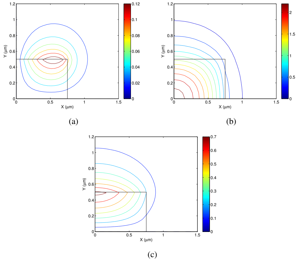
Fig. 6.2 H_x , H_y and H_z field profiles of the fundamental quasi-TE optical mode (only the quarter of the waveguide is shown).
