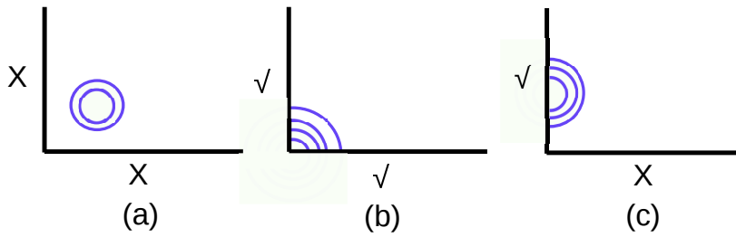
Fig. B.2 Drawn two-fold symmetric displacement profile of (a) U_X , (b) U_Y and (c) U_Z components of U_{11}^Y mode fall in category 2.
