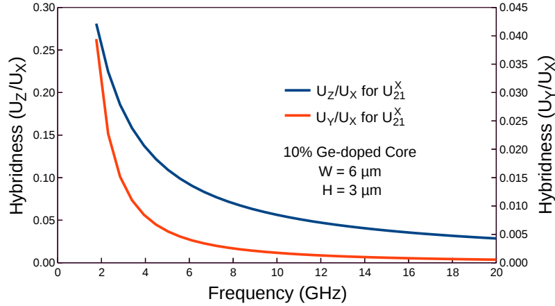
Fig. 5.9 Variations of hybridness with frequency for U_{21}^X mode in 10% Ge-doped core.
