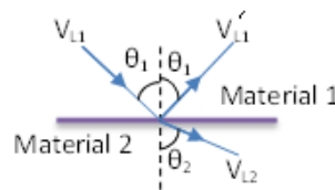
Fig. 2.4 Reflected and refracted longitudinal acoustic waves [NDT Course Material].
