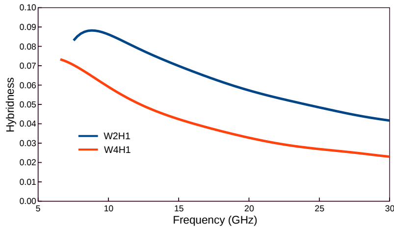
Fig. 4.36 Variation of the modal hybridness of U_{11}^Z for different width.
