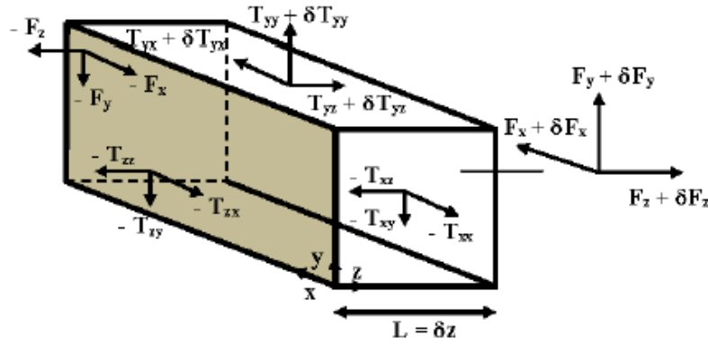
Fig. 2.3 General stress components in a cube [Auld, 1973].
