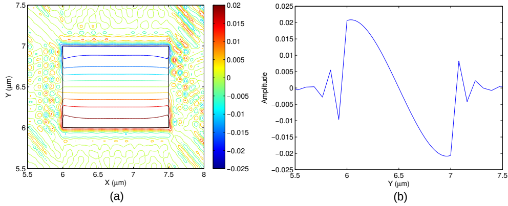
Fig. 6.35 (a) Vector displacement profile and (b) amplitude variations along the y -axis of U_Y component of the highly hybrid acoustic mode U_{11}^{HZ} at 3.24 \text{ GHz} .
