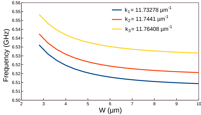
Fig. 5.26 Considered k at three places on SBS Frequency shift for U_{11}^X with guide width.
