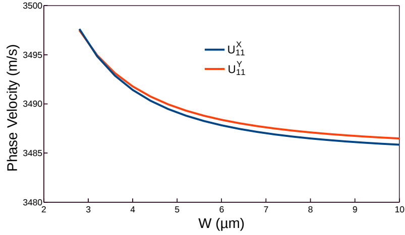
Fig. 5.5 Variation of phase velocity of U_{11}^X and U_{11}^Y modes with width.
