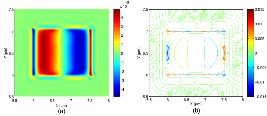
Fig. 6.17 Vector displacement profiles of U_Z component of the fundamental quasi-shear U_{11}^X acoustic mode (a) at 10 GHz and (b) at 8 GHz.
