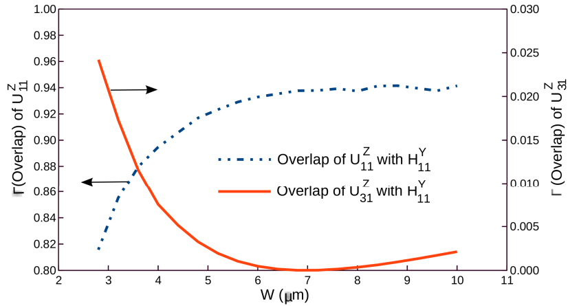
Fig. 5.21 Overlap of H_Y field of the H_{11}^Y mode with the U_Z displacement vector of the U_{11}^Z and U_{31}^Z modes with W .
