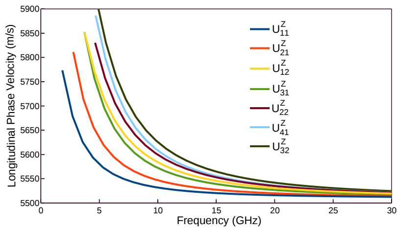
Fig. 5.12 Variations of the phase velocities with the acoustic frequencies for the longitudinal modes.
