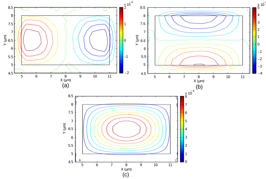
Fig. 5.11 Displacement vector profiles (a) U_X , (b) U_Y and (c) U_Z of the U_{11}^Z acoustic mode.
