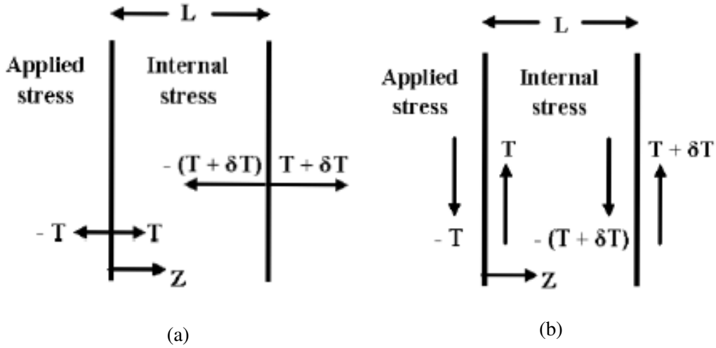
Fig. 2.2 For a slab of infinitesimal length L (a) stress in the longitudinal direction and (b) stress in the transverse direction [Sriratanavaree, Thesis, 2014].
