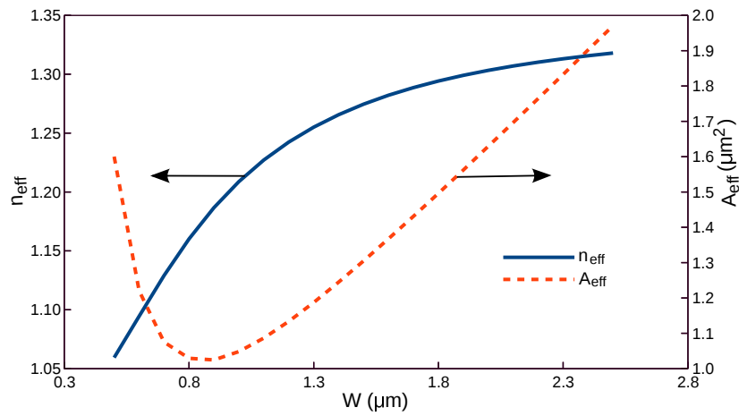
Fig. 6.3 Variation of effective index and effective area of the H_y field profile of quasi-TE optical mode with width, W .
