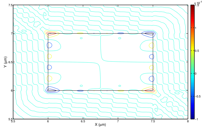
Fig. 6.27 Vector displacement profile of U_X component of the U_{11}^Y mode at 21.0686 GHz.
