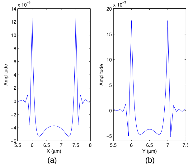
Fig. 6.46 Variations of amplitude along (a) x -axis (b) y -axis of U_Z component of the highly hybrid acoustic mode U_{11}^{HZ} at 7.12\text{ GHz} .
