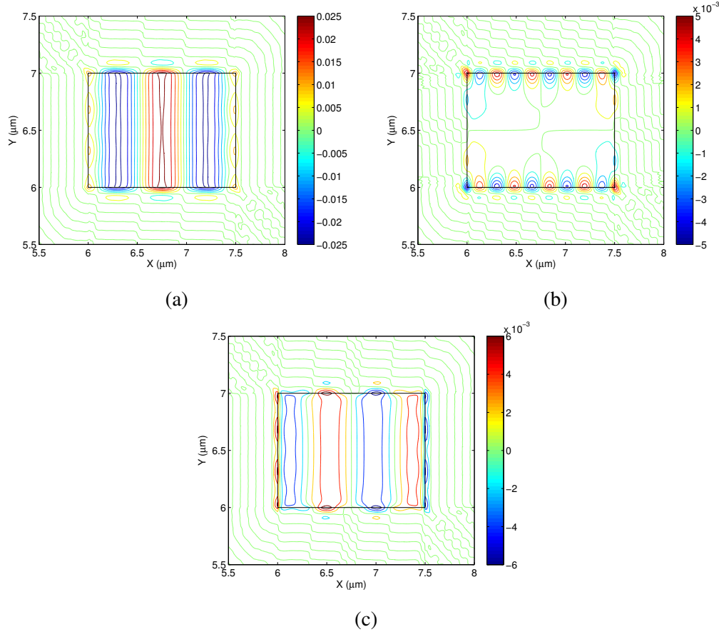
Fig. 6.20 Vector displacement profiles of (a) U_X , (b) U_Y and (c) U_Z components of the U_{31}^X mode at 21.37 GHz .
