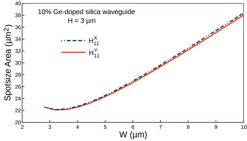
Fig. 5.18 Variations of the spotsize area of the H_{11}^Y and H_{11}^X modes with the guide width, W .
