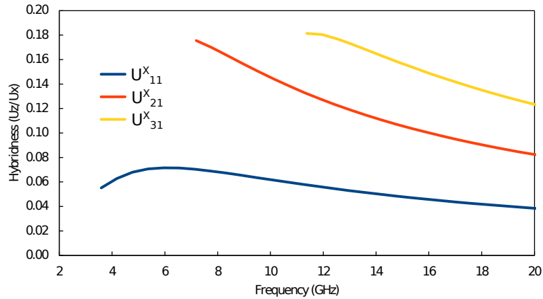
Fig. 4.23 Variation of the modal hybridness for the higher order modes with dominant U_X component.
