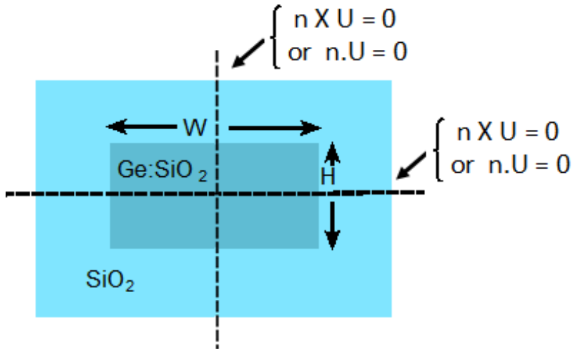
Fig. 4.2 Symmetry boundary conditions for planar silica waveguide.
