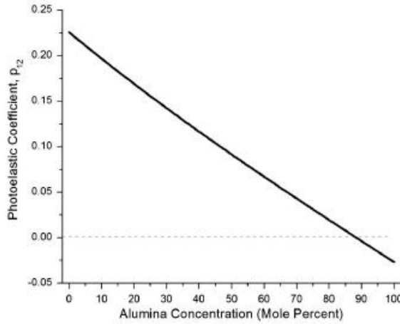
Fig. 5.30 Photoelastic constant, p_{12} , as a function of alumina concentration in silica [Dragic, 2013].
