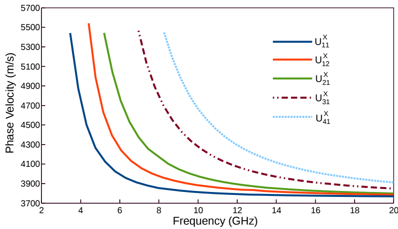
Fig. 6.5 Variation of the phase velocities with the acoustic frequencies for the fundamental and higher order acoustic quasi-shear modes.
