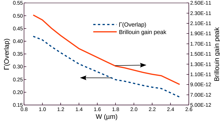
Fig. 6.57 Variations of Brillouin gain peak ( g_B ) of highly hybrid acoustic mode U_{11}^{HZ} and variations of overlap between its U_Z component and H_Y field of quasi-TE optical mode with the guide width.
