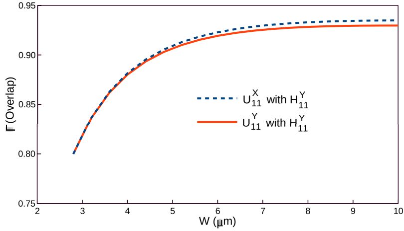
Fig. 5.23 Variations of the H_Y field overlap of the H_{11}^Y mode with the U_{11}^X and U_{11}^Y modes with the width.
