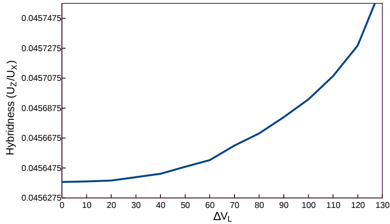
Fig. 4.40 Modal hybridness variation with the incorporated difference in longitudinal velocities.
