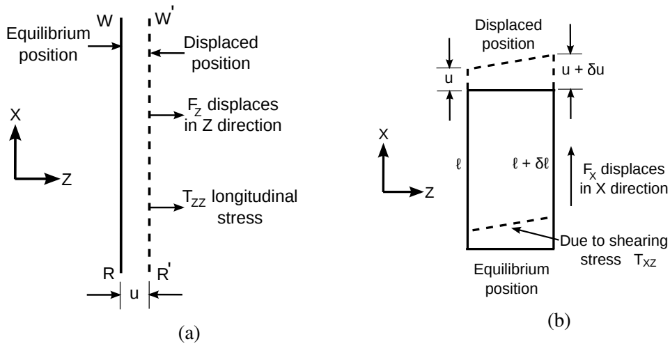
Fig. A.2 Effects of (a) longitudinal and (b) shear stresses normal to the surface [Sriratanavaree, Thesis, 2014].
