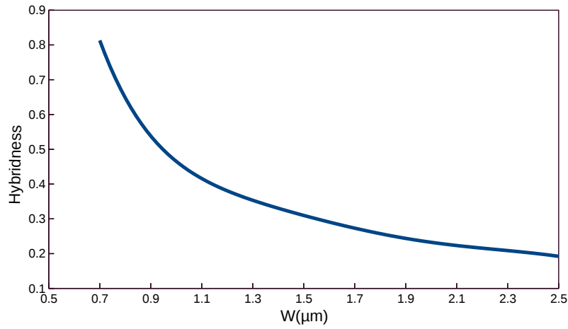
Fig. 6.33 Variation of hybridness of the U_{11}^X acoustic mode with W at k = 10 \mu m^{-1} .
