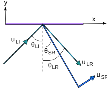
Fig. 2.5 Reflected longitudinal and shear waves from incident of a longitudinal wave on a free surface [Sriratanavaree, Thesis, 2014].
