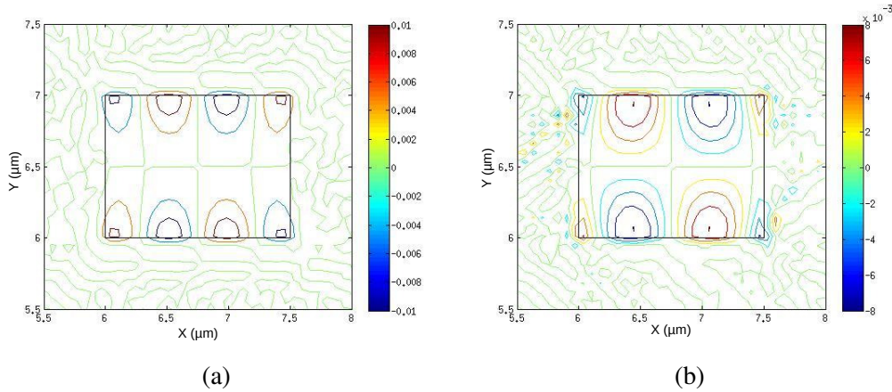
Fig. 6.15 Vector displacement profiles of U_Y component of the fundamental quasi-shear U_{11}^X acoustic mode (a) at 8 GHz and (b) 4 GHz.
