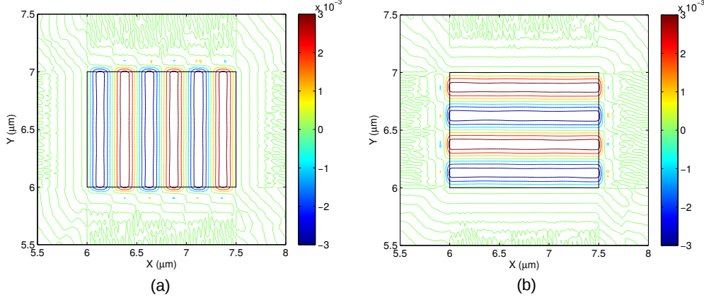
Fig. 6.48 Vector displacement profiles (a) of U_X component and (b) of U_Y component of the complex highly hybrid acoustic mode (CHHM) at 9.81 GHz.
