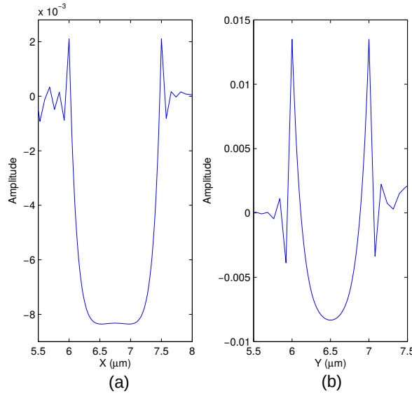
Fig. 6.43 Variations of amplitude along (a) x -axis (b) y -axis of U_Z component of the highly hybrid acoustic mode U_{11}^{HZ} at 4.53 GHz.
