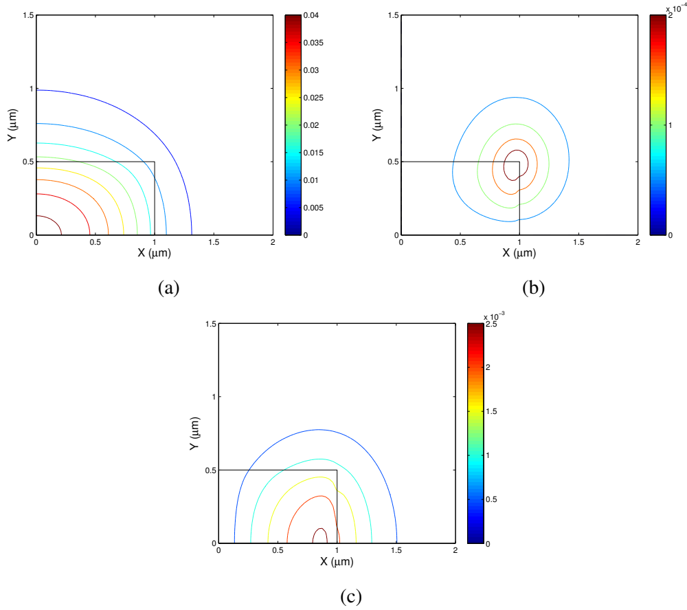
Fig. 4.5 U_X , U_Y and U_Z displacement vectors of the U_{11}^Z mode exploiting two-fold symmetry.
