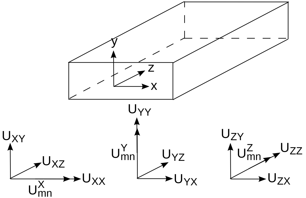
Fig. 3.1 Hybrid components of shear and longitudinal acoustic modes and planar waveguide.
