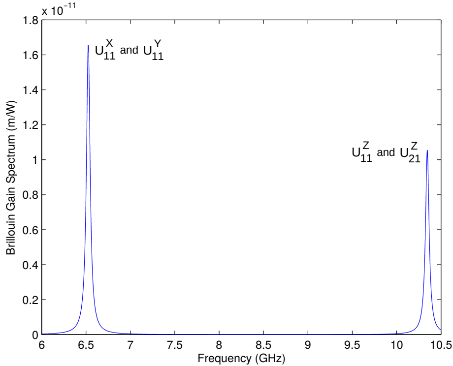
Fig. 5.32 Brillouin gain spectrum of 10% Ge-doped silica waveguide between 6 GHz to 10.5 GHz.
