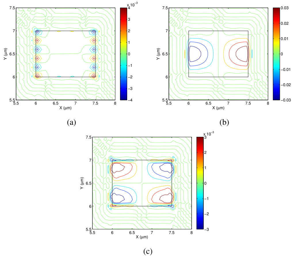
Fig. 6.31 Vector displacement profiles of (a) U_X , (b) U_Y and (c) U_Z components of the U_{21}^Y mode at 21.4262 GHz.
