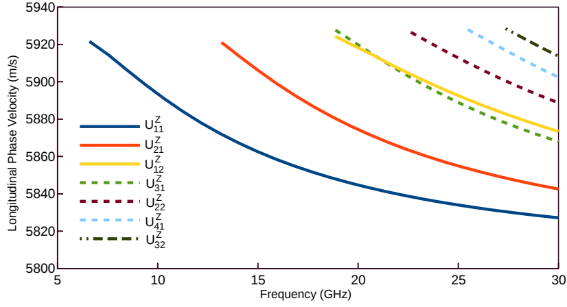
Fig. 4.31 Dispersion curves of acoustic longitudinal U_{mn}^Z modes.
