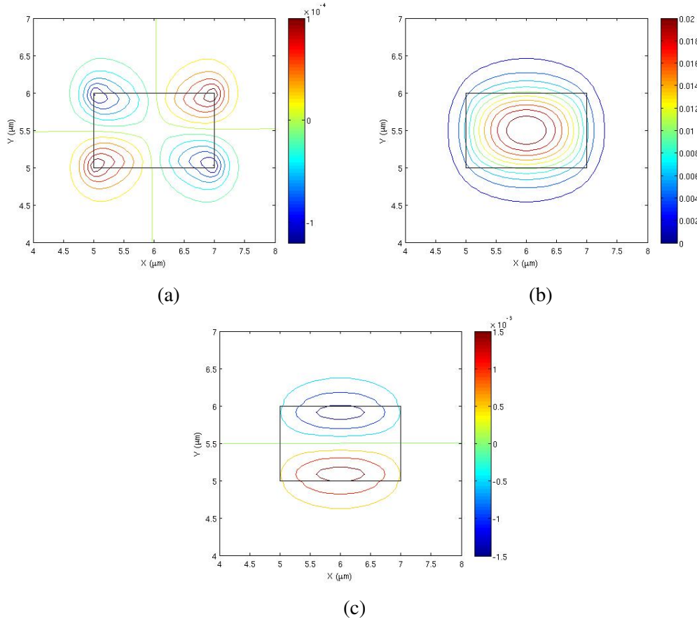
Fig. 4.6 U_X , U_Y and U_Z displacement vectors of the U_{11}^Y mode at k = 17 \mu m^{-1} .
