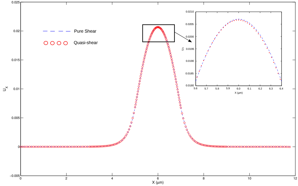
Fig. 4.38 The dominant U_X component of the fundamental quasi-shear mode along x -axis at 16 GHz.
