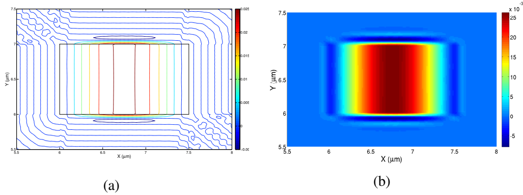
Fig. 6.6 (a) Contour and (b) coloured, vector displacement profiles of U_X component of the fundamental quasi-shear U_{11}^X acoustic mode at 21 GHz.
