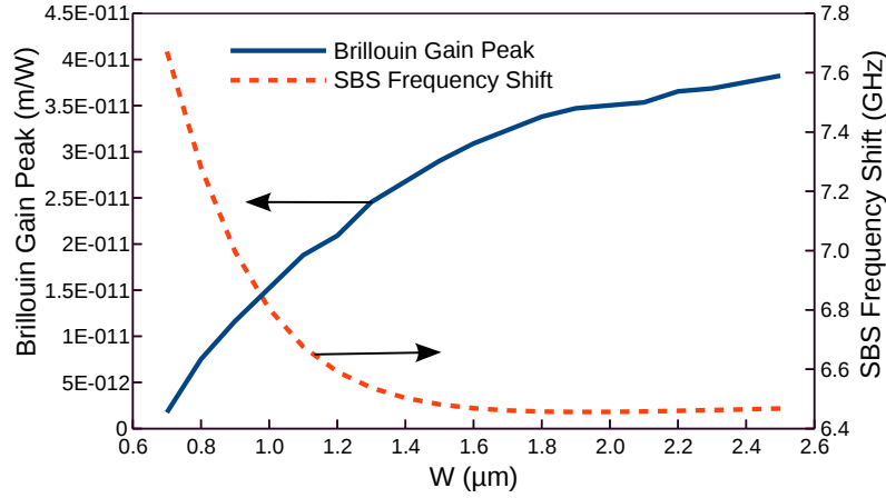
Fig. 6.55 SBS frequency shift and variations of Brillouin gain peak ( g_B ) of U_X displacement vector of the U_{11}^X mode with W .
