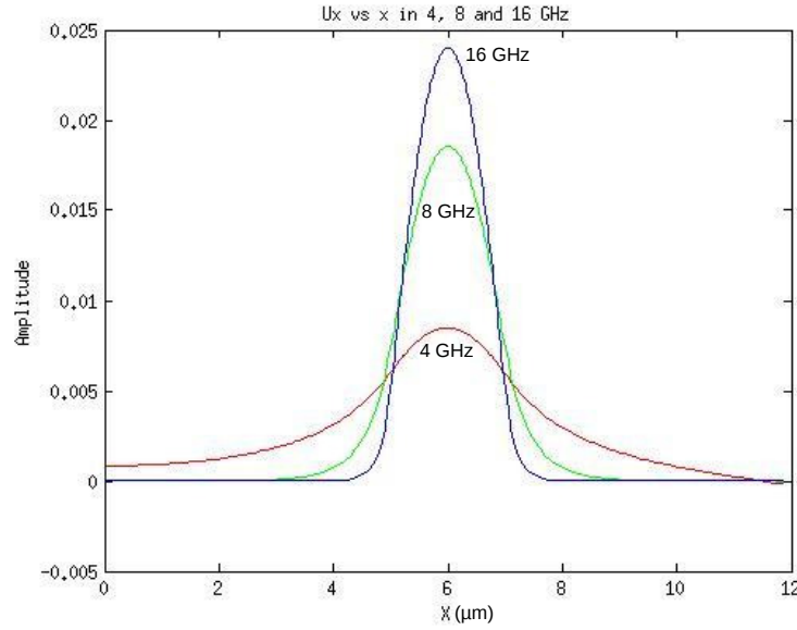
Fig. 4.4 The dominant U_X component of the U_{11}^X mode at 4, 8 and 16 GHz acoustic frequencies.
