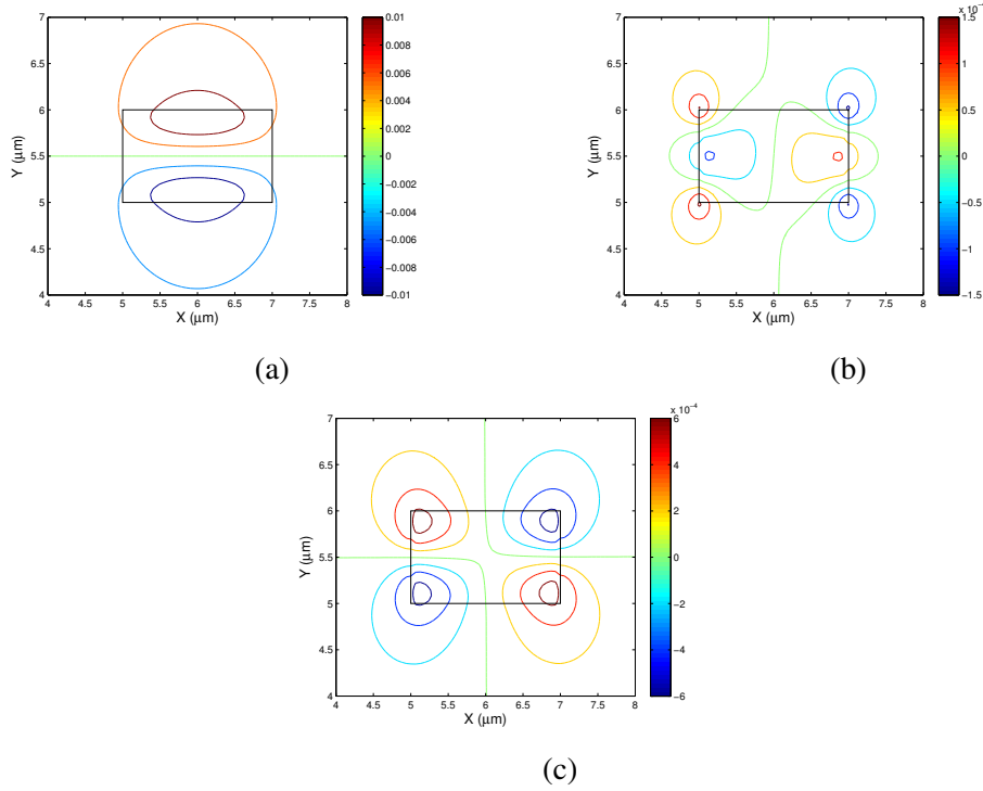
Fig. 4.12 U_X , U_Y and U_Z displacement vectors of the U_{12}^X mode.
