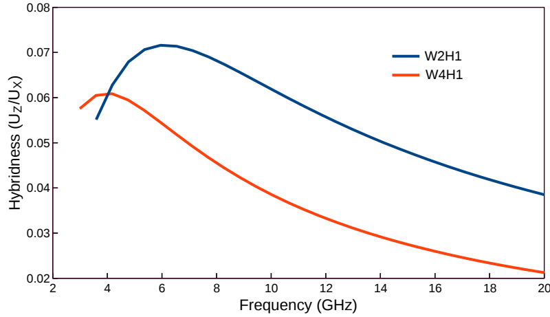
Fig. 4.24 Variation of the modal hybridness of U_{11}^X for different width.
