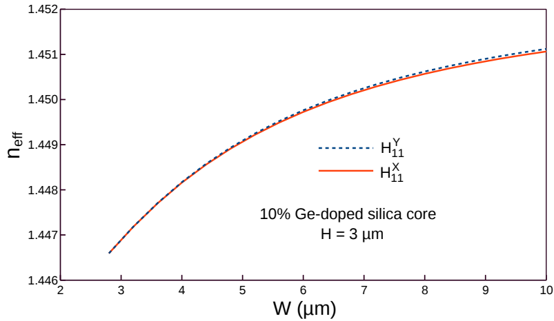
Fig. 5.17 Variations of n_{eff} with the guide width for the optical quasi-TE and quasi-TM modes.
