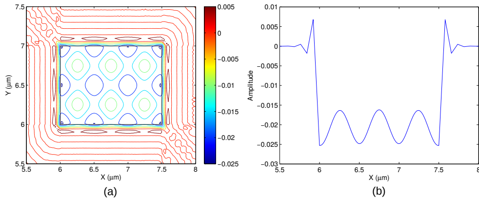
Fig. 6.52 (a) Vector displacement profile and (b) variations of amplitude along x -axis of the U_Z component of the CHHM mode at 9.81 \text{ GHz} .
