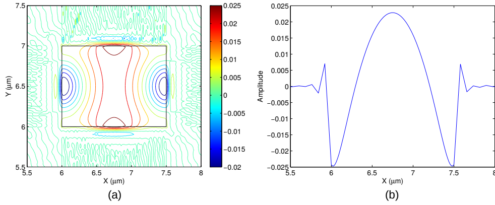
Fig. 6.8 (a) Vector displacement profile and (b) variations of amplitude along x -axis of U_X component of the fundamental quasi-shear acoustic mode U_{11}^X at 8 GHz.
