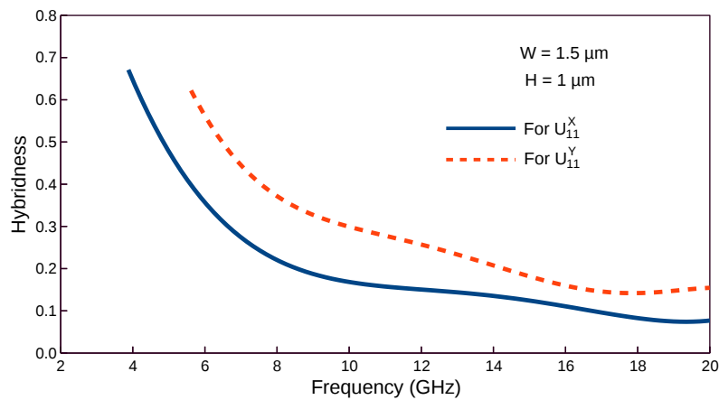
Fig. 6.32 Variation of the hybridness with frequency for the U_{11}^X and U_{11}^Y modes.
