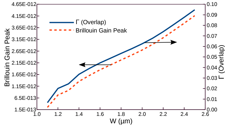
Fig. 6.56 Variations of Brillouin gain peak ( g_B ) of U_{21}^X acoustic mode and variations of overlap between its U_Z component and H_Y field of quasi-TE optical mode with the guide width.
