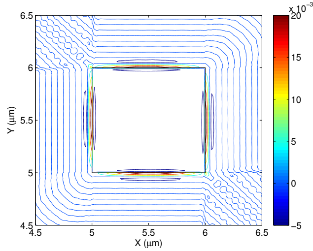
Fig. 3.12 Displacement vector profile of the U_Z component of U_{21}^x acoustic mode at k = 200 \text{ m}^{-1} .
