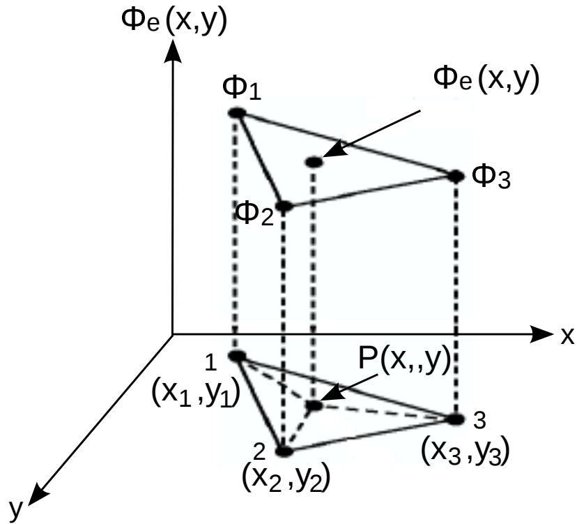
Fig. 3.4 A typical first order triangular element [Leung, Thesis, 2013].
