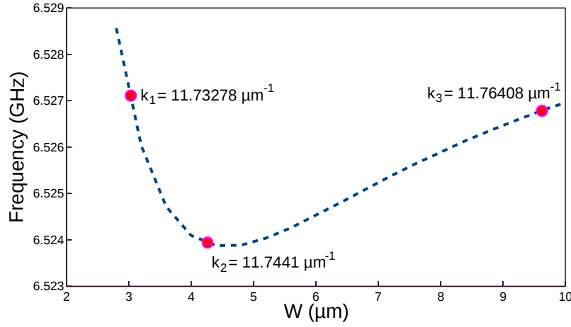
Fig. 5.25 Considered k at three places on SBS Frequency shift for U_{11}^X with guide width.
