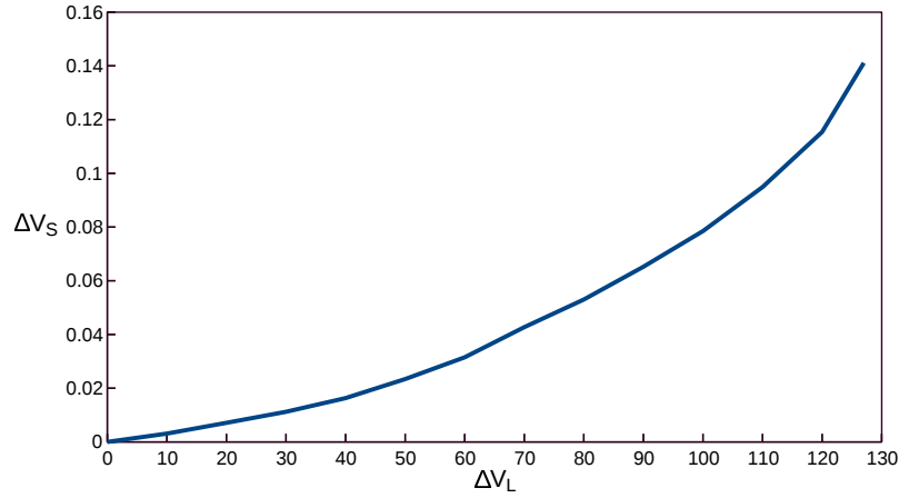
Fig. 4.39 Variation in the shear phase velocities difference with the incorporated difference in longitudinal velocities.
