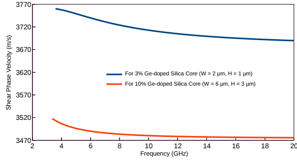
Fig. 5.2 Variations of the phase velocities with the acoustic frequencies for different doping concentration of shear mode U_{11}^X .
