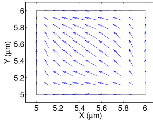
Fig. 3.8 Displacement vectors of U_T mode at k = 400 \text{ m}^{-1} .
