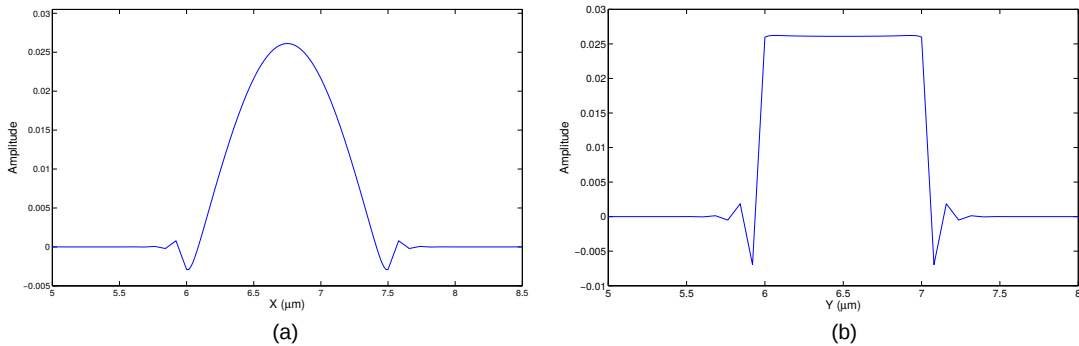
Fig. 6.7 Variations of the of U_X component of the fundamental quasi-shear acoustic U_{11}^X mode along (a) the x -axis and (b) the y -axis at 21 GHz.
