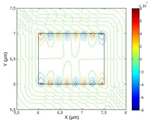
Fig. 6.11 Vector displacement profile of U_Y component of the fundamental quasi-shear acoustic mode U_{11}^X at 21 GHz.
