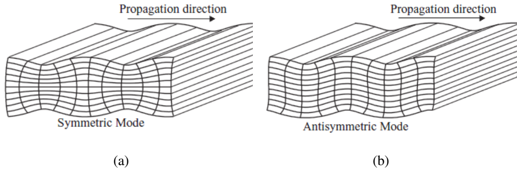
Fig. 2.9 (a) Symmetric and (b) Antisymmetric modes of guided wave motion in plates [Fong, Thesis, 2005].
