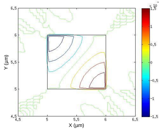
Fig. 3.9 Displacement vector profile of the non-dominant U_Z component of fundamental U_{11}^X acoustic mode at k = 400 \text{ m}^{-1} .
