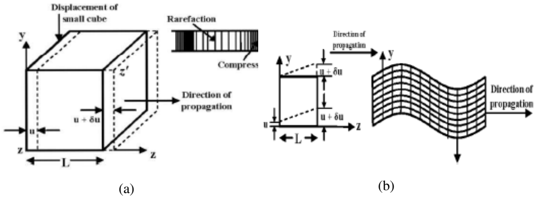
Fig. 2.1 (a) Longitudinal and (b) shear waves propagation [Sriratanavaree, Thesis, 2014].
