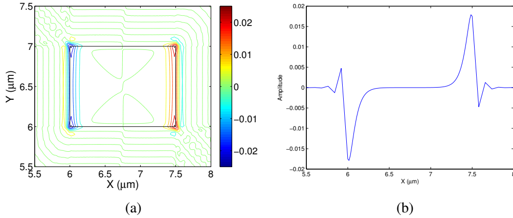
Fig. 6.41 (a) Vector displacement profile and (b) amplitude variations along the x -axis of U_x component of the highly hybrid acoustic mode U_{11}^{HZ} at 20.13 GHz.
