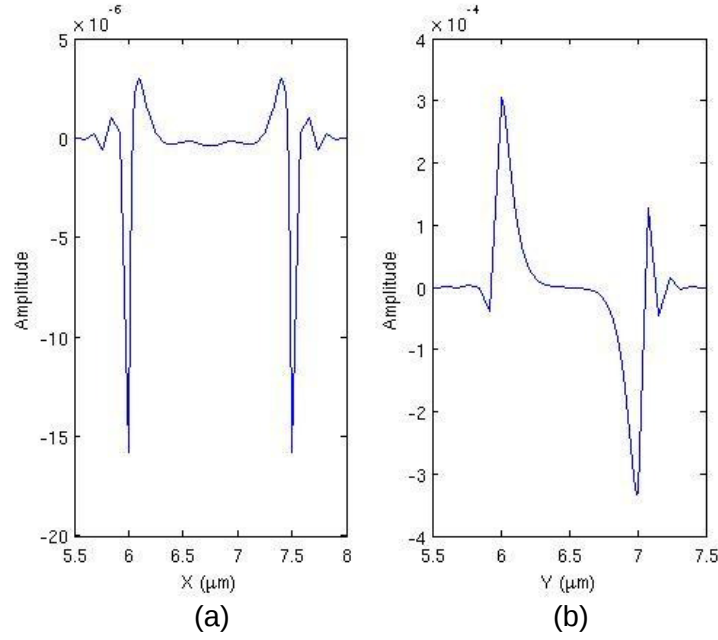
Fig. 6.12 Variations of amplitude (a) along x -axis and (b) along y -axis of U_Y component of the fundamental quasi-shear acoustic mode U_{11}^X at 21 \text{GHz} .
