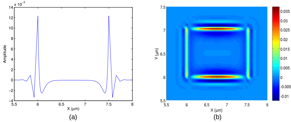
Fig. 6.47 (a) Variations of amplitude along x -axis and (b) vector displacement coloured profile of U_Z component of the highly hybrid acoustic mode U_{11}^{HZ} at 20.13\text{ GHz} .
