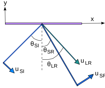
Fig. 2.6 Reflected longitudinal and shear waves from incident of a shear wave on a free surface [Sriratanavaree, Thesis, 2014].
