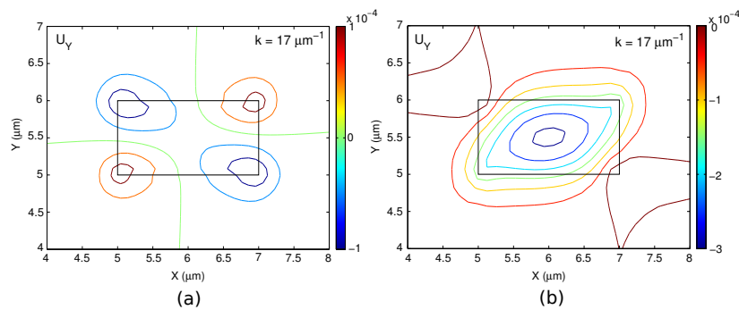
Fig. 4.17 U_Y displacement vectors of the U_{11}^X mode, when (a) 500 \times 500 and (b) 80 \times 80 mesh divisions.
