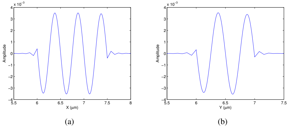
Fig. 6.49 Amplitude variations along the (a) x -axis of U_X component and (b) y -axis of U_Y component of the CHHM mode at 9.81 GHz.
