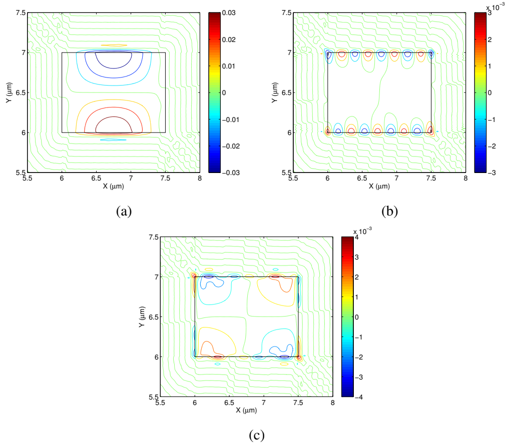
Fig. 6.22 Vector displacement profiles of (a) U_X , (b) U_Y and (c) U_Z components of the U_{12}^X mode at 21.0766 GHz.
