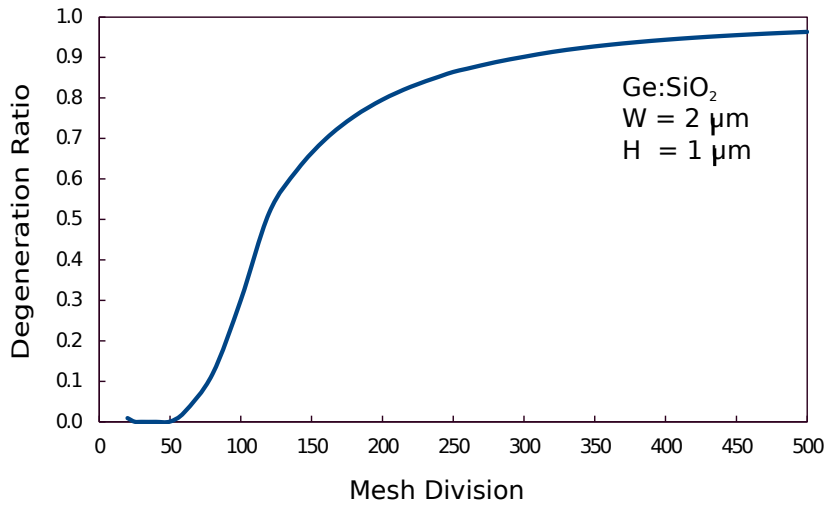
Fig. 4.18 Degeneration ratio against the mesh division for U_y displacement vectors of the U_{11}^x mode at k = 17 \mu m^{-1} .
