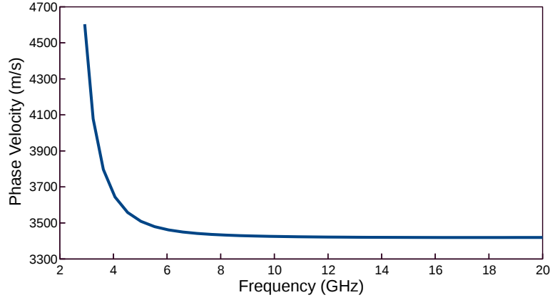
Fig. 6.34 Variations of phase velocity with acoustic frequencies for the highly hybrid acoustic mode U_{11}^{HZ} .
