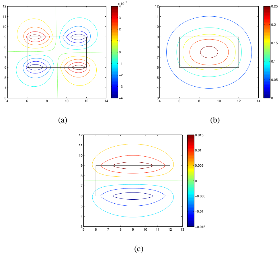
Fig. 5.15 H_x , H_y and H_z field profiles of the fundamental quasi-TE optical mode.
