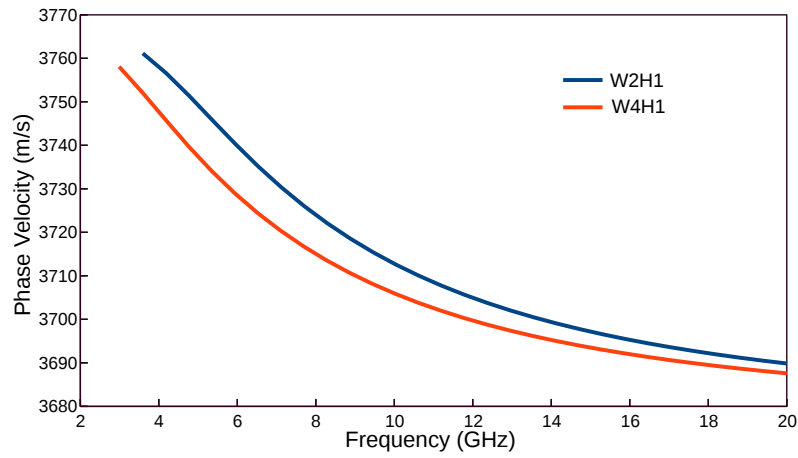
Fig. 4.27 Variation of the phase velocity of U_{11}^X mode for different width.
