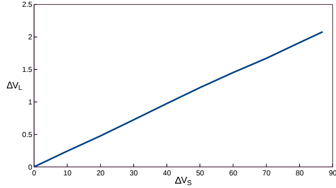
Fig. 4.41 Variation in the longitudinal phase velocities difference with the incorporated difference in shear velocities.
