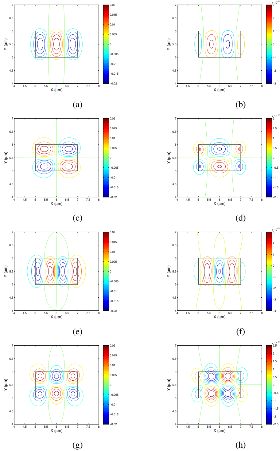
Fig. 4.13 U_X and U_Z displacement vectors of the U_{31}^X (a, b), U_{22}^X (c, d), U_{41}^X (e, f) and U_{32}^X (g, h) modes.
