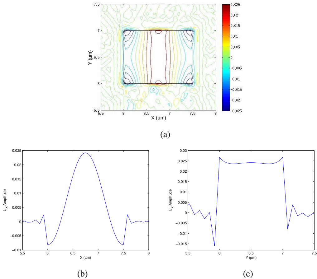
Fig. 6.10 (a) Vector displacement profile, variations of amplitude (b) along x -axis and (c) along y -axis of U_X component of the fundamental quasi-shear acoustic mode U_{11}^X at 4 GHz.
