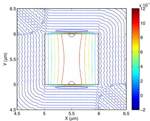
Fig. 3.6 Displacement vector profile of the dominant U_X component of fundamental U_{11}^X acoustic mode at k = 400 \text{ m}^{-1} .
