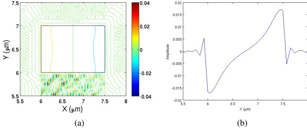
Fig. 6.36 (a) Vector displacement profile and (b) amplitude variations along the x -axis of U_X component of the highly hybrid acoustic mode U_{11}^{HZ} at 5.71 \text{ GHz} .
