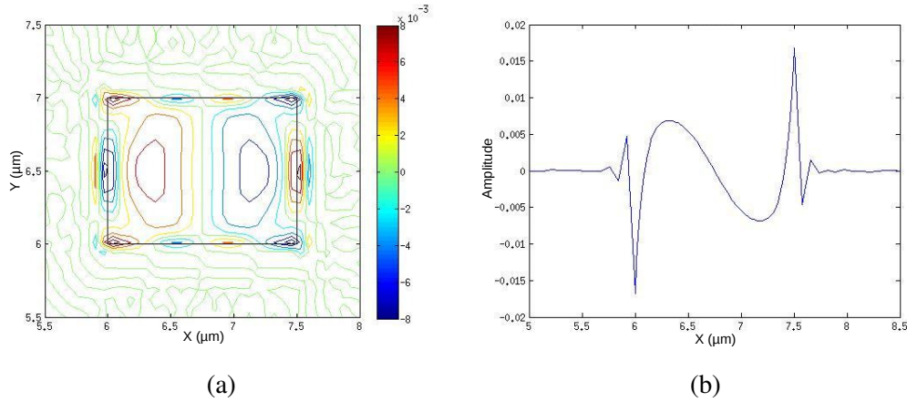
Fig. 6.18 (a) Vector displacement profile and (b) variations of amplitude along x -axis of U_Z component of the U_{11}^X mode at 4 GHz.
