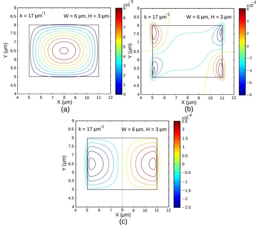
Fig. 5.1 Displacement vector profiles (a) U_X , (b) U_Y and (c) U_Z of the fundamental shear U_{11}^X acoustic mode.
