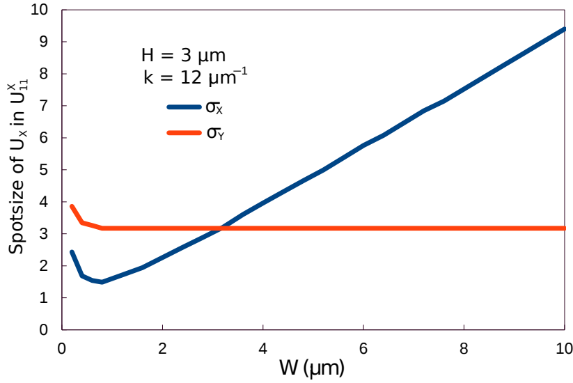
Fig. 5.10 Variations of spot sizes with width for U_{11}^X mode in 10% Ge-doped core.
