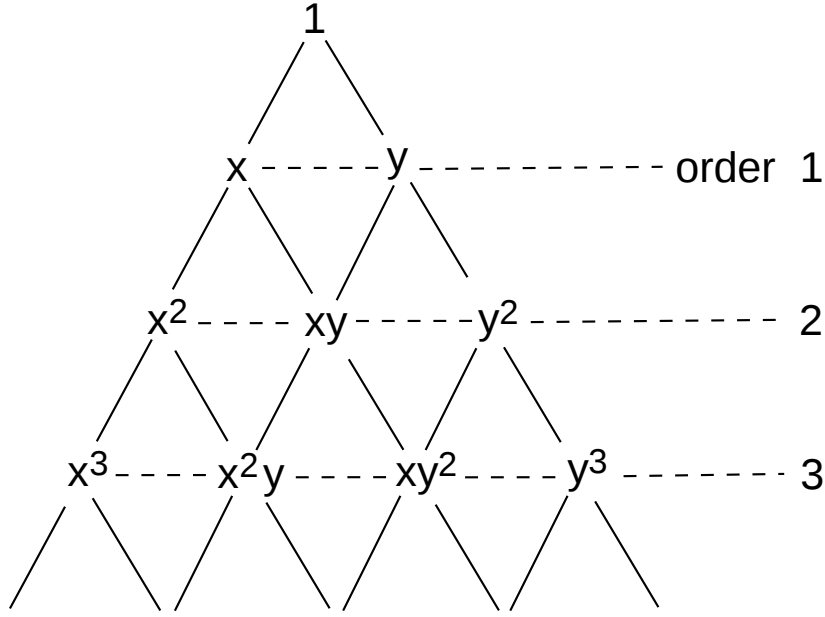
Fig. 3.3 The Pascal triangle [Rahman, Book, 2013].
