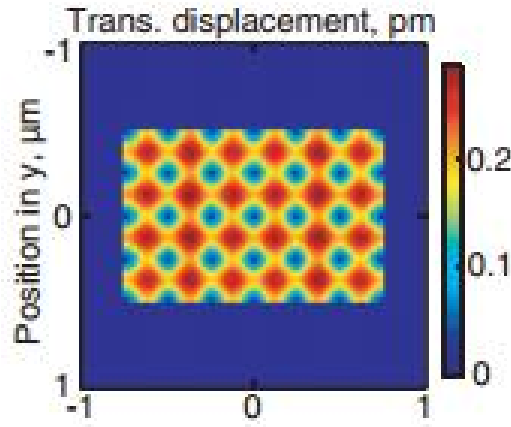
Fig. 6.51 Transverse plane displacement component of the highly hybrid acoustic mode at 9.81 GHz [Laude, 2013].
