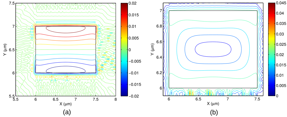
Fig. 6.37 Vector displacement profiles of (a) U_Y component and (b) transverse plane component U_T of the highly hybrid acoustic mode U_{11}^{HZ} at 5.71 \text{ GHz} .
