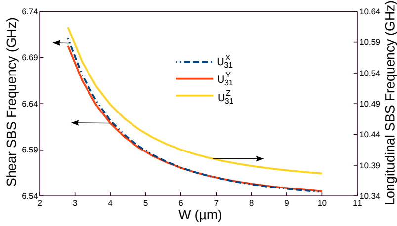
Fig. 5.28 SBS frequency shift for the U_{31}^X , U_{31}^Y and U_{31}^Z modes with varying guide width.
