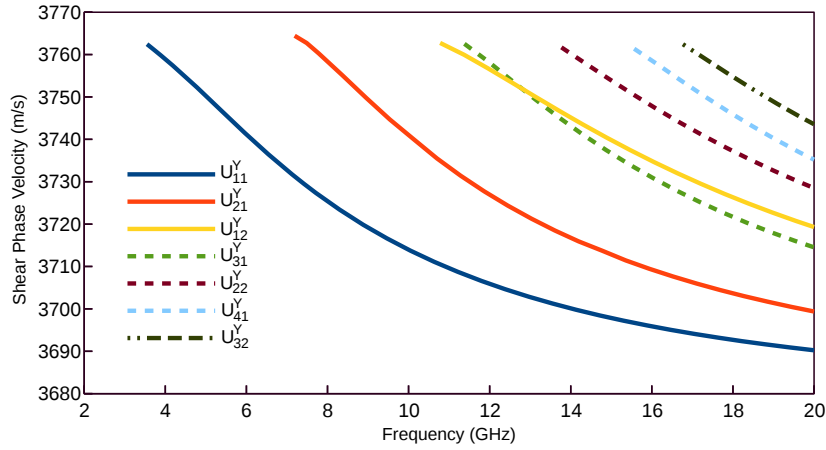
Fig. 4.10 Dispersion curves of acoustic shear U_{mn}^Y modes.
