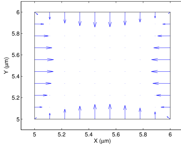
Fig. 3.13 Displacement vectors of U_T mode at k = 200 \text{ m}^{-1} of the surface acoustic mode U_{21}^X .
