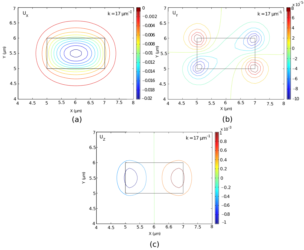
Fig. 4.3 U_x , U_y and U_z displacement vectors of the U_{11}^X mode.
