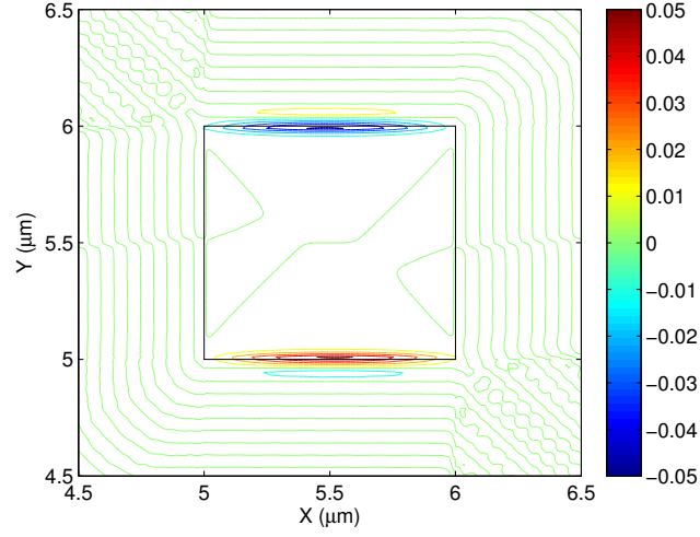
Fig. 3.11 Displacement vector profile of the U_Y component of U_{21}^x acoustic mode at k = 200 \text{ m}^{-1} .
