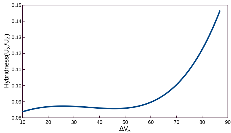
Fig. 4.42 Modal hybridness variation with the incorporated difference in shear velocities.
