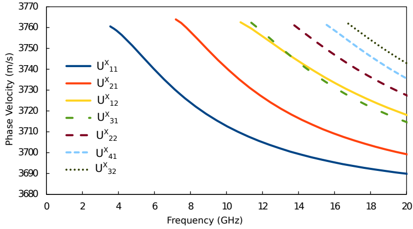
Fig. 4.9 Dispersion curves of acoustic shear U_{mn}^X modes.
