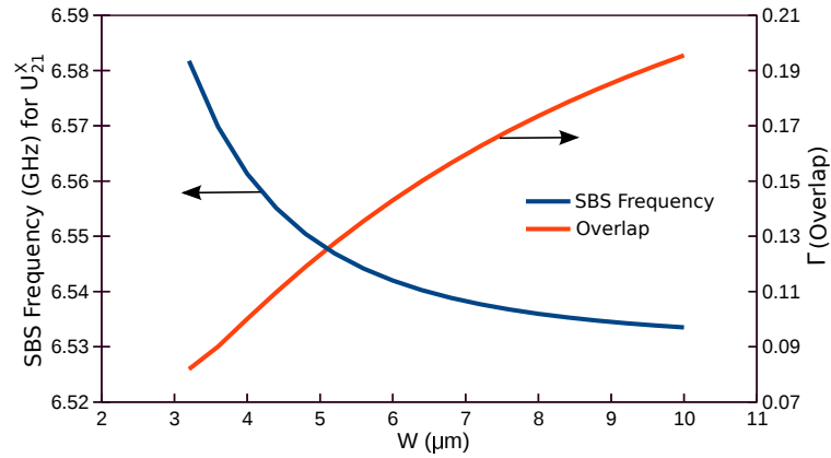
Fig. 5.29 SBS frequency and overlap for the U_Z component of the U_{21}^X mode with varying guide width.
