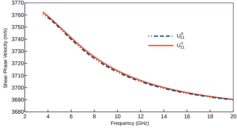
Fig. 4.8 Dispersion curves of acoustic shear U_{11}^X and U_{11}^Y modes.
