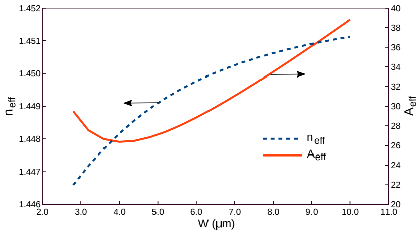
Fig. 5.19 Variations of the n_{eff} and A_{eff} of the H_{11}^Y mode with the guide width, W .
