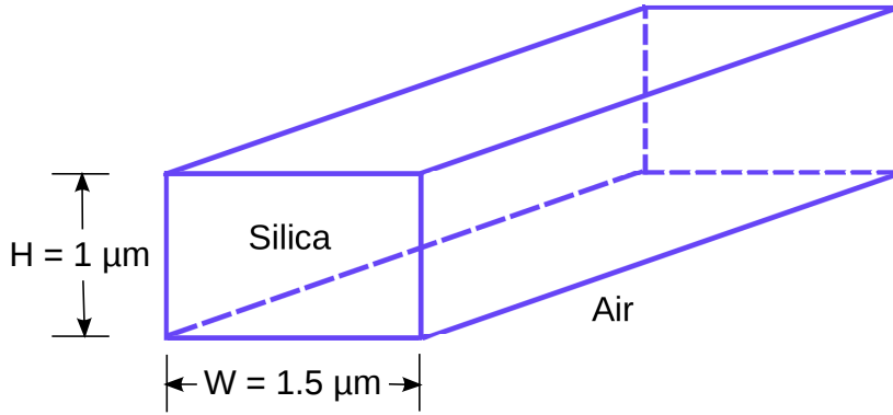
Fig. 6.1 An air cladded silica optical waveguide.
