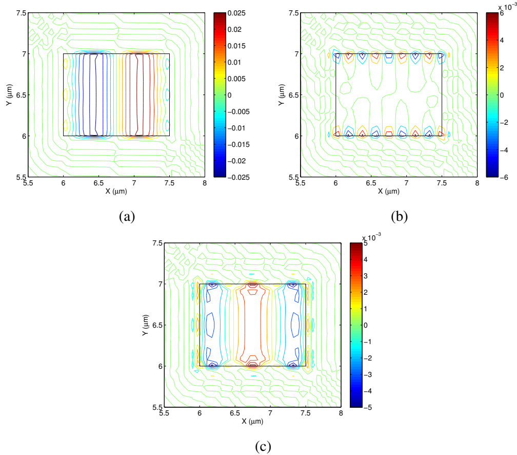
Fig. 6.19 Vector displacement profiles of (a) U_X , (b) U_Y and (c) U_Z components of the U_{21}^X mode at 21.137 GHz.
