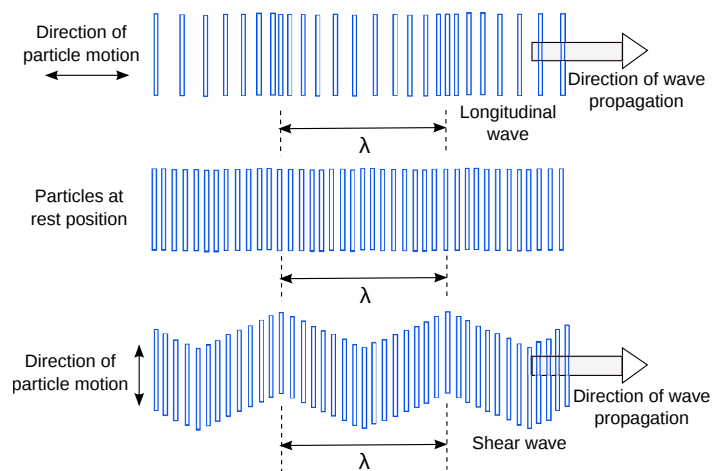
Fig. 2.7 Particles motion and direction of propagation for longitudinal and shear waves [NDT Course Material].
