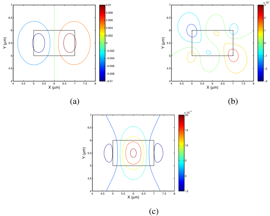
Fig. 4.11 U_X , U_Y and U_Z displacement vectors of the U_{21}^X mode.
