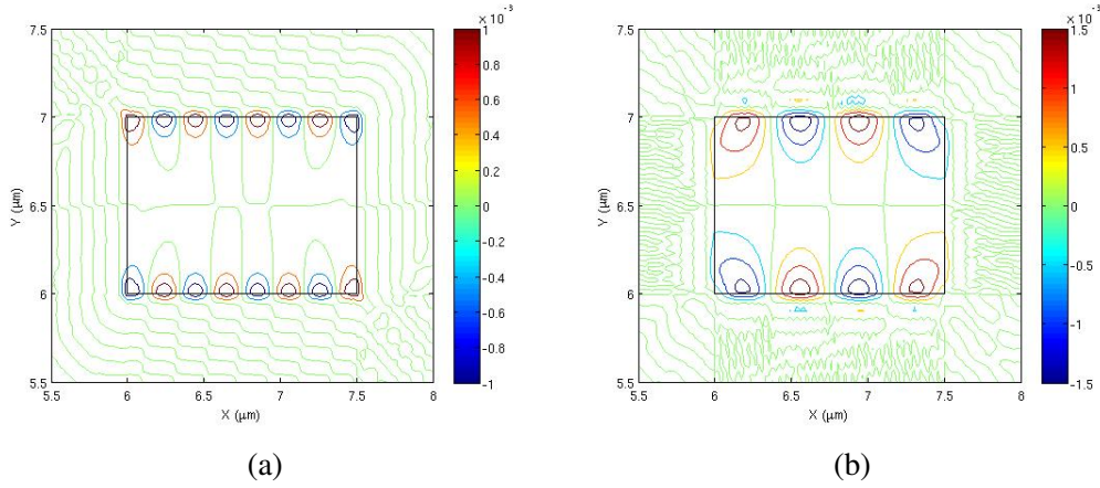
Fig. 6.13 Non-dominant U_Y displacement profiles of the fundamental quasi-shear U_{11}^X acoustic mode (a) at 20 \text{GHz} and (b) 10 \text{GHz} .
