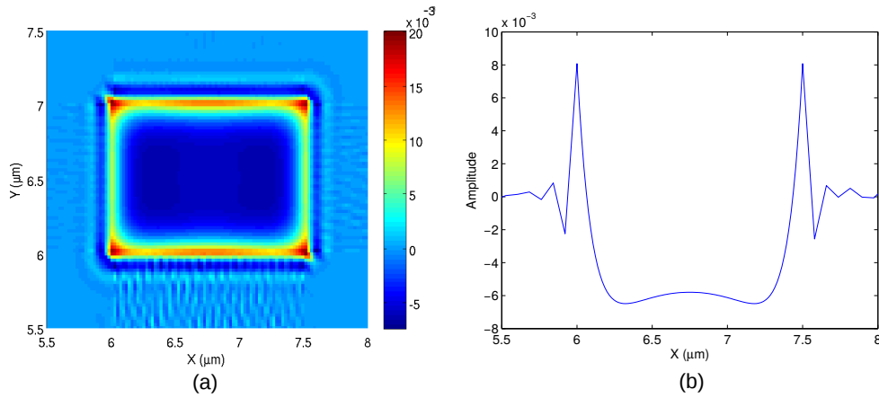
Fig. 6.44 (a) Vector displacement coloured profile and (b) variations of amplitude along x -axis of U_Z component of the highly hybrid acoustic mode U_{11}^{HZ} at 5.71 GHz.
