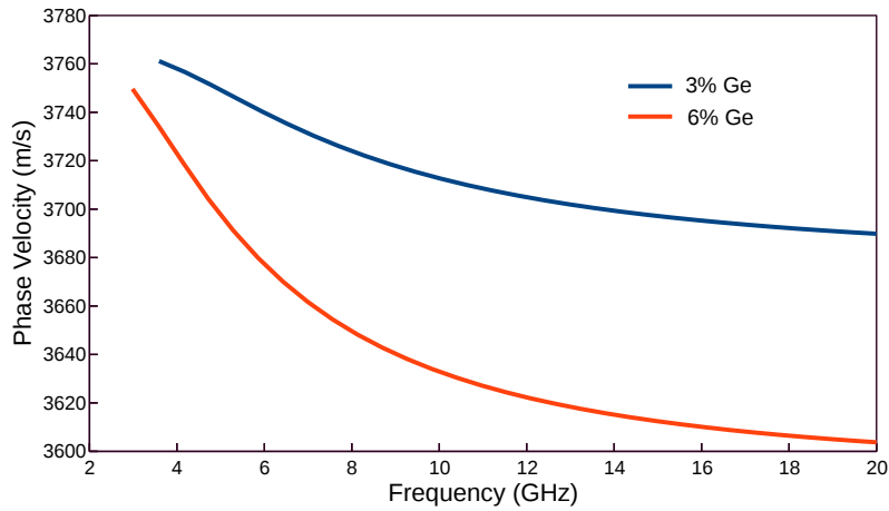
Fig. 4.28 Variation of the phase velocity of U_{11}^X mode for different doping concentration.
