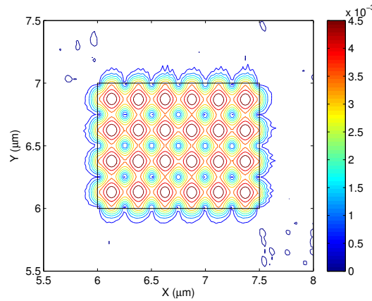
Fig. 6.50 Transverse plane component U_T of the complex highly hybrid acoustic mode (CHHM) at 9.81 GHz.
