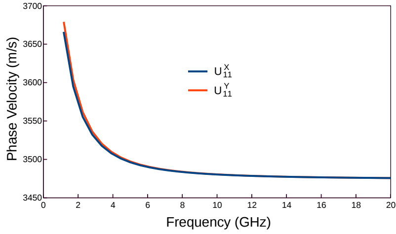
Fig. 5.4 Dispersion curves of acoustic shear U_{11}^X and U_{11}^Y modes in 10% Ge-doped core.
