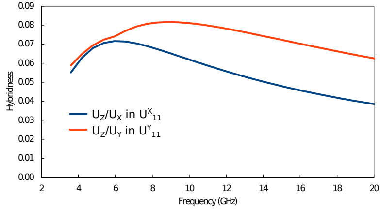
Fig. 4.22 Variation of modal hybridness of two fundamental shear modes with the frequency.
