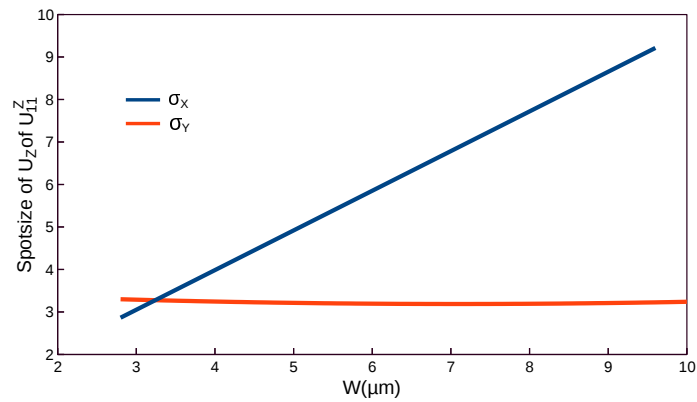
Fig. 5.14 Variations of spotsizes with width for U_{11}^Z mode in 10% Ge-doped core.
