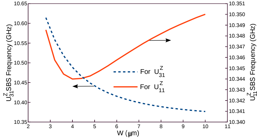
Fig. 5.22 SBS frequency shifts for the U_{11}^Z and U_{31}^Z modes with waveguide width.
