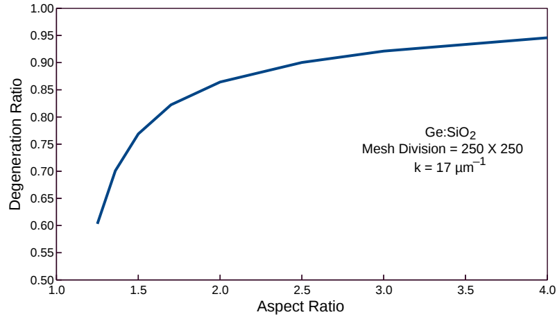
Fig. 4.19 Degeneration ratio against the aspect ratio of guide for U_y displacement vectors of the U_{11}^x mode.
