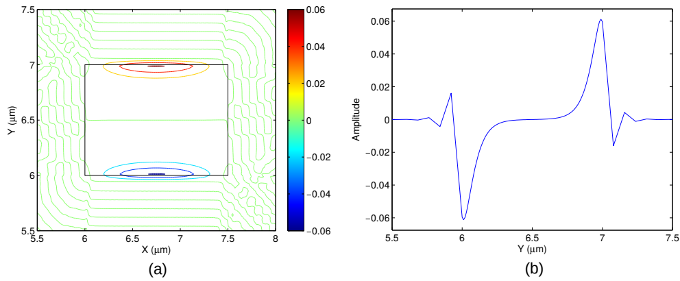
Fig. 6.39 (a) Vector displacement profile and (b) amplitude variations along the y -axis of U_Y component of the highly hybrid acoustic mode, U_{11}^{HZ} at 20.13 \text{ GHz} .
