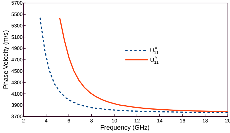
Fig. 6.24 Variations of the velocities with the acoustic frequencies for the two near degenerate fundamental acoustic quasi-shear U_{11}^X and U_{11}^Y modes.
