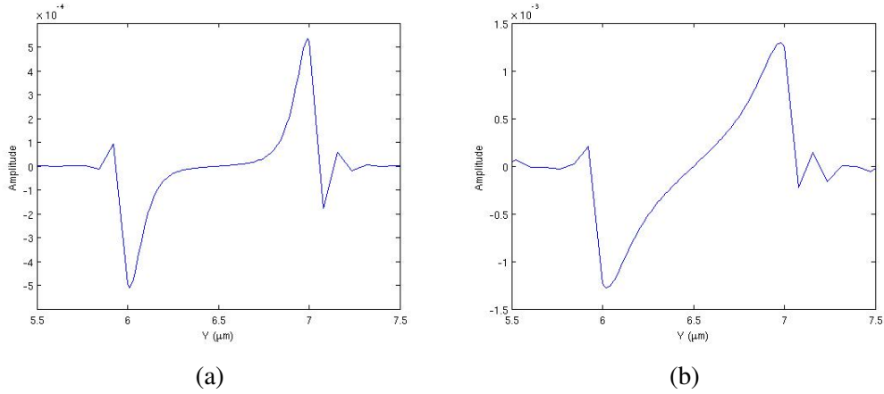
Fig. 6.14 Variations of amplitude along y-axis of U_Y component of the fundamental quasi-shear acoustic mode U_{11}^X at (a) 20 GHz and (b) 10 GHz.
