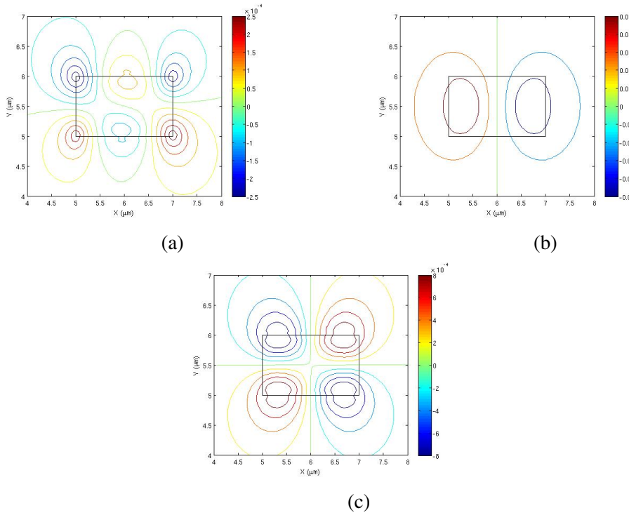
Fig. 4.14 U_X , U_Y and U_Z displacement vectors of the U_{21}^Y mode.
