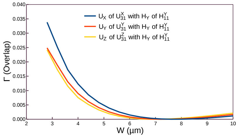
Fig. 5.27 Variations of overlaps of H_{11}^Y with the U_{31}^X , U_{31}^Y and U_{31}^Z modes with varying guide width.
