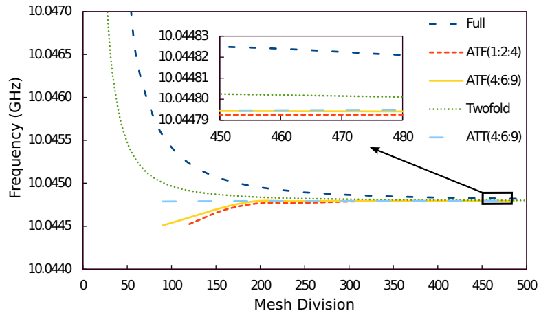
Fig. 4.21 Variation of eigen frequency with the mesh division for the U_{11}^x mode at k = 17 \mu m^{-1} for both full and quarter structures.
