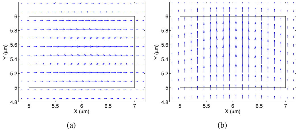
Fig. 4.7 Total displacement vectors, U_T , in the transverse plane at k = 17 \mu m^{-1} for (a) U_{11}^X and (b) U_{11}^Y modes.
