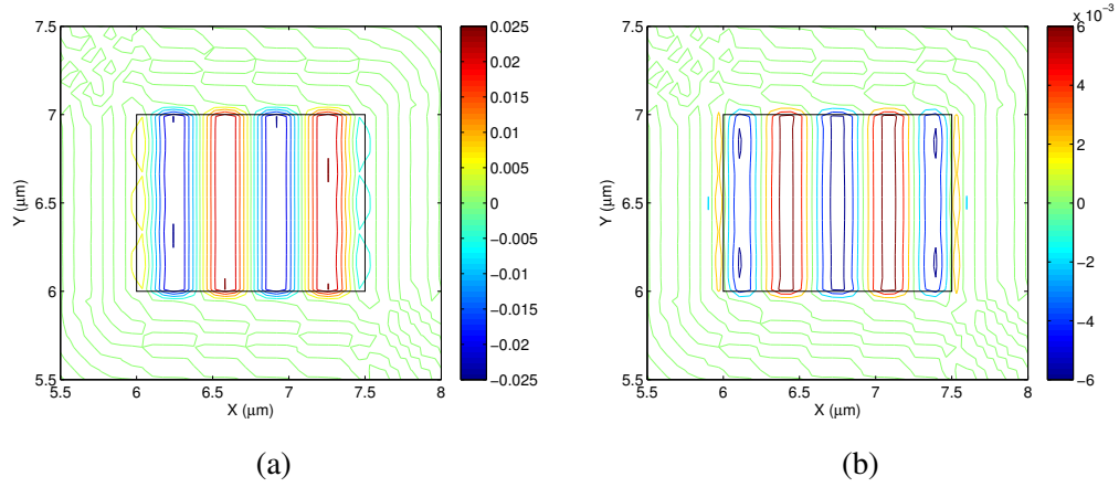
Fig. 6.21 Vector displacement profiles of (a) U_X and (b) U_Z components of the U_{41}^X mode at 21.69 GHz.
