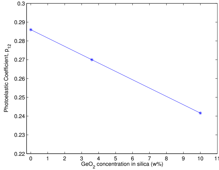
Fig. 5.31 Photoelastic constant, p_{12} , as a function of GeO_2 concentration in silica.
