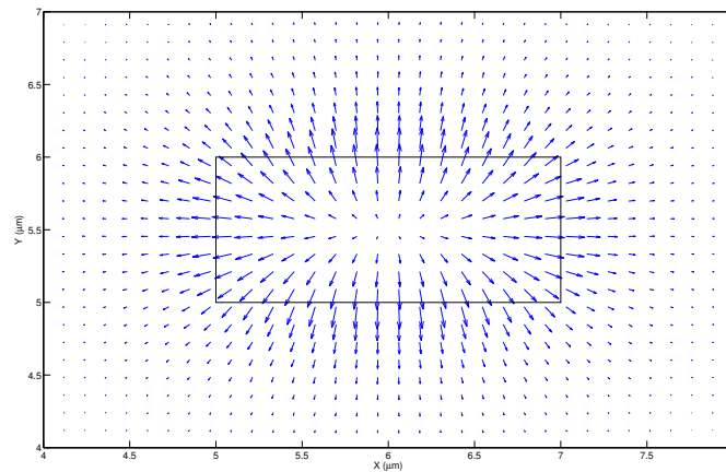
Fig. 4.30 Transverse plane displacement vector, U_T , at k = 17 \mu\text{m}^{-1} for U_{11}^Z mode.
