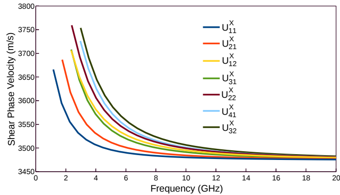
Fig. 5.3 Variations of the phase velocities with the acoustic frequencies for the shear modes.
