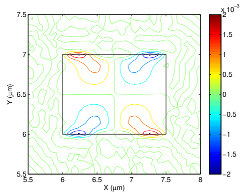
Fig. 6.28 Vector displacement profile of U_X component of the U_{11}^Y mode at 8.38 GHz.
