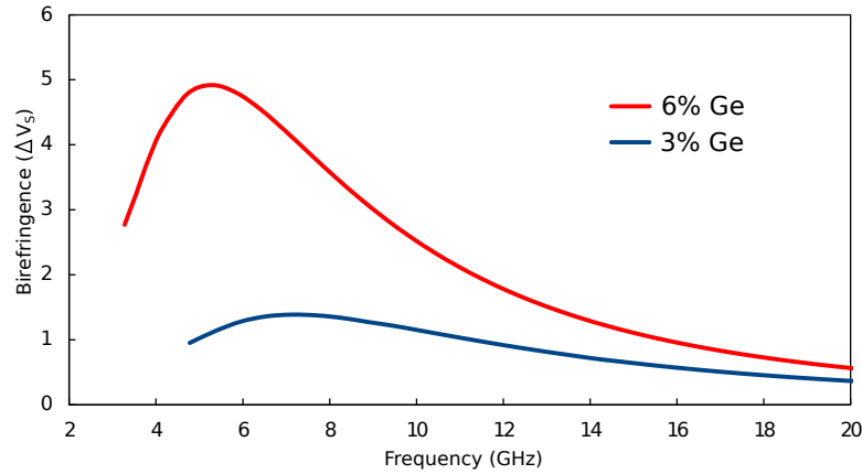
Fig. 4.26 Variation of modal birefringence with frequency for different Ge doped waveguides.
