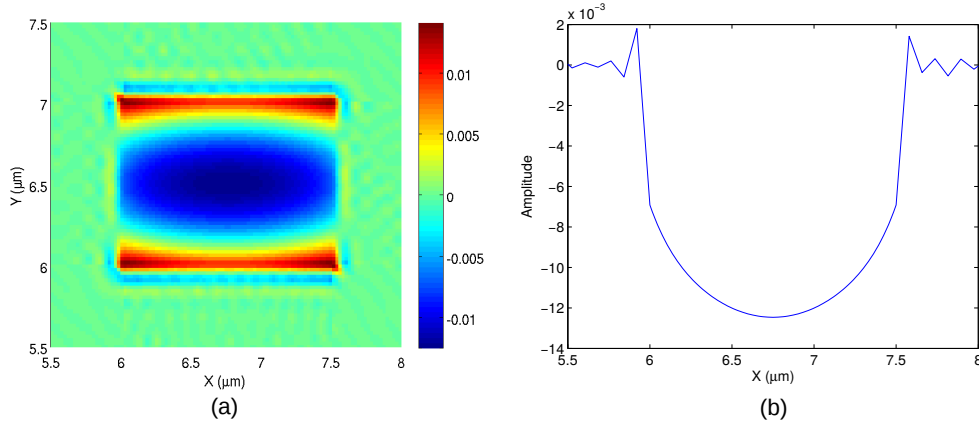
Fig. 6.42 (a) Vector displacement coloured profile and (b) variations of amplitude along x -axis of U_Z component of the highly hybrid acoustic mode U_{11}^{HZ} at 3.24 GHz.
