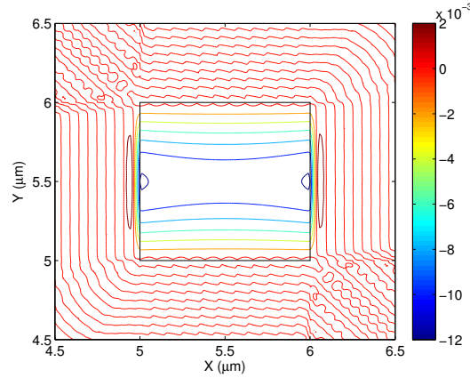
Fig. 3.7 Displacement vector profile of the non-dominant U_Y component of fundamental U_{11}^X acoustic mode at k = 400 \text{ m}^{-1} .
