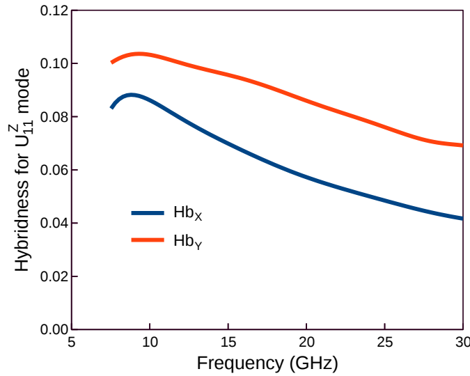
Fig. 4.34 Variation of modal hybridness of the fundamental longitudinal mode with the frequency.
