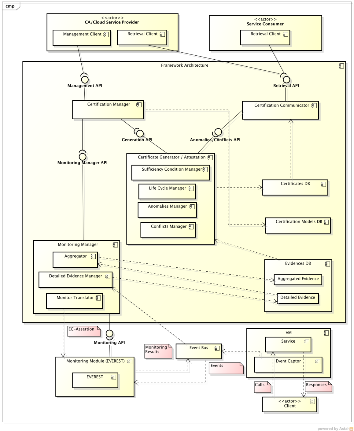
Figure 49 – Monitoring Architecture
