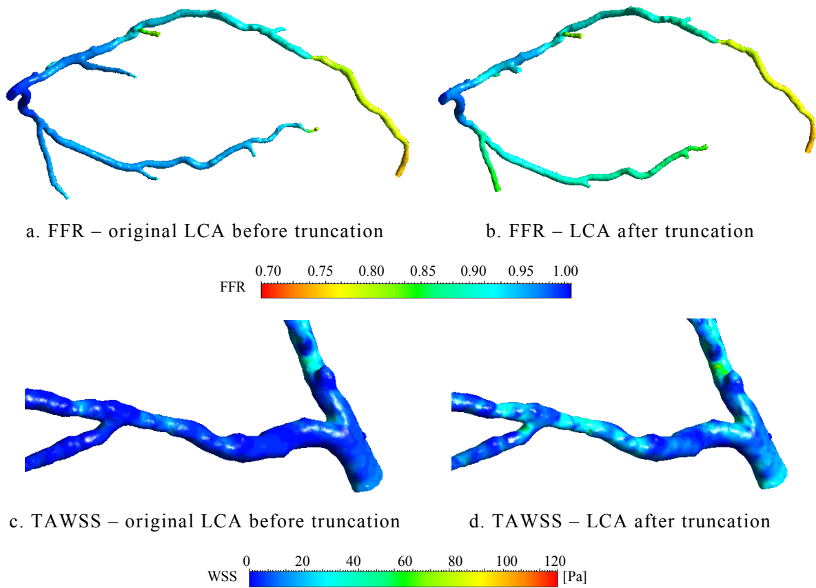
Figure 5.35 Computed 3D FFR and TAWSS before and after truncation of side branches up to \approx 2 mm level ( \text{dR} = 0.2 )
