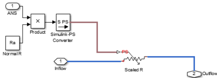
Figure 4.24 0D model of the “R peripheral coronary vasculature” element implemented in MATLAB® Simulink
