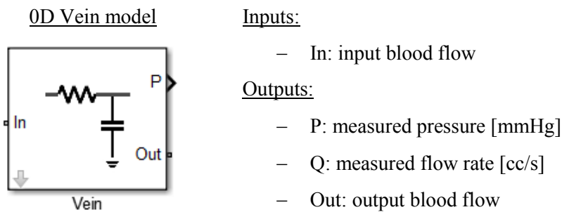
Figure 4.22 0D model of the “Vein” element implemented in MATLAB® Simulink
