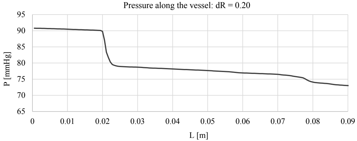
Figure 4.9 Computed pressure along a single 0D vessel branch model
