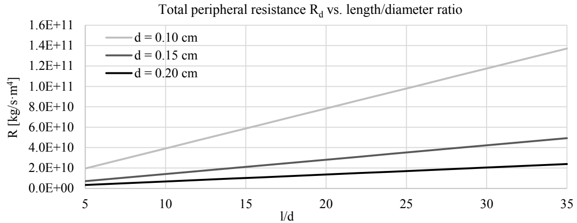
Figure 5.20 Computed downstream resistance for an outlet vs. length/diameter ratio of the 1D peripheral tree for three d_{\text{out}} cases
