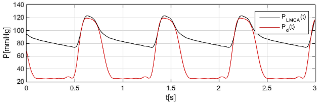
Figure 3.10 BC model pressure waveforms measured in the 0D CVS model
