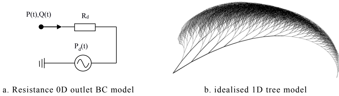
Figure 4.7 0D model of peripheral vasculature for coronary tree outlets
