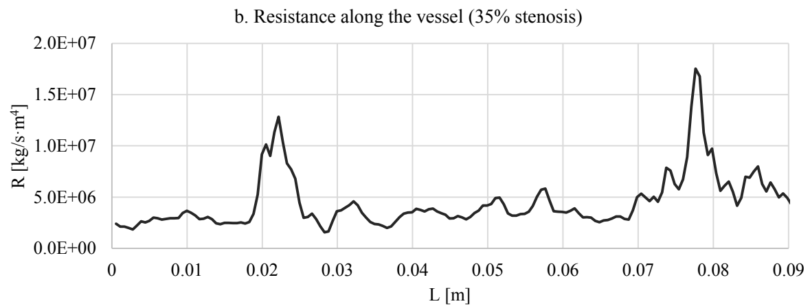
Figure 5.51 Extracted 0D flow resistance along 35% stenosis vessel case
