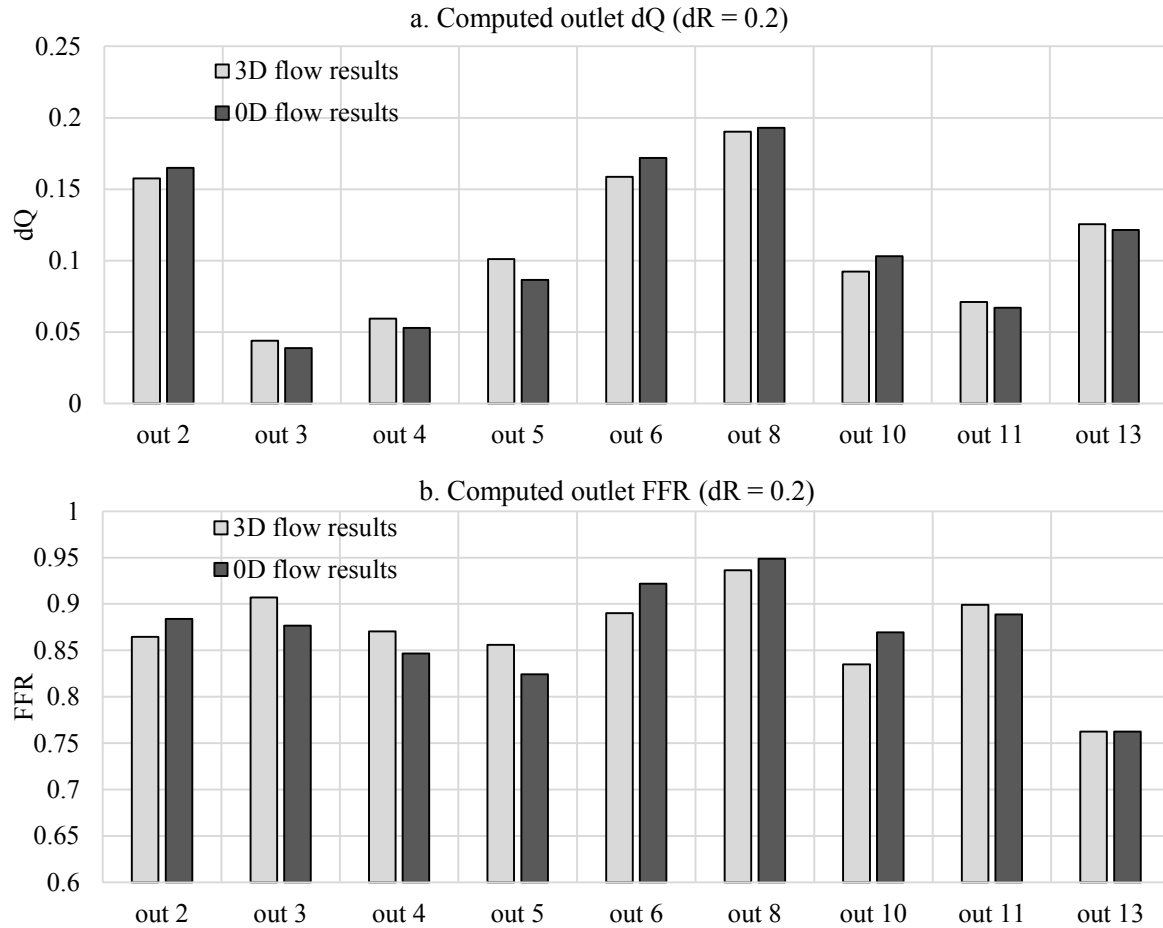
Figure 5.57 0D and 3D computed outlet FFR and dQ for the baseline LCA case (dR = {0.2; 1.0})
