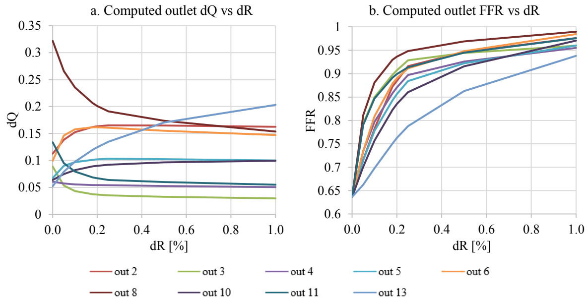
Figure 3.20 An example of changes in the computed FFR and dQ at the outlets in response to modelled peripheral vasodilation (dR = 0.0:1.0)
