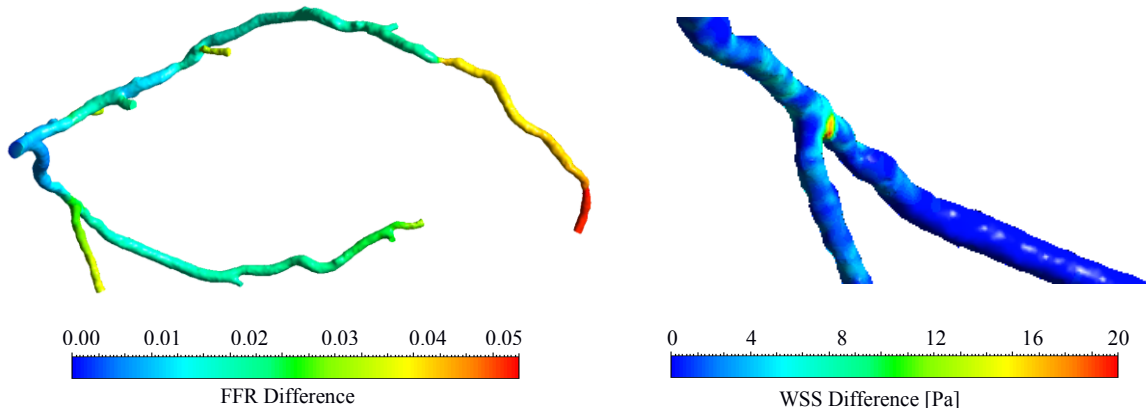
Figure 5.17 Computed difference in FFR and TAWSS before and after adjustment of R_d ( dR = 0.2 )
