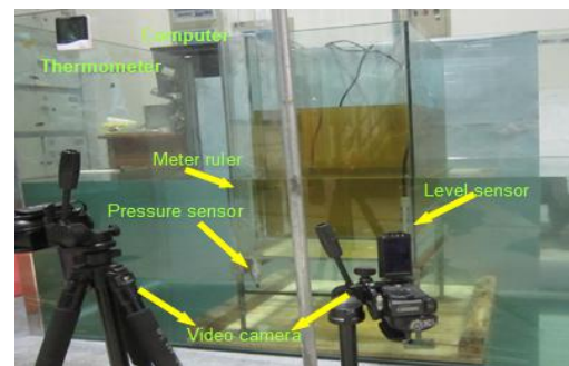
Fig.3 Experimental equipments
