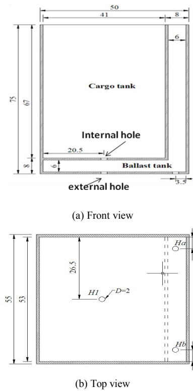
Fig. 1 Dimensions of model tank (a) and location of the hole (b) (unit: cm)
